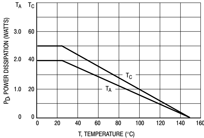
Figure 3. Power Derating
