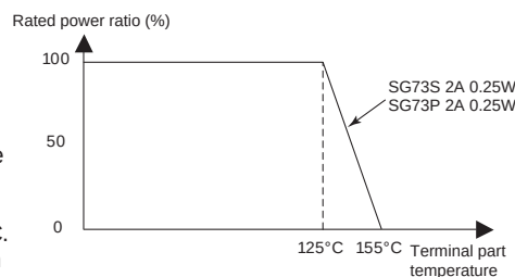
Figure 8. Derating curve of 0.25W rated power based on terminal part temperature
