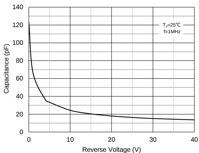
Fig.3 - Typical Capacitance Characteristics (per diode)
