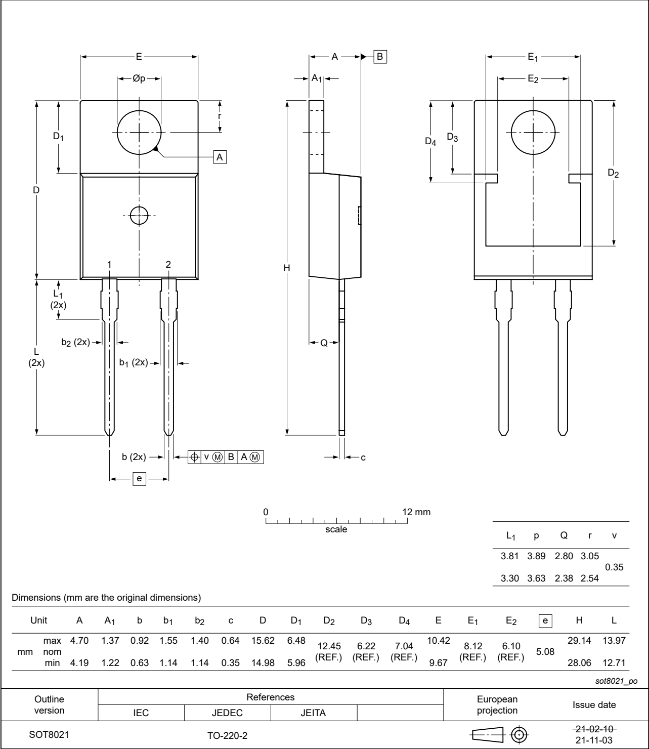
Fig. 11. Package outline TO-220-2 (SOT8021)
