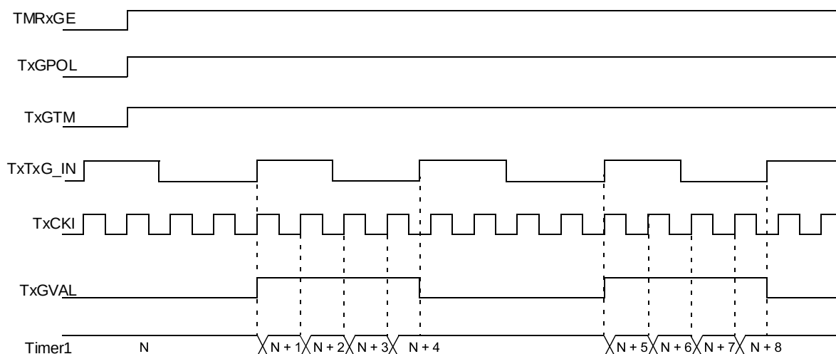
Figure 23-5. Timer1 Gate Toggle Mode
