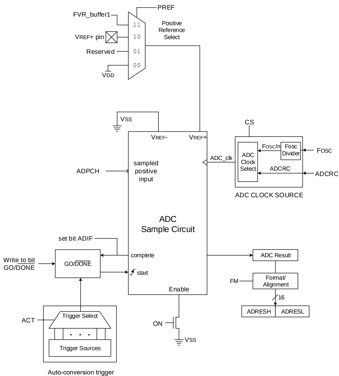
Figure 32-1. ADC Block Diagram
