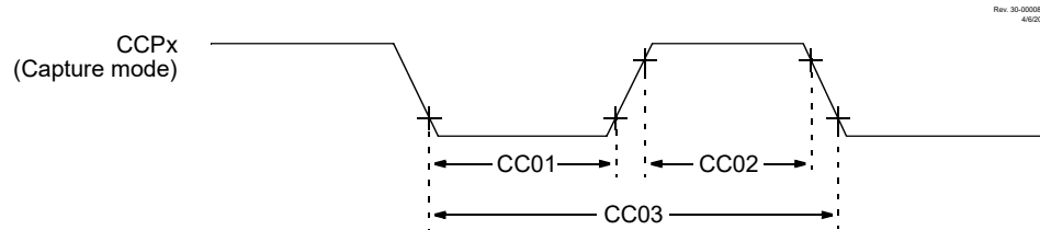
Figure 42-12. Capture/Compare/PWM Timings (CCP)
