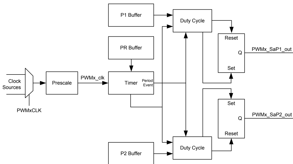
Figure 27-5. Center-Aligned Block Diagram
