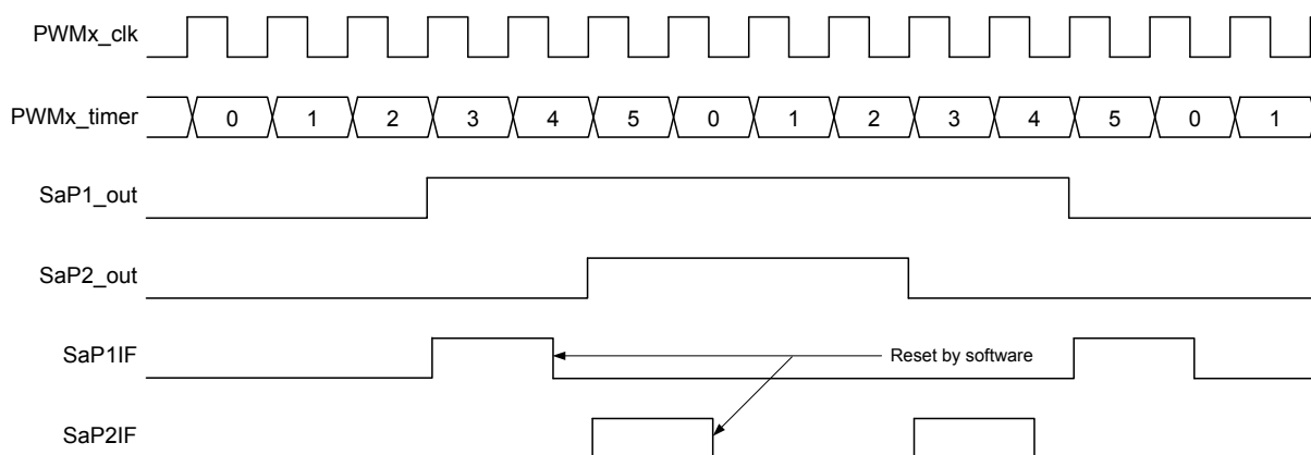
Figure 27-6. Center-Aligned Timing Diagram
