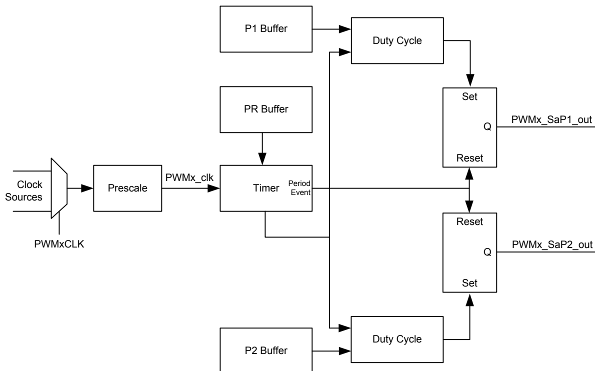
Figure 27-3. Right-Aligned Block Diagram
