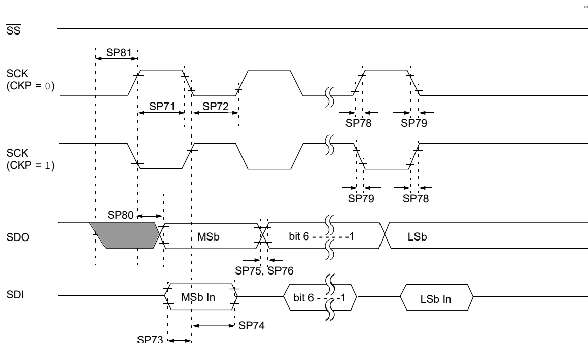
Figure 42-15. SPI Host Mode Timing (CKE = 0, SMP = 0)
