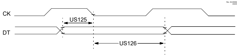
Figure 42-14. EUSART Synchronous Receive (Host/Client) Timing
