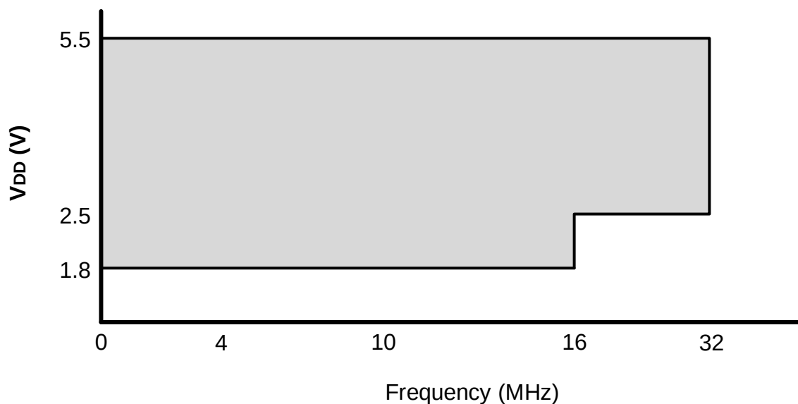
Figure 42-1. Voltage Frequency Graph, -40°C ≤ T_A ≤ +125°C
