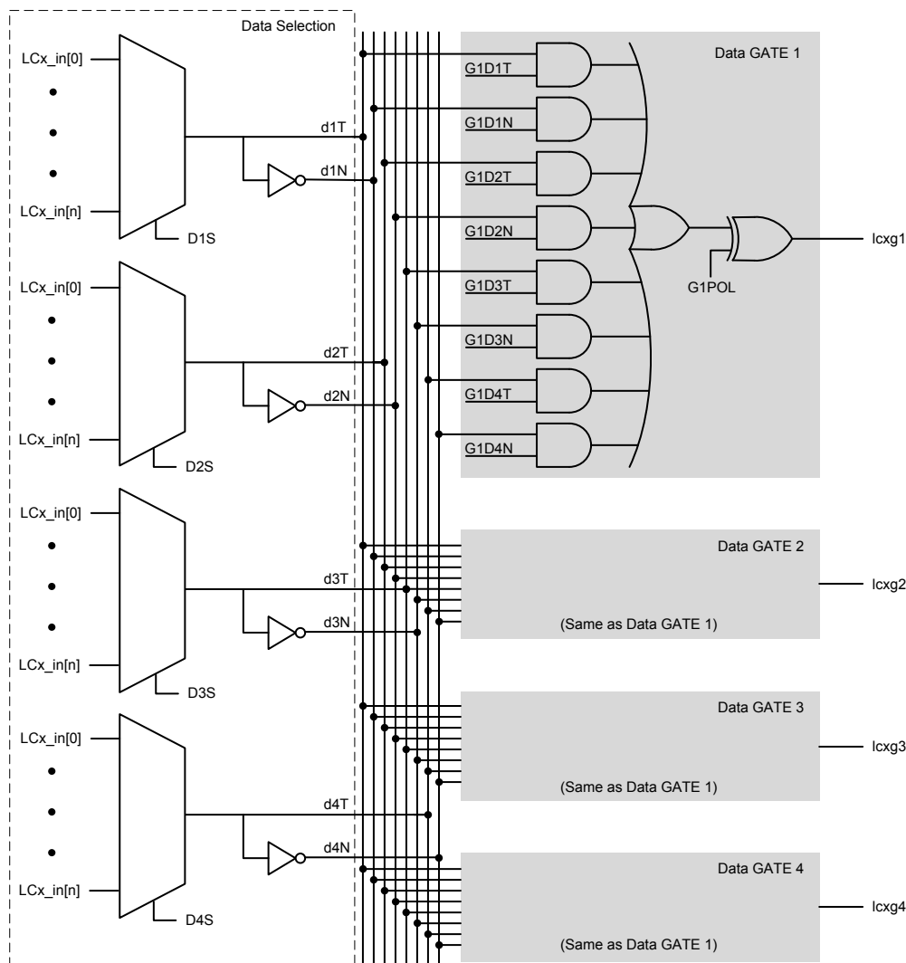
Figure 28-2. Input Data Selection and Gating
