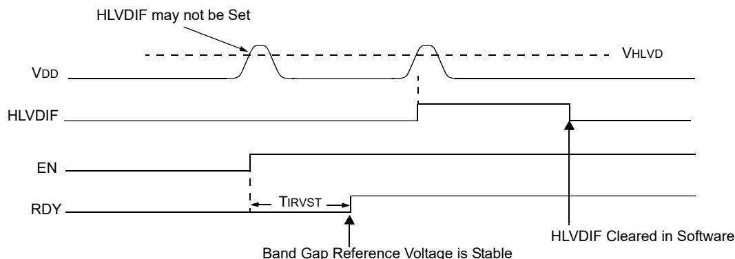
Figure 35-3. High-Voltage Detect Operation (INTH = 1)
