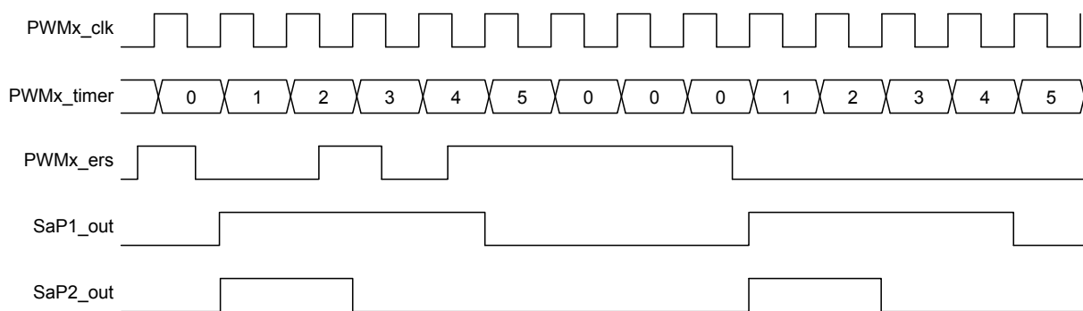
Figure 27-16. Left Aligned Mode with ERSNOW = 0
