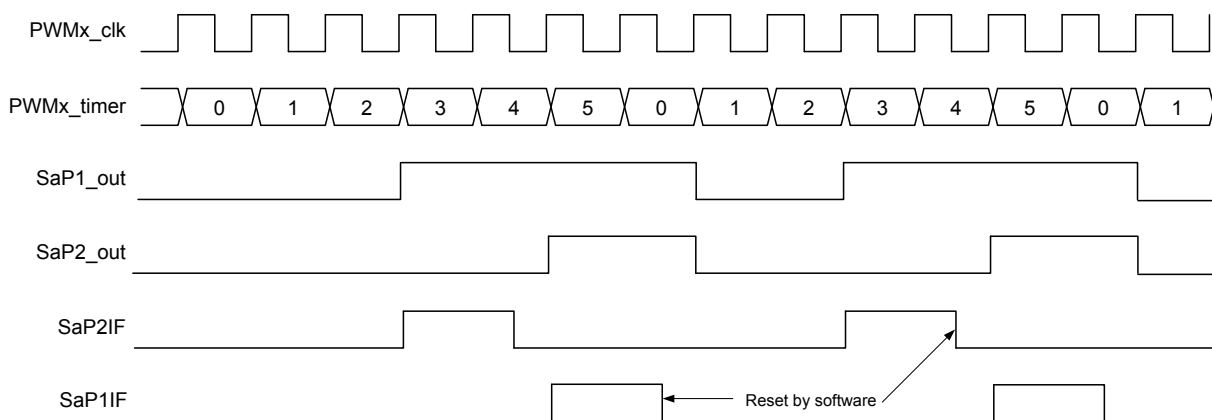
Figure 27-4. Right-Aligned Timing Diagram
