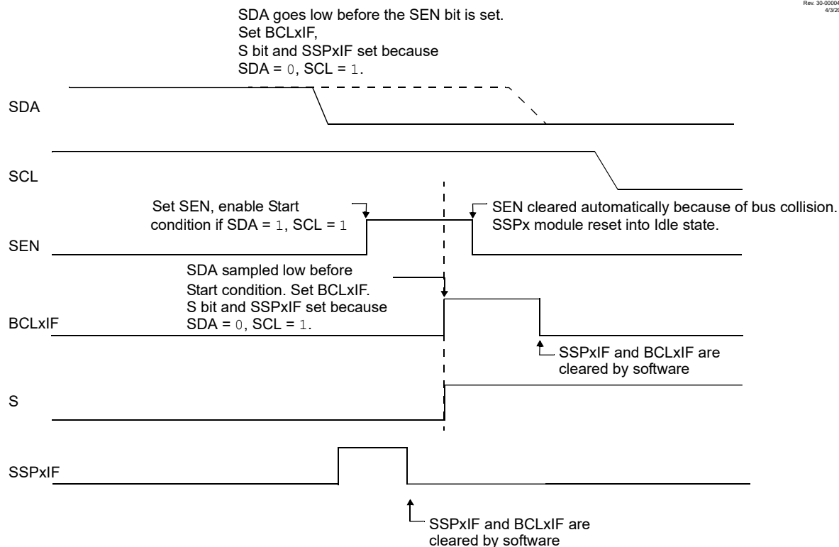
Figure 30-34. Bus Collision During Start Condition (SDA Only)
