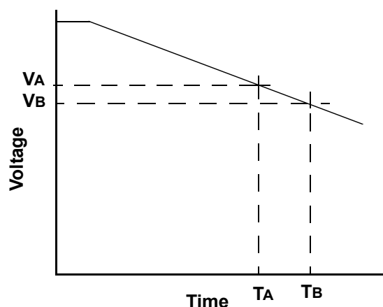
Figure 35-4. Typical Low-Voltage Detect Application
