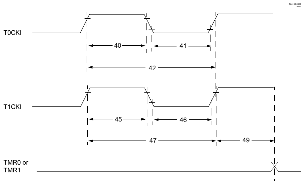
Figure 42-11. Timer0 and Timing1 External Clock Timings
