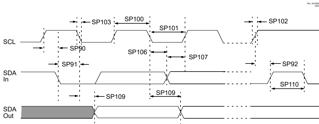
Figure 42-20. I 2 C Bus Data Timing
