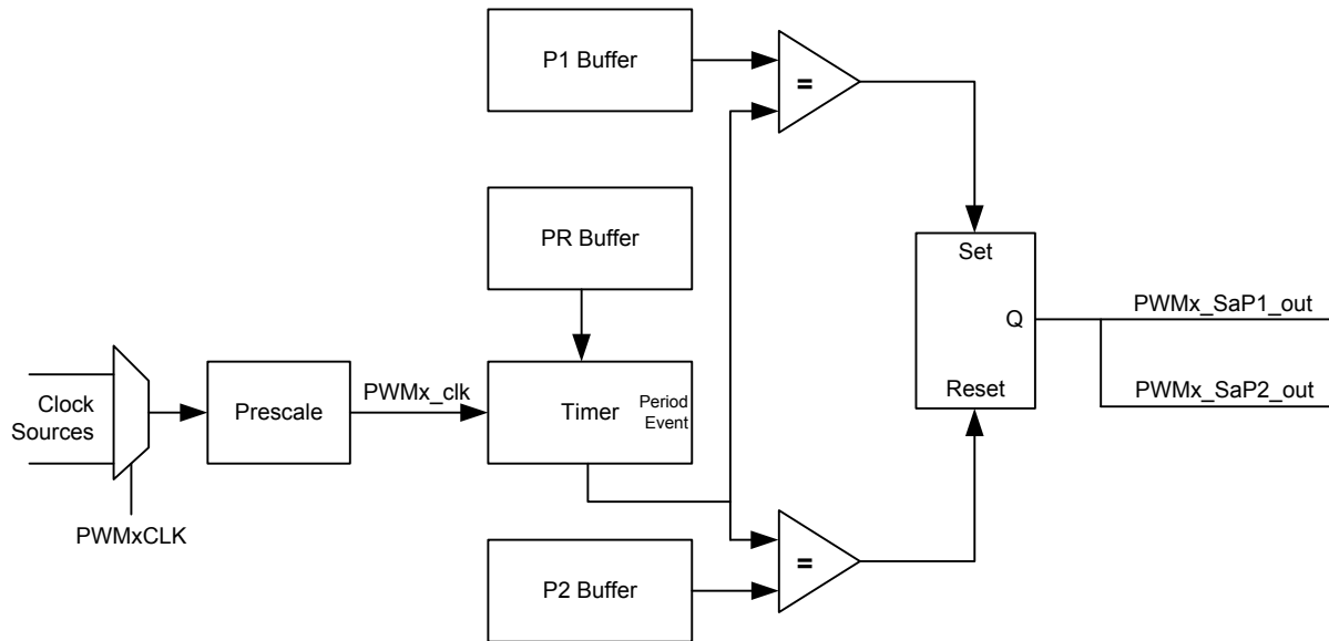
Figure 27-7. Variable Alignment Block Diagram
