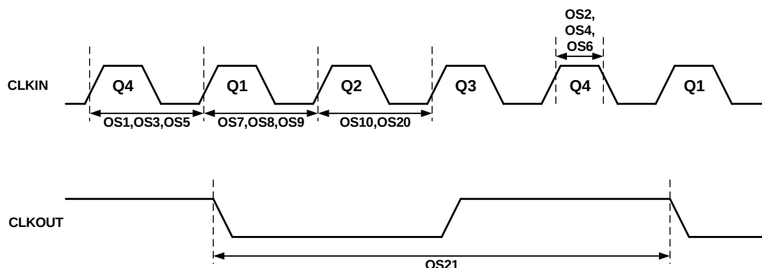
Figure 42-4. Clock Timing
