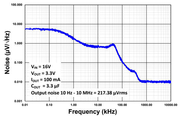
Figure 4-21. Noise vs. Frequency (3.3V)
