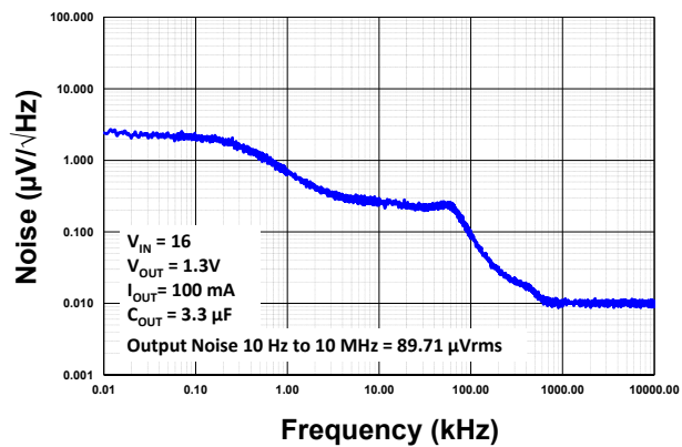
Figure 4-20. Noise vs. Frequency (1.3V – ADJ Output)
