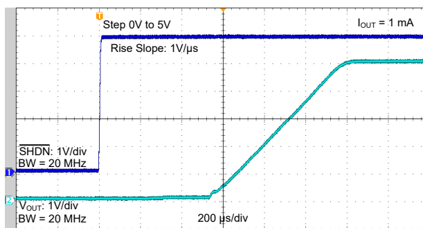
Figure 4-37. Start-up from \overline{\text{SHDN}} (0V to 5V, 5V)
