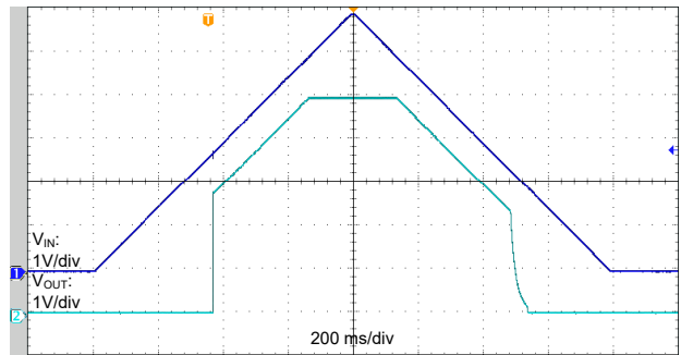
Figure 4-19. UVLO (5V)
