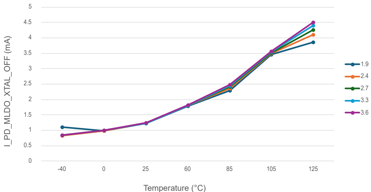
Figure 49-9. Sleep Current with MLDO_XTAL_OFF
