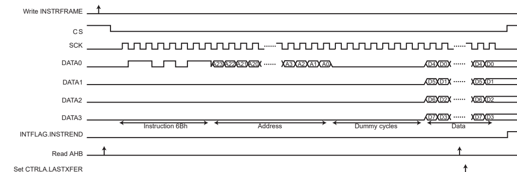
Figure 36-17. Instruction Transmission Waveform 6
