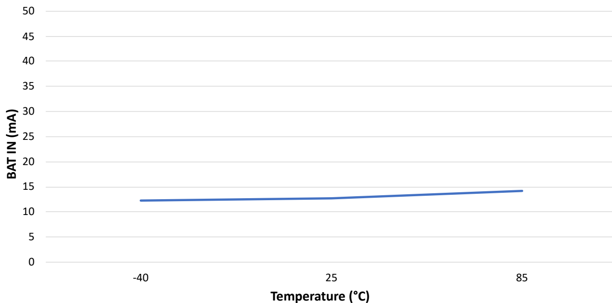
Figure 49-58. Module IEEE® 802.15.4 Receive Current vs. Temperature
