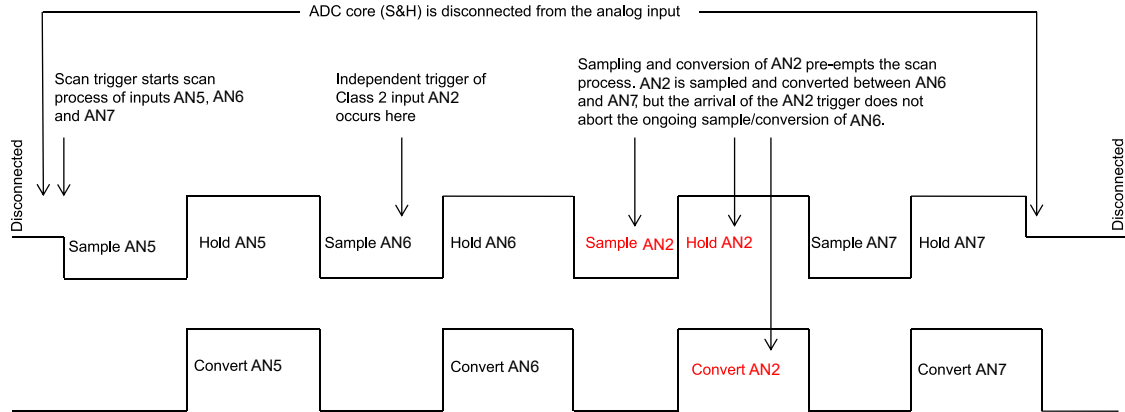
Figure 37-6. Scan Conversion Pre-empted by Class 2 Input Trigger
