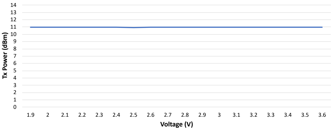
Figure 49-48. IEEE® 802.15.4 Transmit Power vs. VDD Supply Voltage
