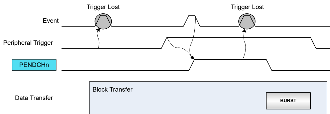
Figure 27-13. Periodic Event with Burst Peripheral Triggers
