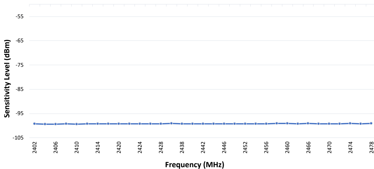
Figure 49-46. Module Bluetooth Low Energy Receive Sensitivity vs. Frequency
