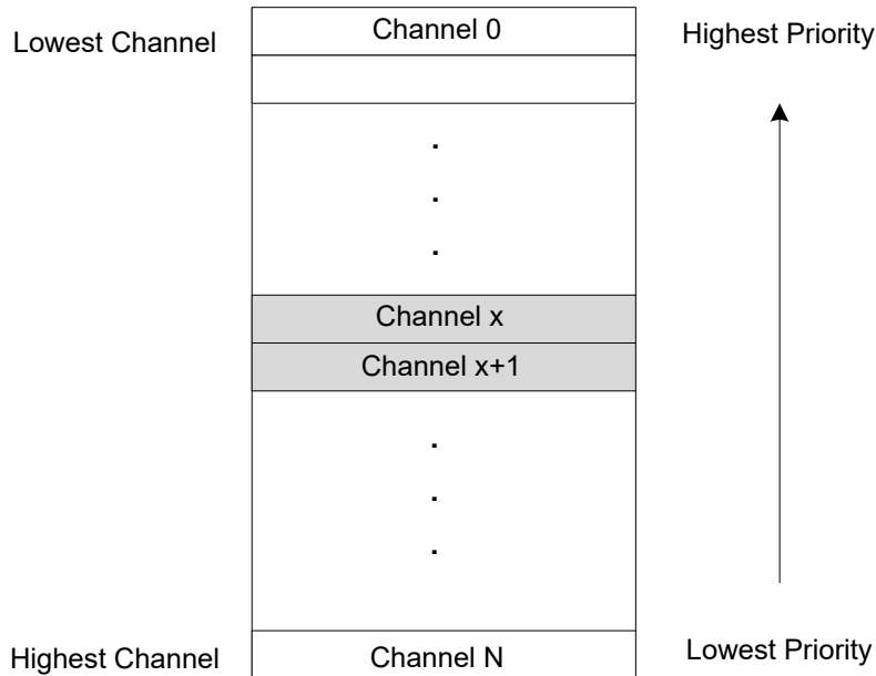
Figure 27-5. Static Priority Scheduling
