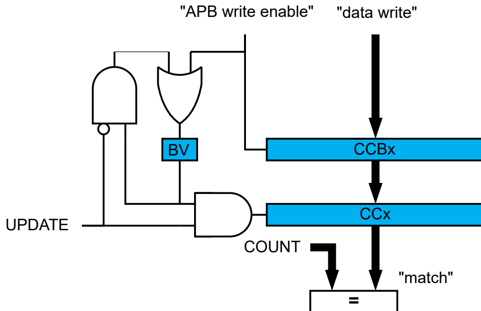
Figure 42-9. Compare Channel Double Buffering
