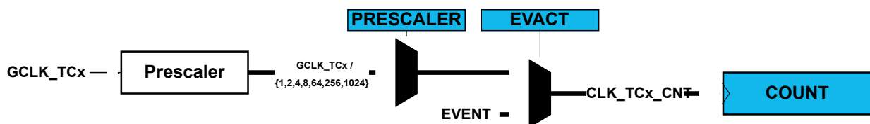
Figure 41-2. Prescaler
