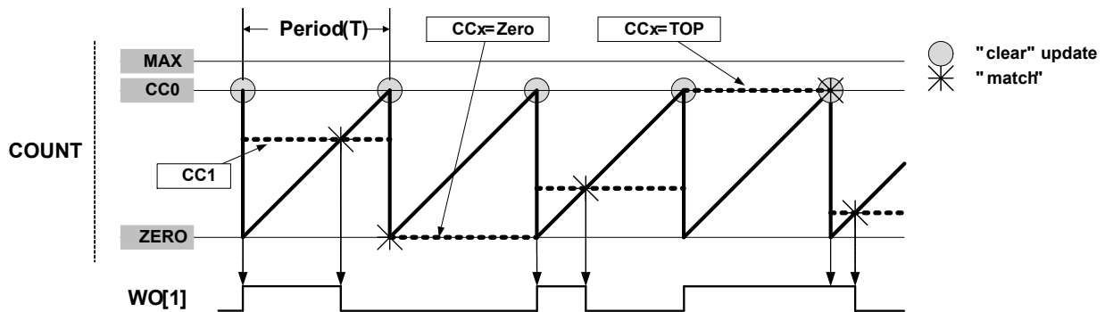
Figure 41-6. Match PWM Operation
