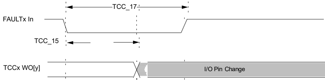
Figure 49-31. TCC_x Timer Compare Fault Output Module AC Timing Diagram
