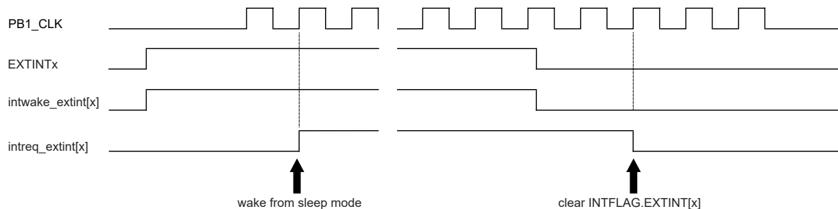
Figure 28-5. Wake-up Operation Example (High-Level Detection, No Filter, Interrupt Enable Set)
