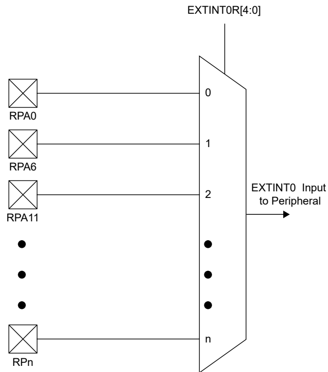
Figure 7-2. EXTINT0 Remappable Pin Selection
