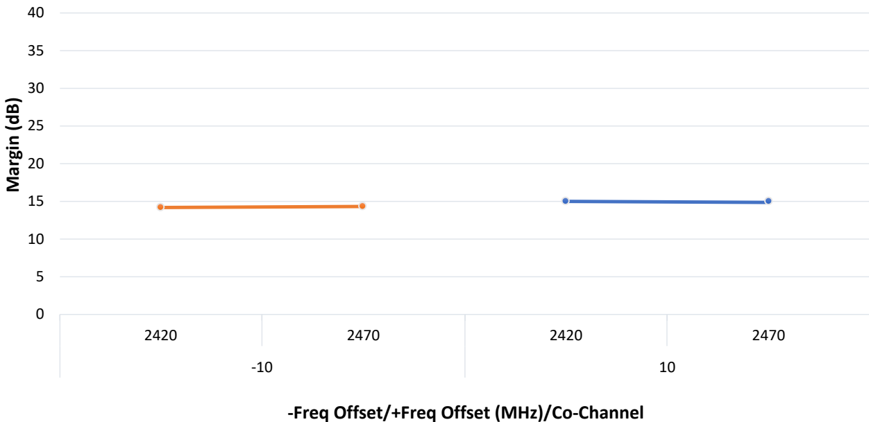
Figure 49-57. IEEE® 802.15.4 ACR RX CI 10M Margin
