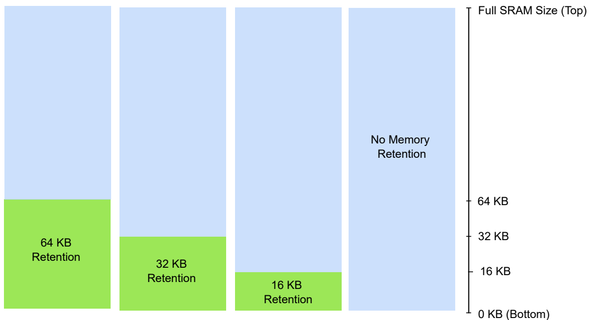
Figure 9-2. Retention Options
