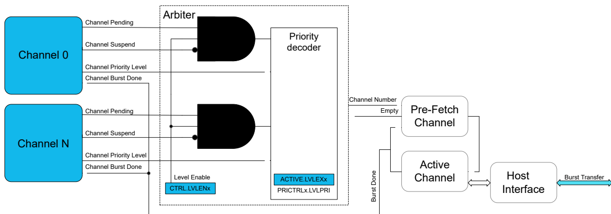
Figure 27-4. Arbiter Overview
