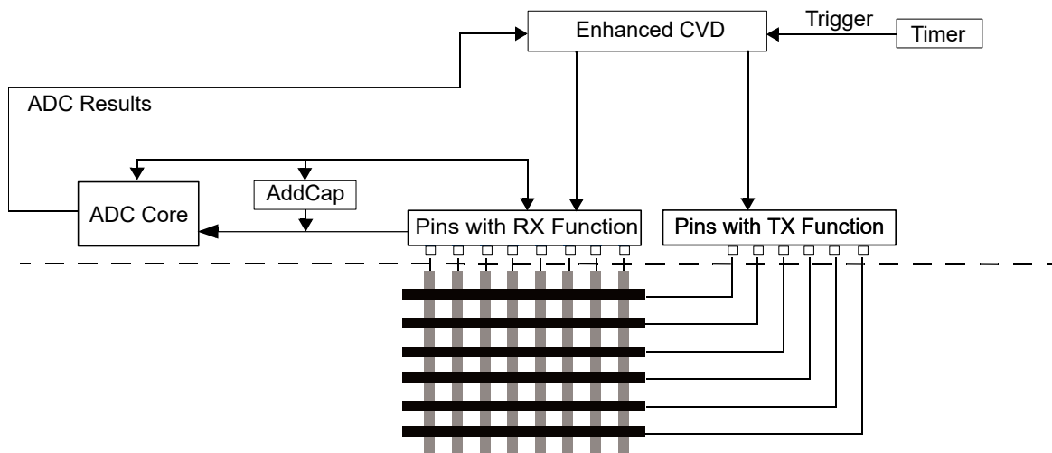
Figure 38-1. Enhanced Capacitive Voltage Divider (CVD) Controller Block Diagram
