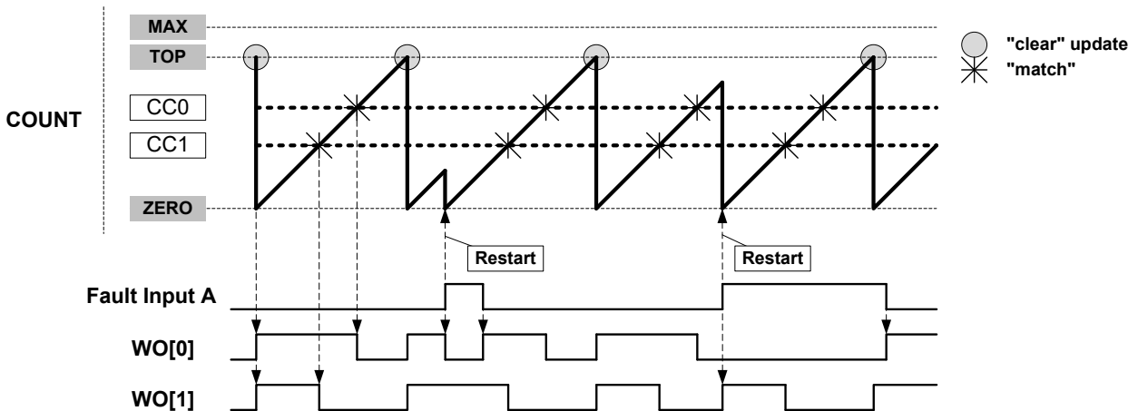
Figure 42-26. Waveform Generation in RAMP1 mode with Restart Action
