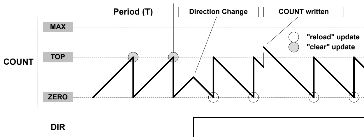
Figure 41-3. Counter Operation
