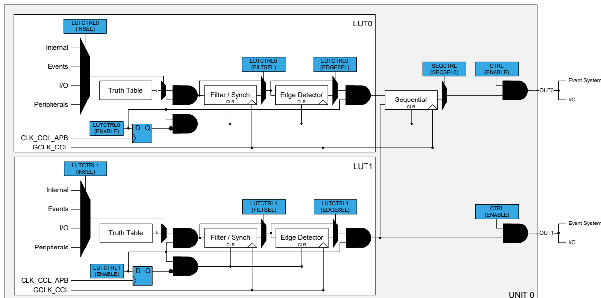
Figure 29-1. Configurable Custom Logic
