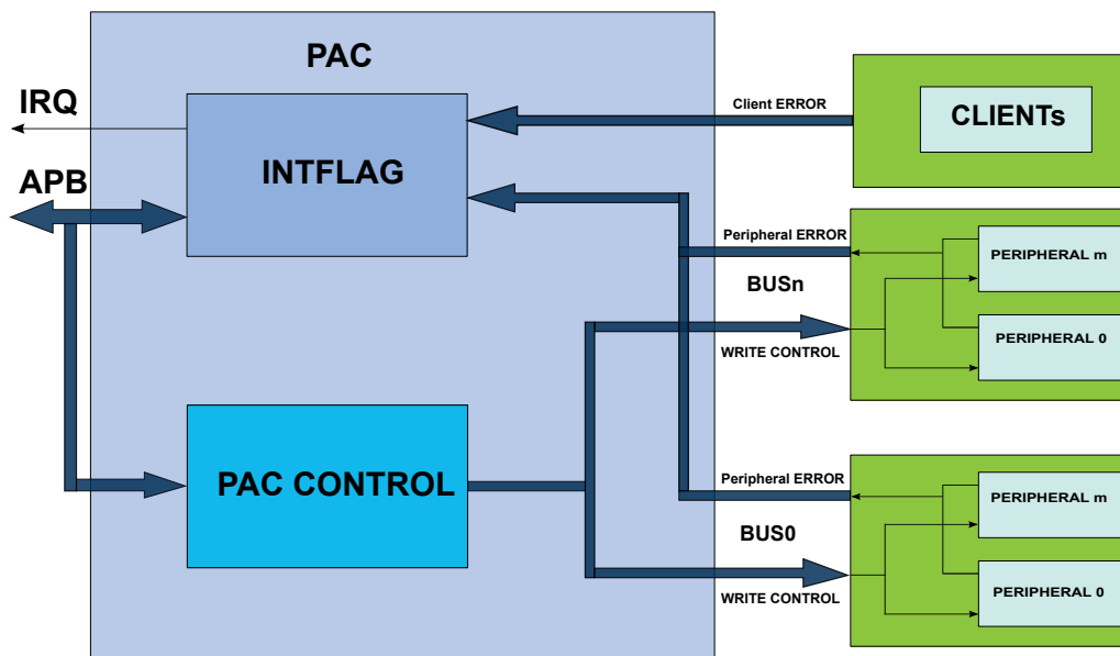
Figure 25-1. PAC Block Diagram
