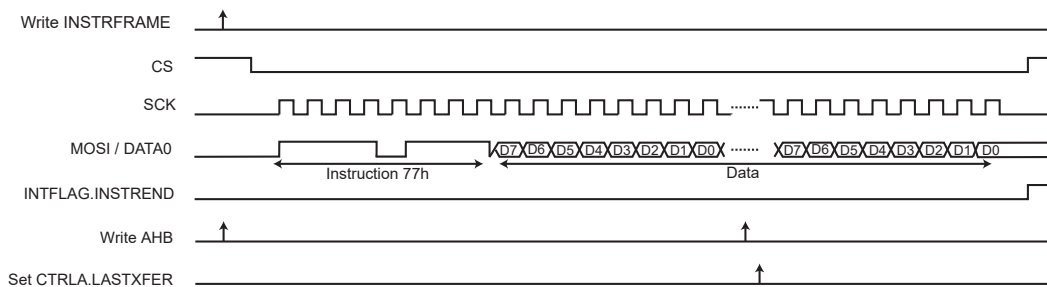
Figure 36-15. Instruction Transmission Waveform 4
