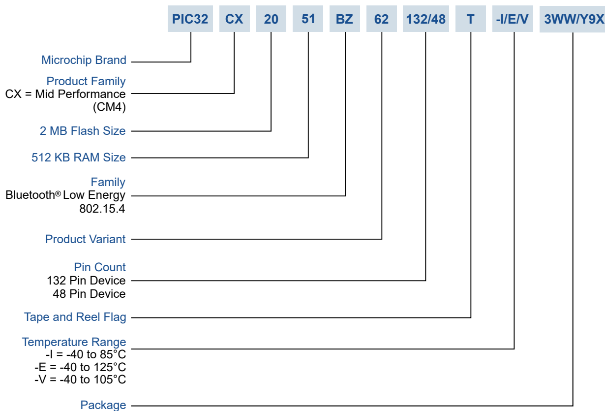
Figure 2-1. PIC32CX-BZ6 Ordering Information
