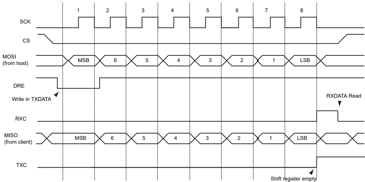
Figure 36-8. Interrupt Flags Behaviour
