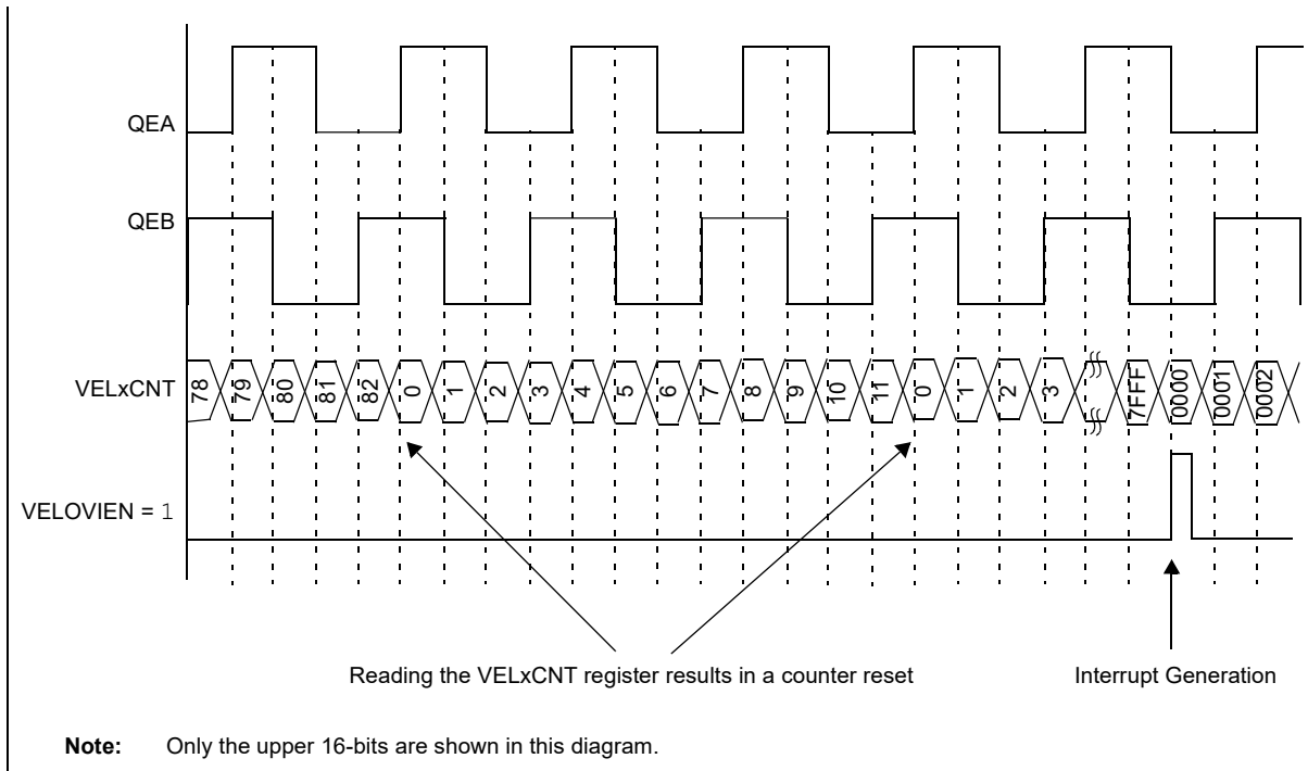
Figure 46-6. Velocity Counter
