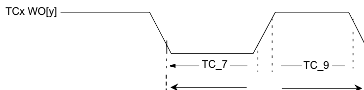
Figure 49-28. TCx Timer Capture Output Module AC Timing Diagram
