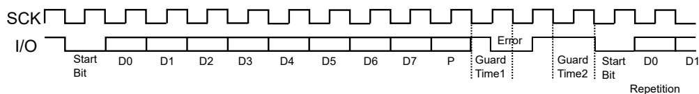
Figure 33-19. T = 0 Protocol with Parity Error
