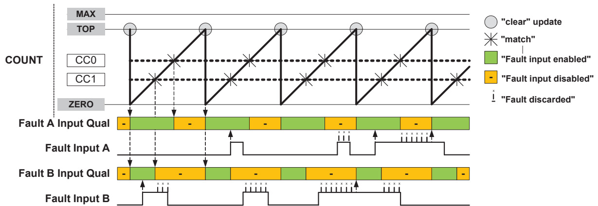
Figure 42-24. Fault Qualification in RAMP2 Operation with Inverted Polarity
