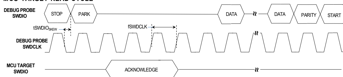
Figure 49-34. SWD Two-Wire Read/Write AC Timing Diagram
