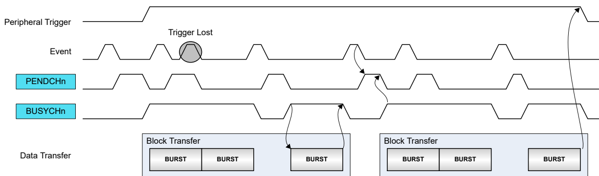
Figure 27-12. Burst Event Trigger Action
