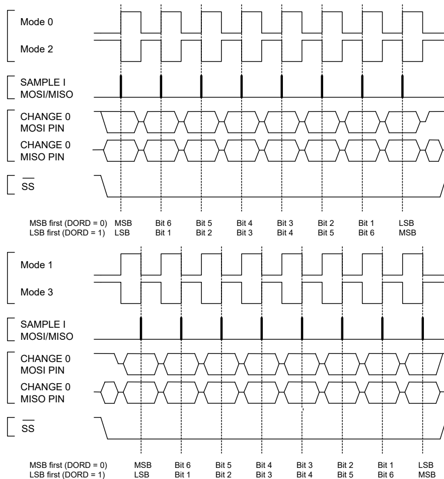
Figure 34-3. SPI Transfer Modes
