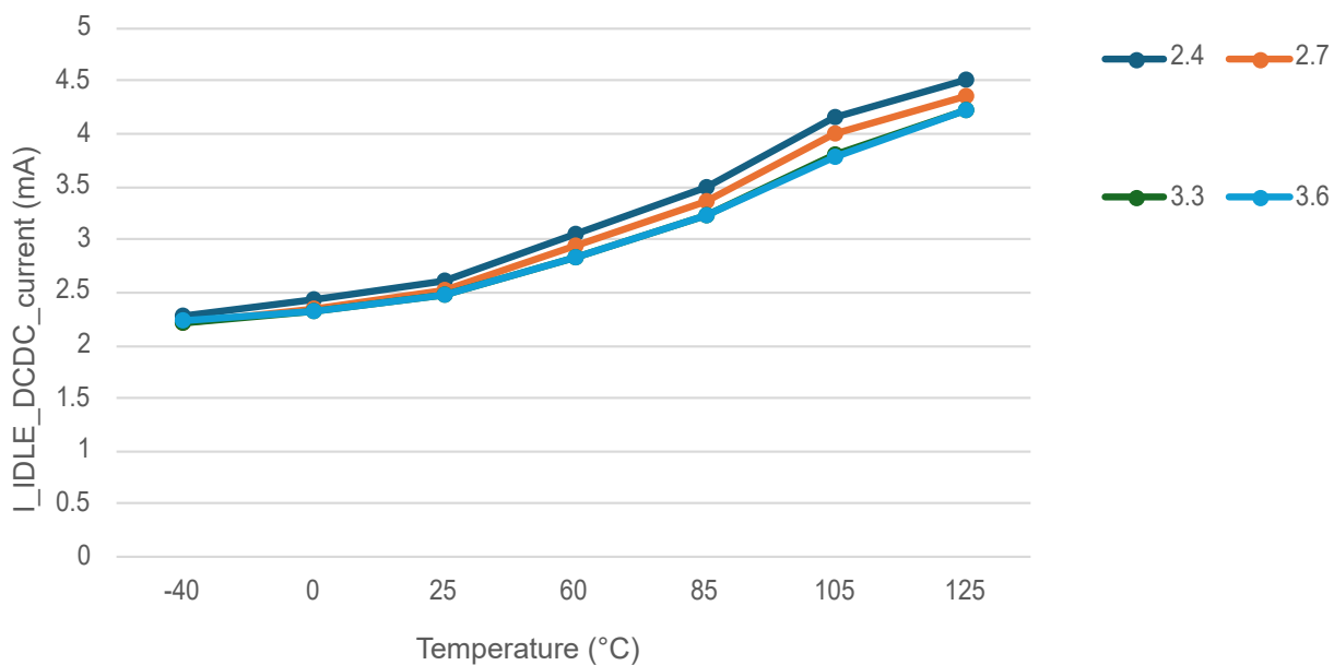
Figure 49-8. Idle Mode Current Consumption in Buck Mode at FRC 8 MHz
