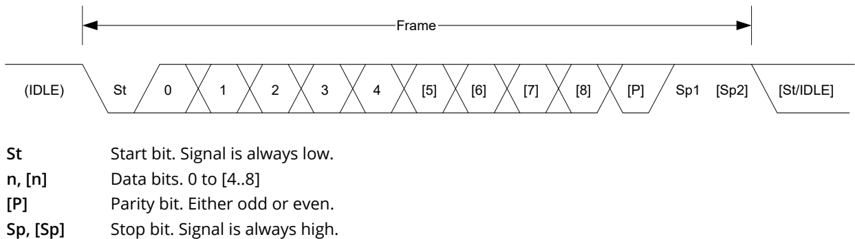
Figure 33-2. Frame Formats
