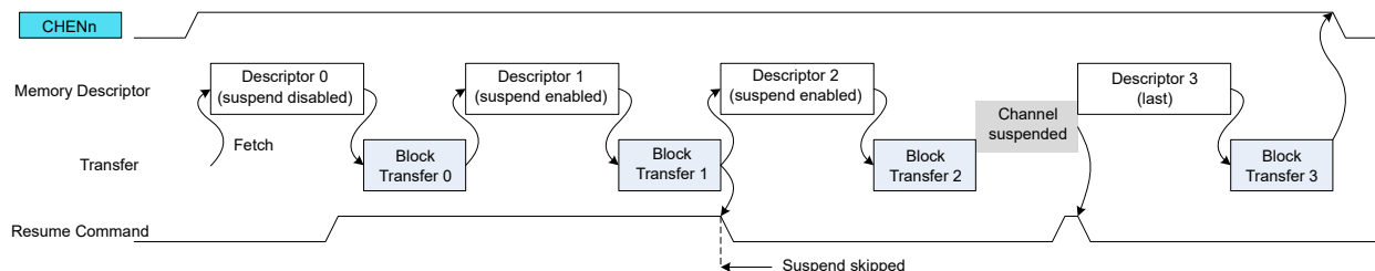
Figure 27-11. Channel Suspend/Resume Operation
