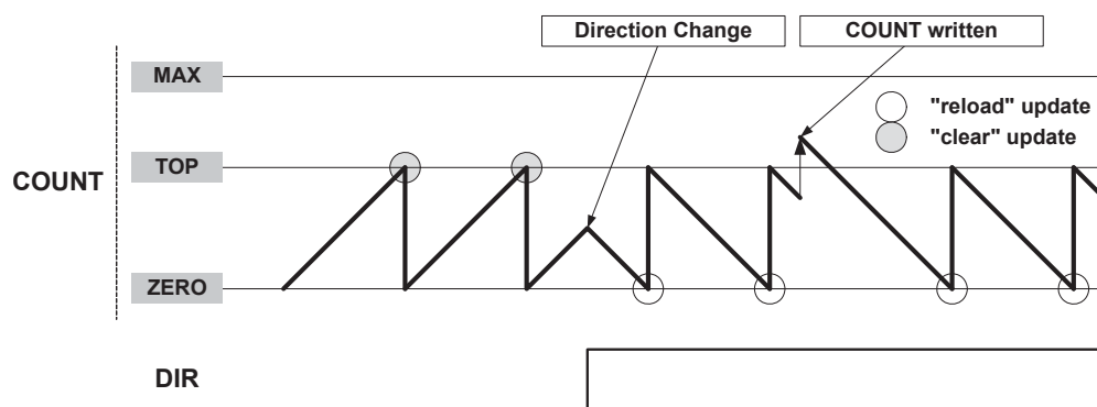
Figure 42-3. Counter Operation
