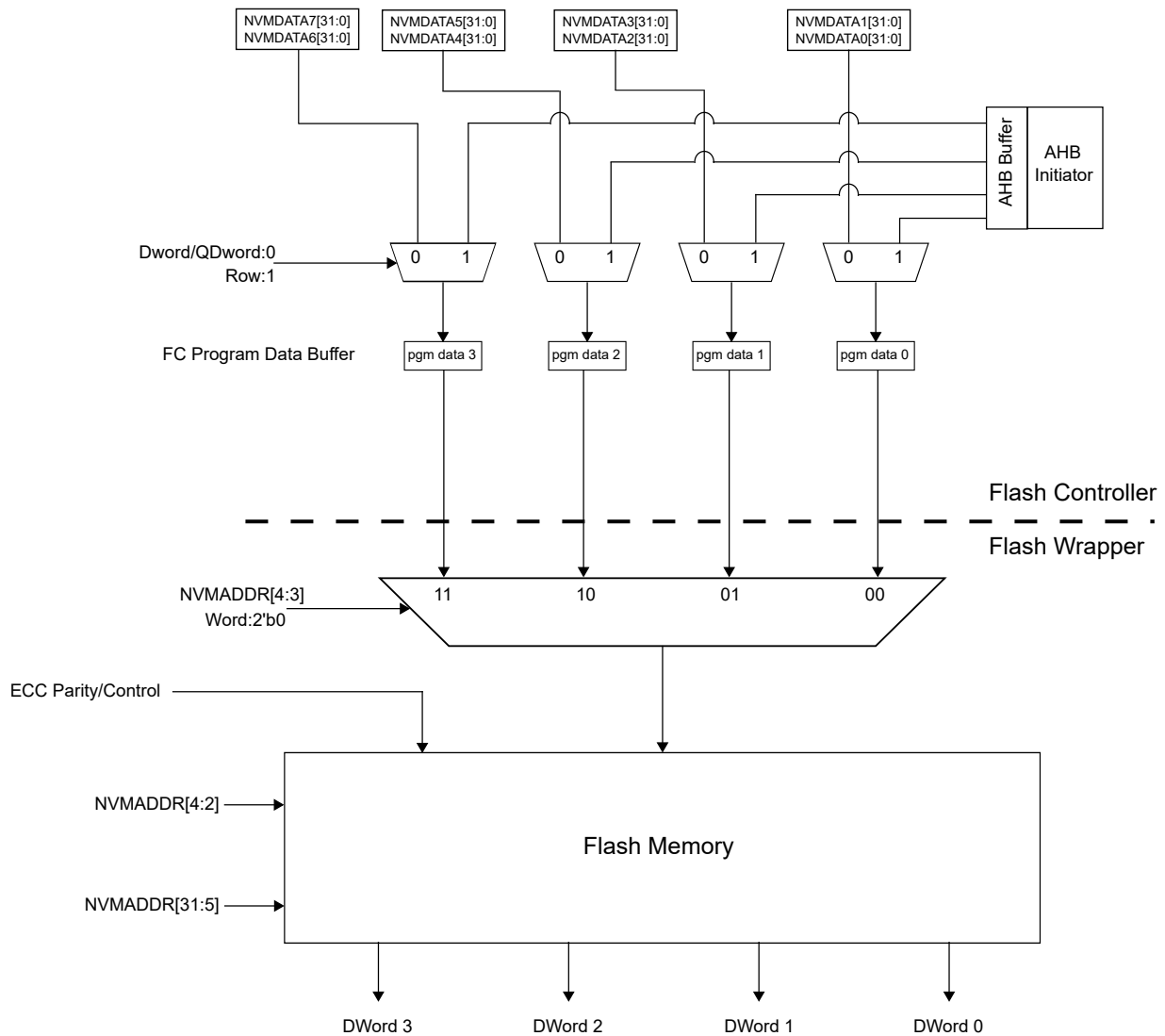
Figure 16-1. Flash Memory Block Diagram
