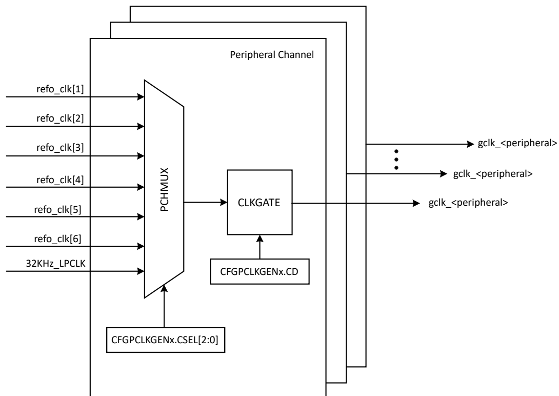
Figure 18-5. Peripheral Clock Generation (GCLK)
