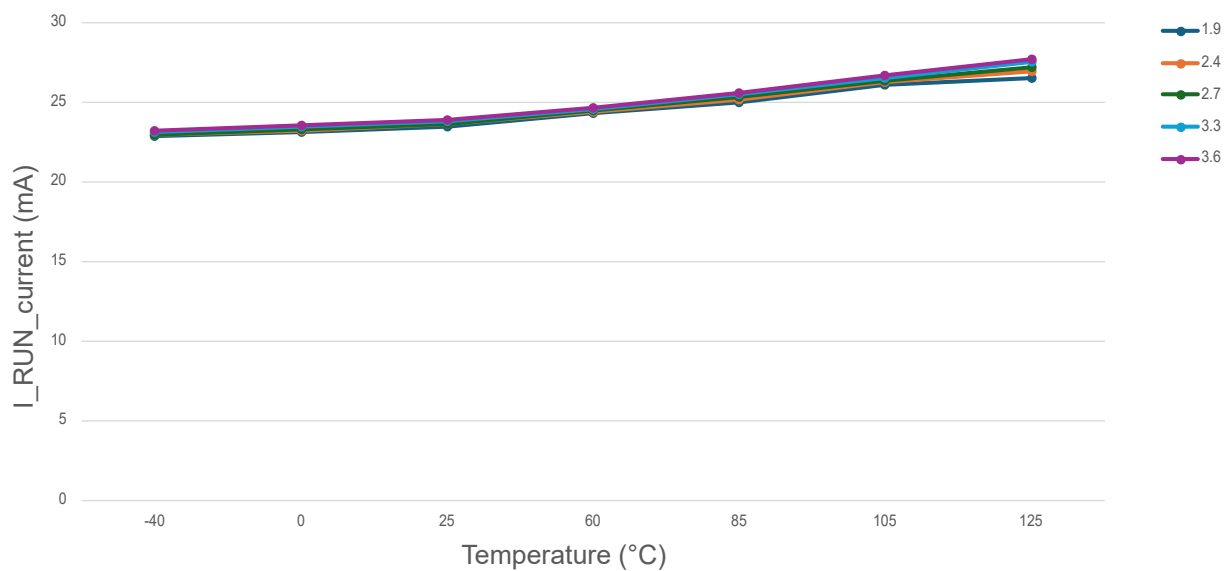
Figure 49-2. Run Mode Current Consumption in MLDO Mode at FRC 8 MHz
