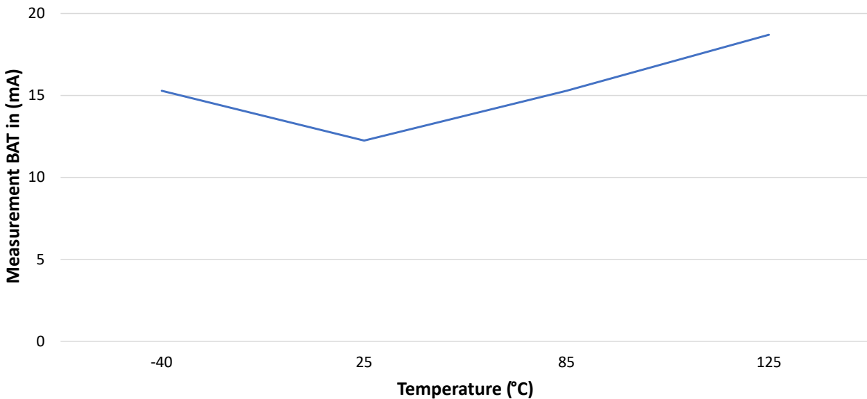
Figure 49-42. Bluetooth Low Energy Receive Current vs. Temperature
