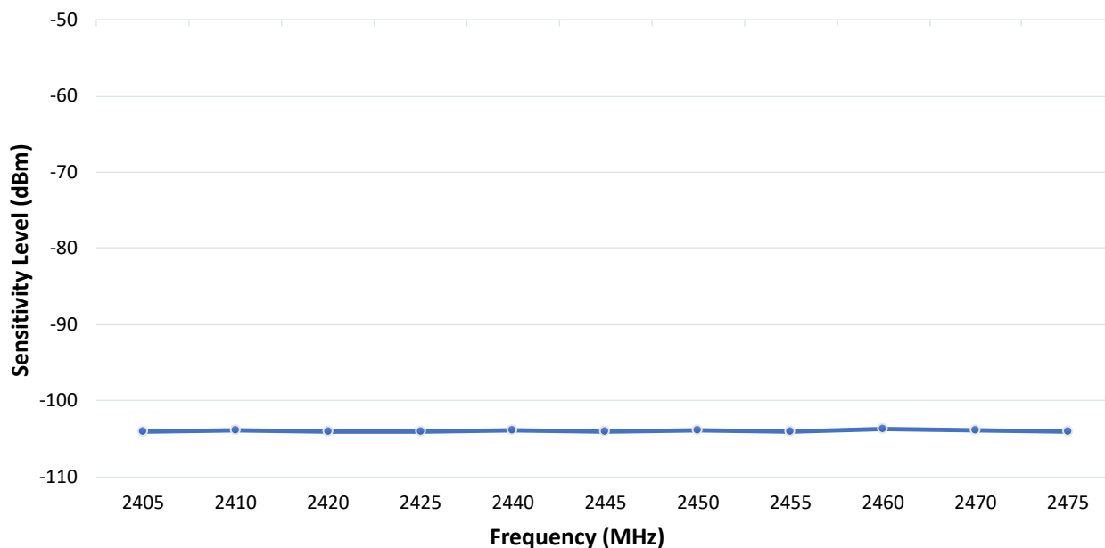
Figure 49-59. Module IEEE® 802.15.4 Receive Sensitivity vs. Frequency
