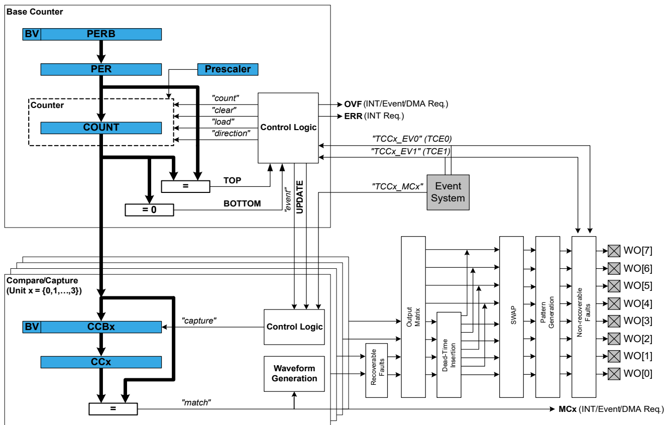
Figure 42-1. Timer/Counter for Control Applications - Block Diagram
