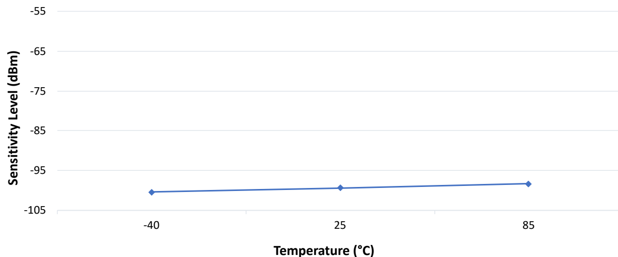
Figure 49-45. Module Bluetooth Low Energy Receive Sensitivity vs. Temperature
