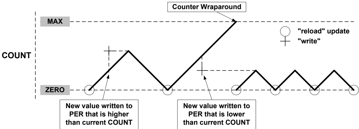
Figure 42-12. Unbuffered Dual-Slope Operation
