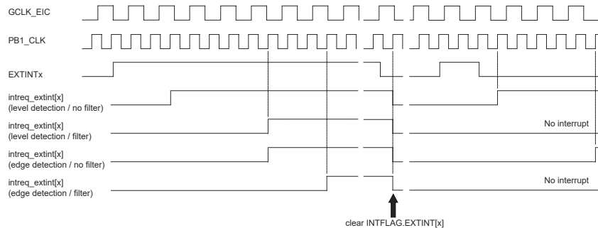
Figure 28-2. Interrupt Detection Latency by Modes (Rising Edge)
