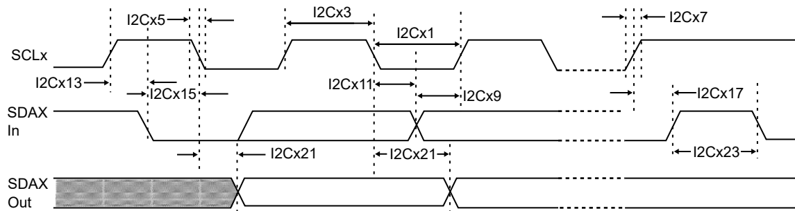
Figure 49-23. I 2 C Bus Data Host Mode AC Timing Diagram
