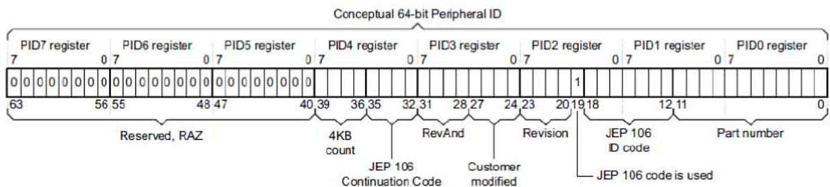
Figure 17-5. Conceptual 64-bit Peripheral ID
