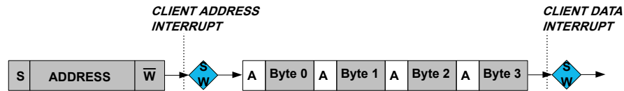
Figure 35-13. 32-Bit Extension Client Operation
