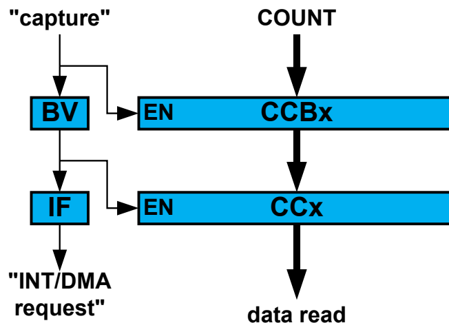
Figure 42-15. Capture Double Buffering
