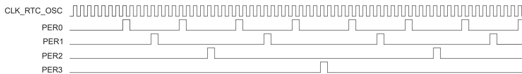
Figure 26-5. Example Periodic Events
