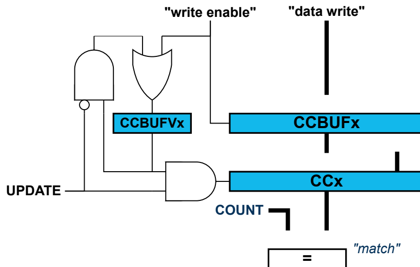
Figure 41-7. Compare Channel Double Buffering
