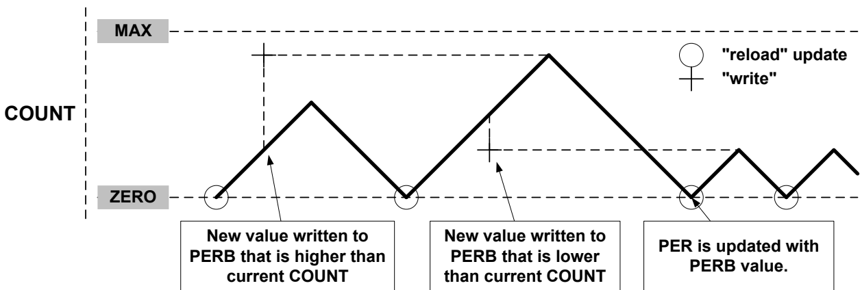
Figure 42-13. Changing the Period Using Buffering
