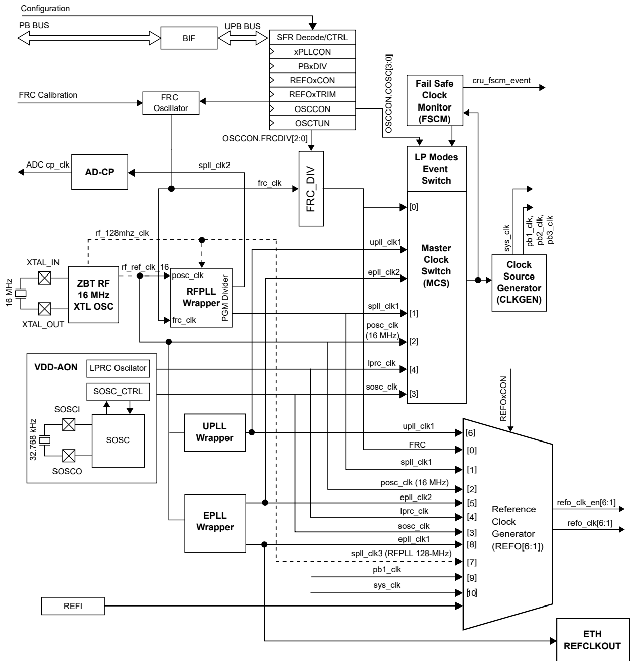
Figure 18-1. Clock System Block Diagram
