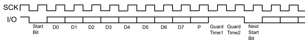
Figure 33-18. T = 0 Protocol without Parity Error
