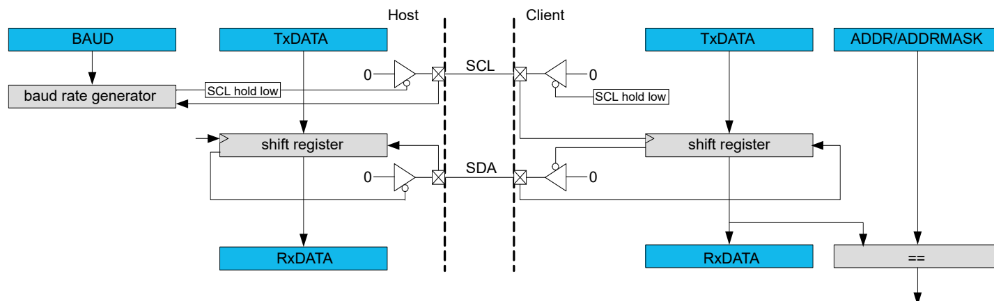
Figure 35-1. I 2 C Single-Host Single-Client Interconnection
