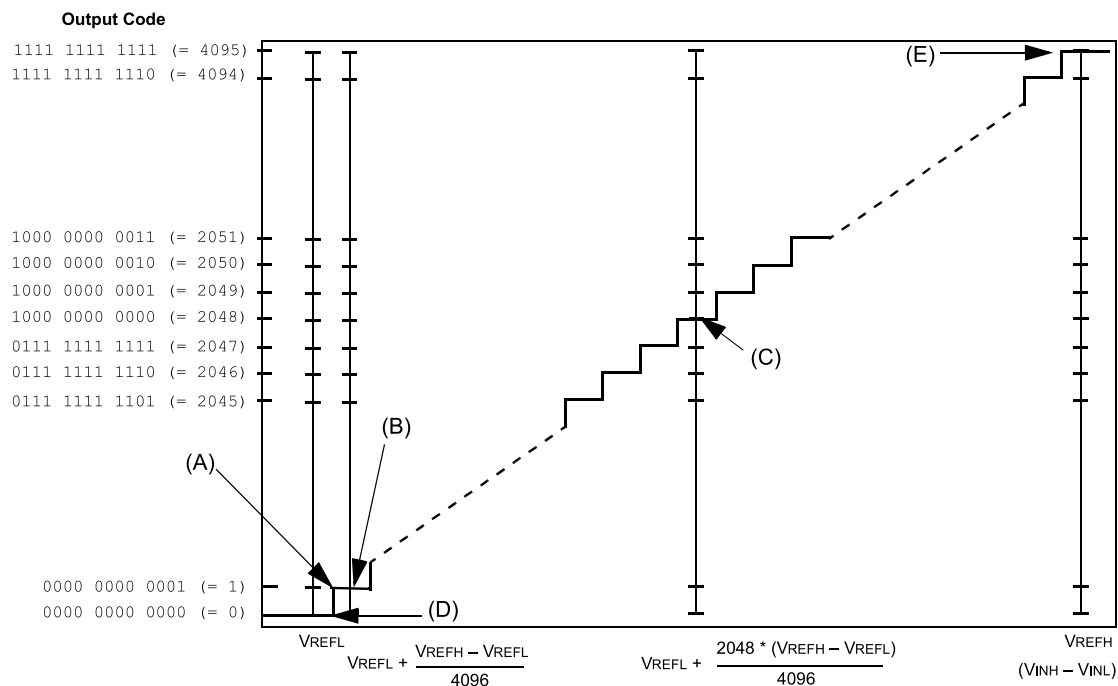
Figure 37-11. Analog-to-Digital Transfer Function
