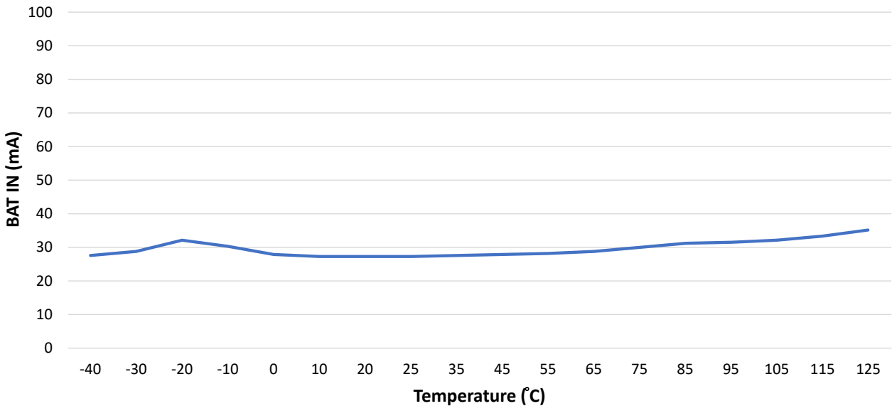
Figure 49-51. IEEE® 802.15.4 Transmit Current vs. Temperature
