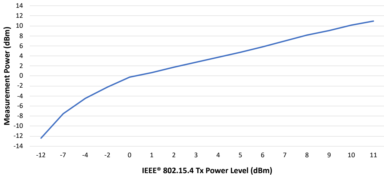
Figure 49-50. IEEE® 802.15.4 Transmit Power vs. Power Level
