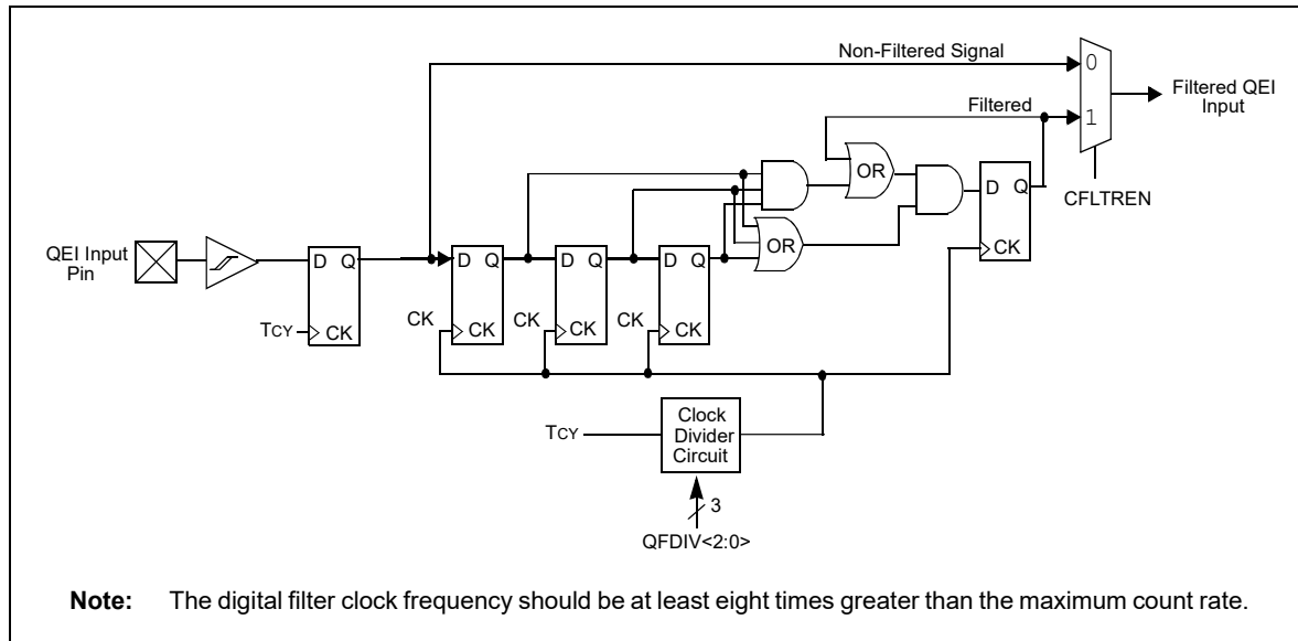
Figure 46-9. Block Diagram of Digital Noise Filter
