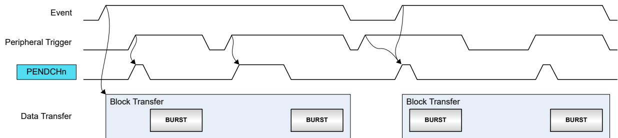
Figure 27-15. Conditional Block Transfer with Burst Peripheral Triggers
