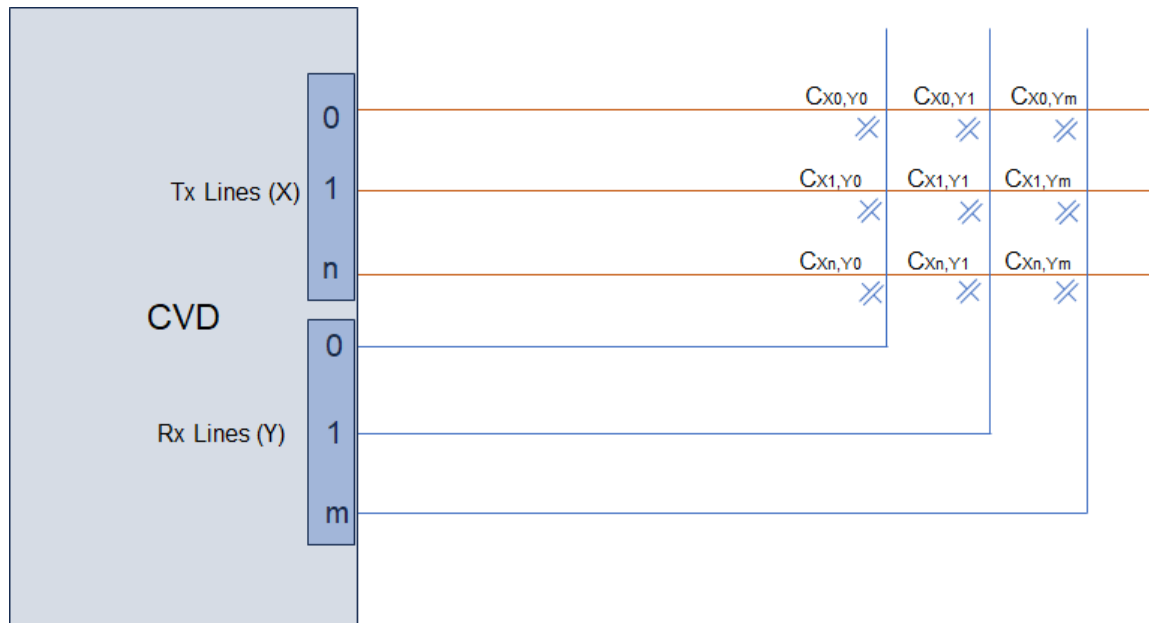
Figure 38-3. Typical Mutual Cap Sensor Arrangements
