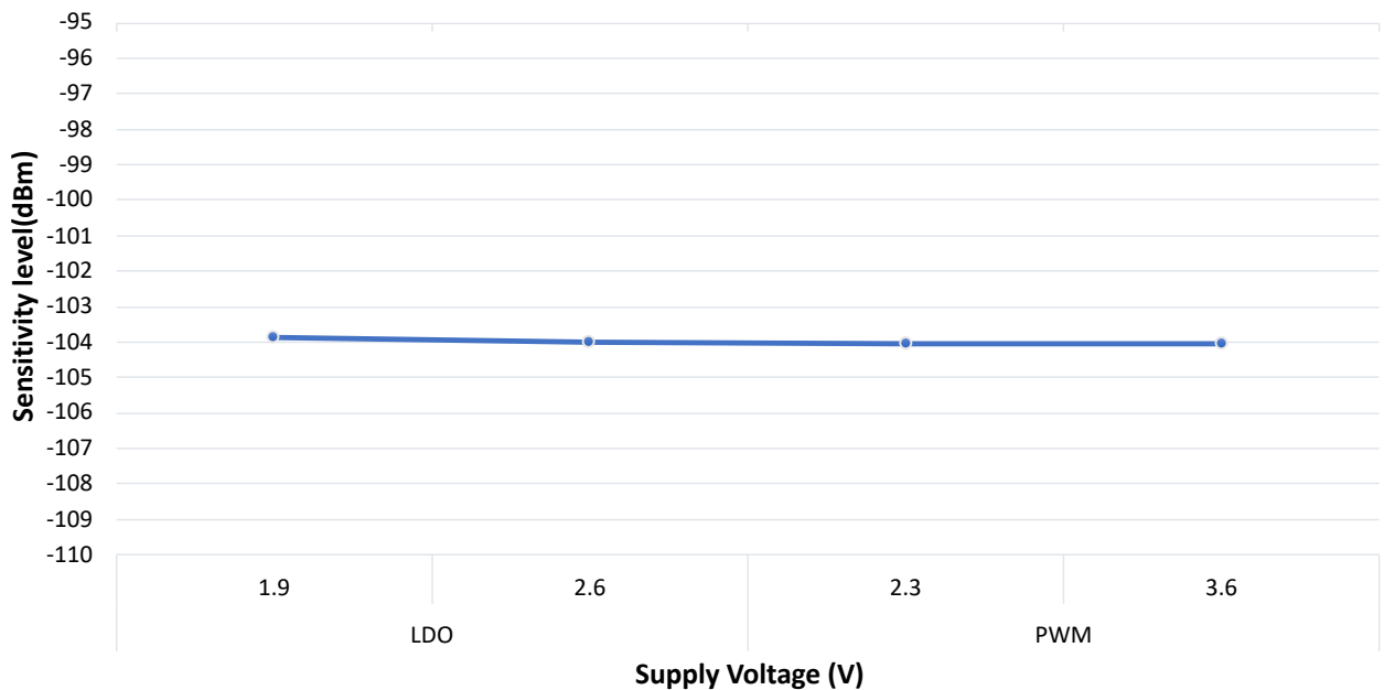
Figure 49-52. IEEE® 802.15.4 Receive Sensitivity vs. Voltage
