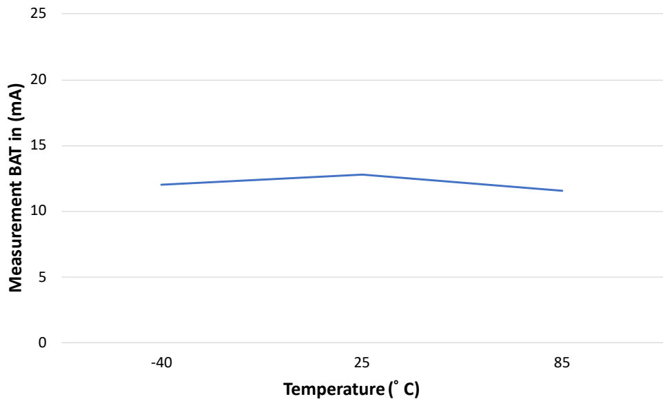
Figure 49-44. Module Bluetooth Low Energy Receive Current vs. Temperature
