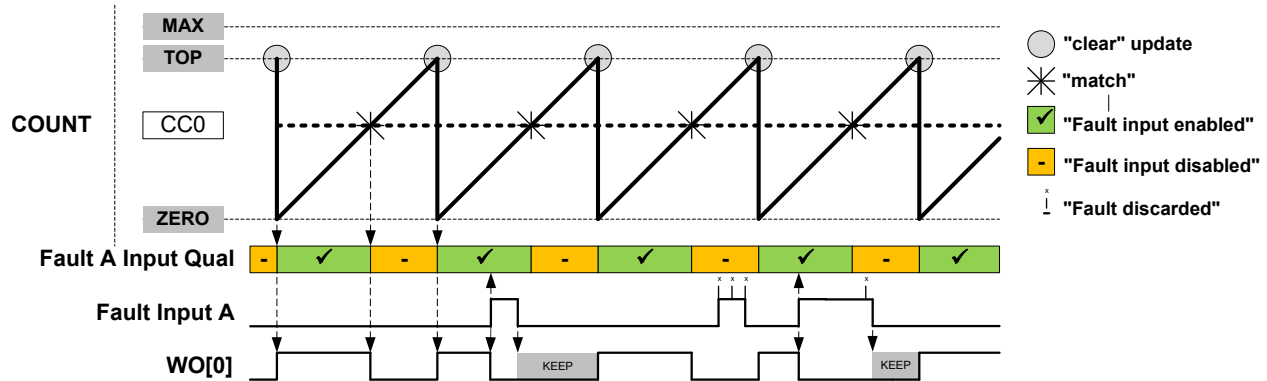
Figure 42-25. Waveform Generation with Fault Qualification and Keep Action
