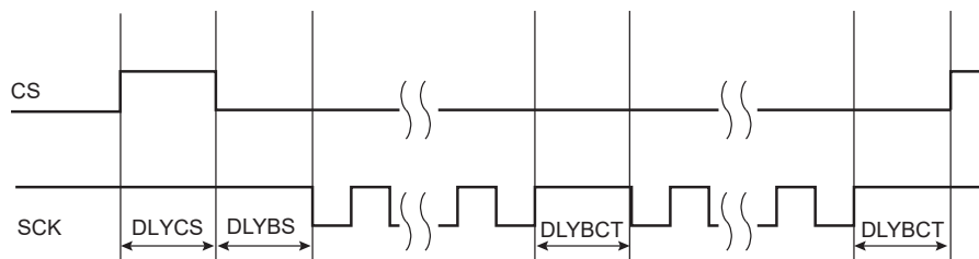
Figure 36-5. Programmable Delay
