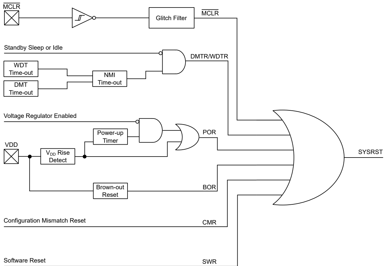
Figure 18-8. CRU-System Reset Block Diagram
