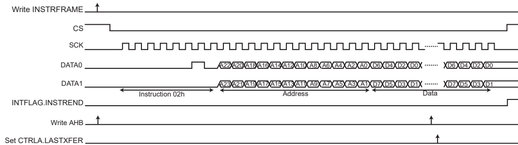
Figure 36-16. Instruction Transmission Waveform 5
