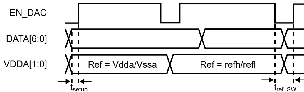
Figure 40-2. DAC Timing Diagram
