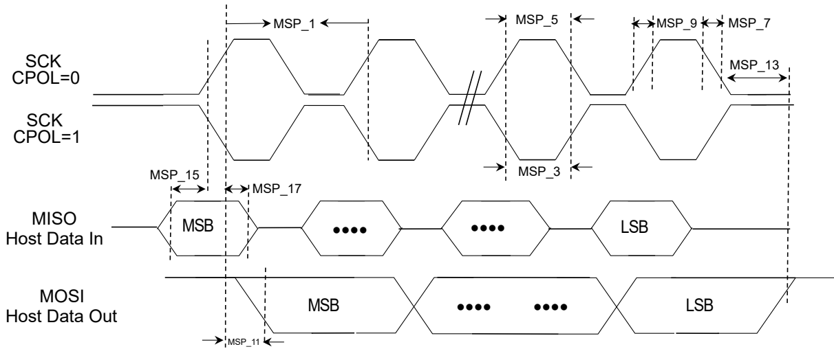
Figure 49-19. SPI Host Module CPHA = 1 Timing Diagrams
