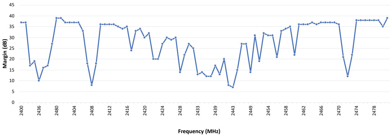
Figure 49-43. Bluetooth Low Energy Rx CI Margin
