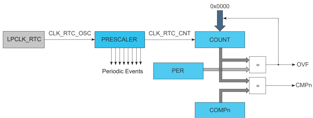
Figure 26-2. RTCC Block Diagram (Mode 1 — 16-Bit Counter)
