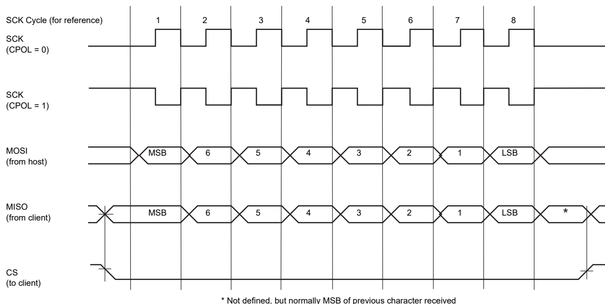
Figure 36-3. QSPI Transfer Modes (BAUD.CPHA = 0, 8-bit transfer)
