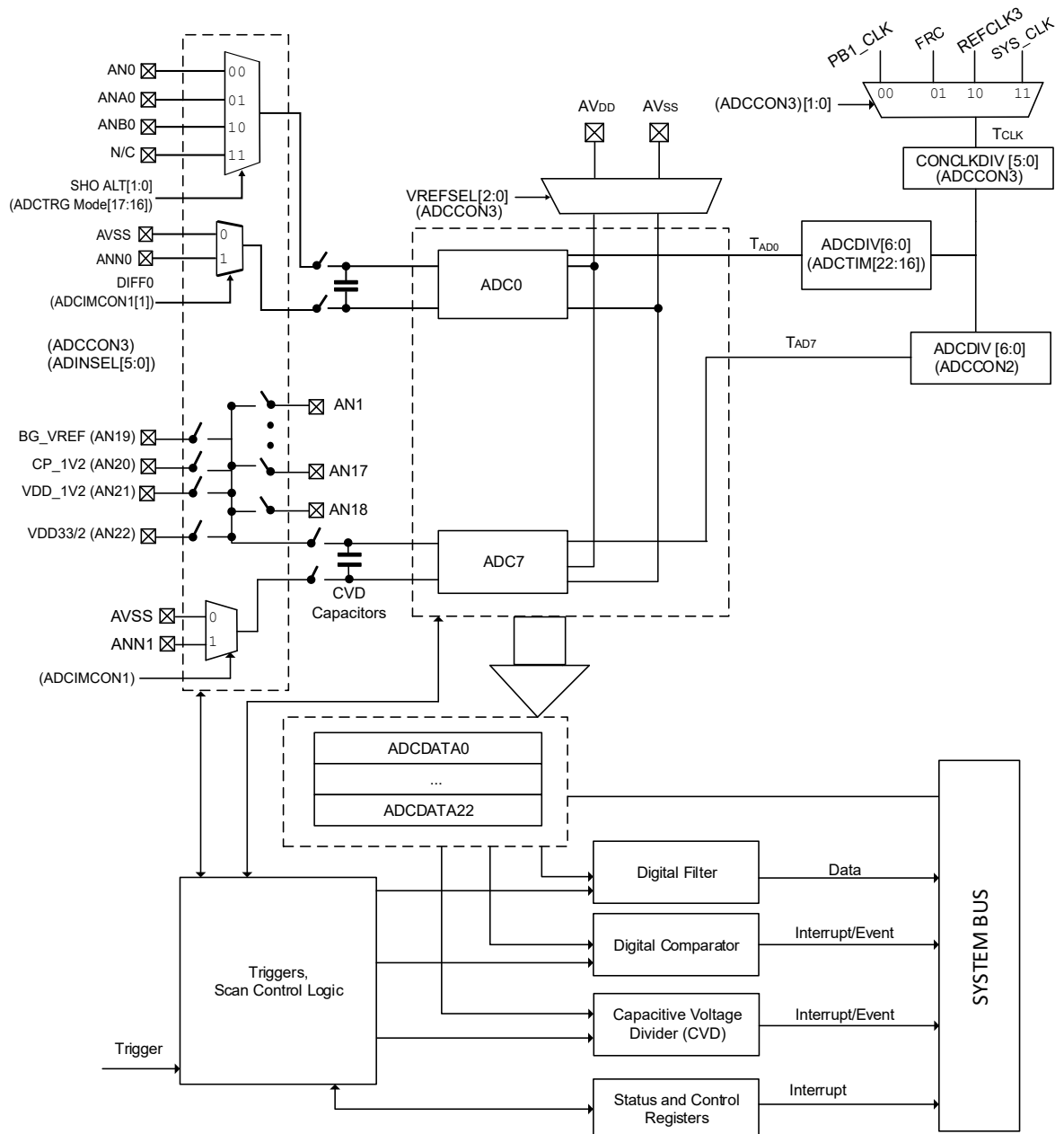
Figure 37-1. ADC Block Diagram
