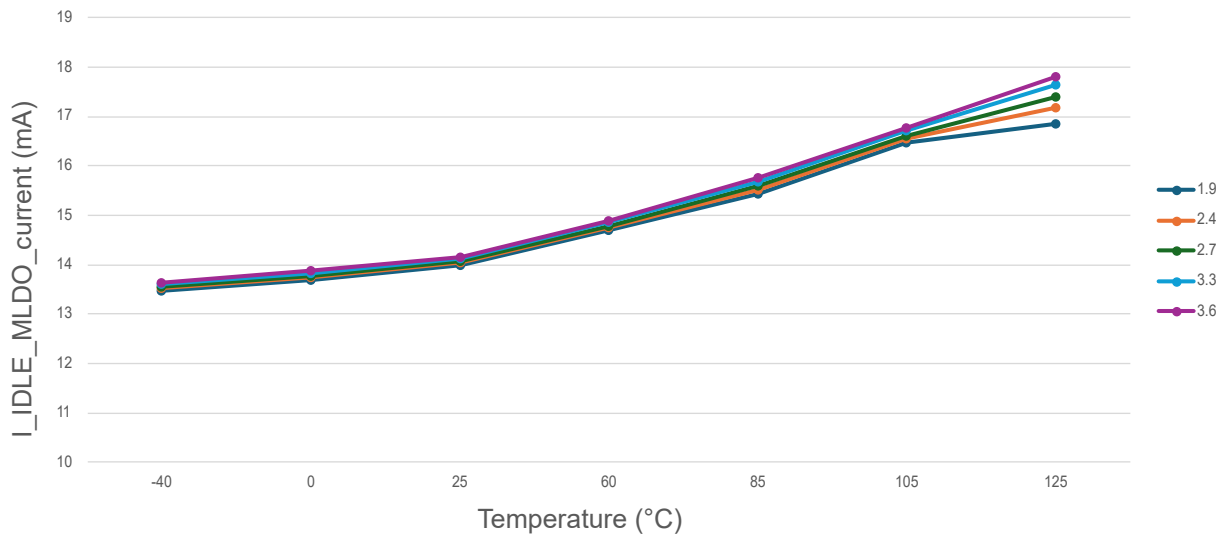
Figure 49-5. Idle Mode Current Consumption in MLDO Mode at PLL 128 MHz
