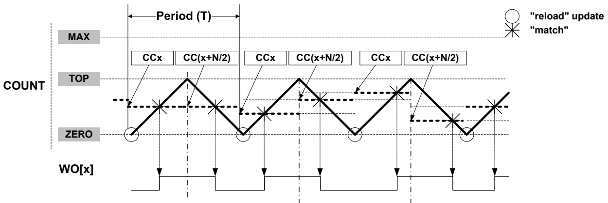
Figure 42-8. Dual-Slope Critical Pulse Width Modulation ( N=\text{CC\_NUM} )
