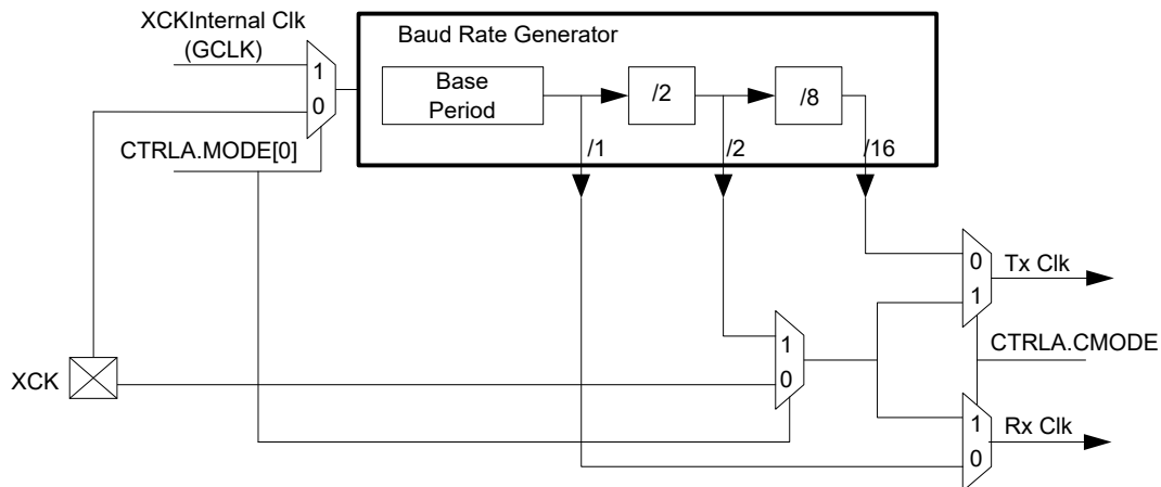
Figure 33-3. Clock Generation
