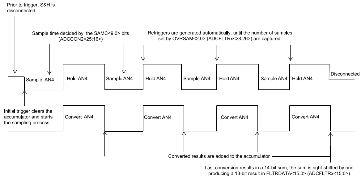
Figure 37-9. 4x Oversampling of a Class 2 Input
