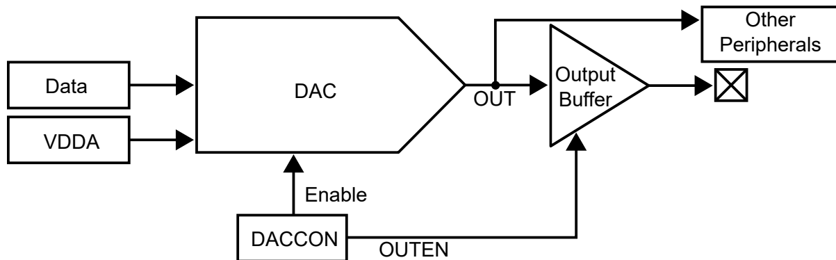
Figure 40-1. Block Diagram
