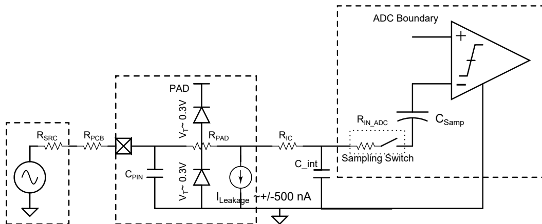
Figure 37-12. 12-bit ADC Analog Input Model
