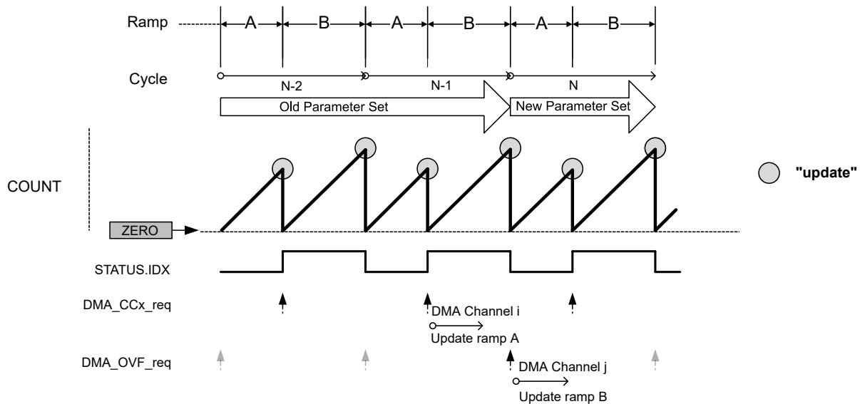
Figure 42-38. DMA Triggers in RAMP and RAMP2 Operation Mode and Circular Buffer Enabled
