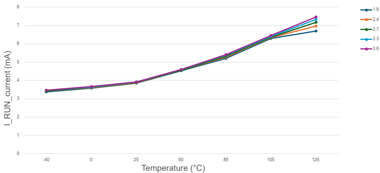
Figure 49-2. Run Mode Current Consumption in MLDO Mode at FRC 8 MHz
