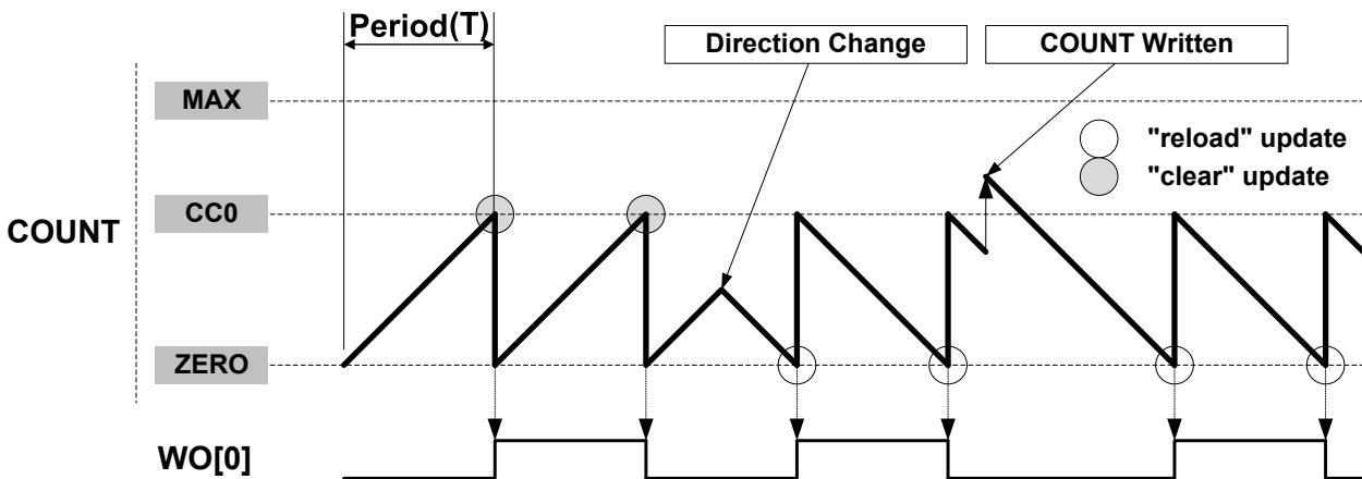
Figure 42-5. Match Frequency Operation
