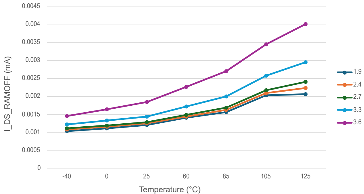
Figure 49-13. Deep Sleep Current RAM OFF
