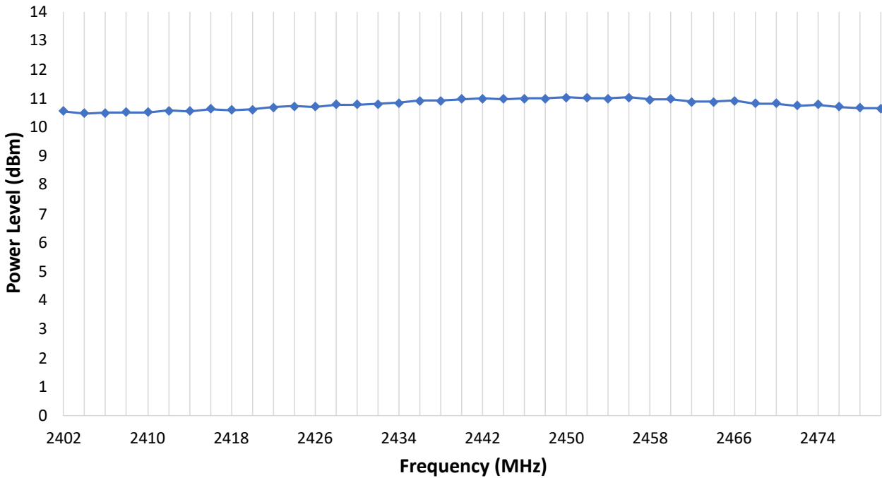
Figure 49-37. Bluetooth Low Energy Transmit Power vs. Frequency
