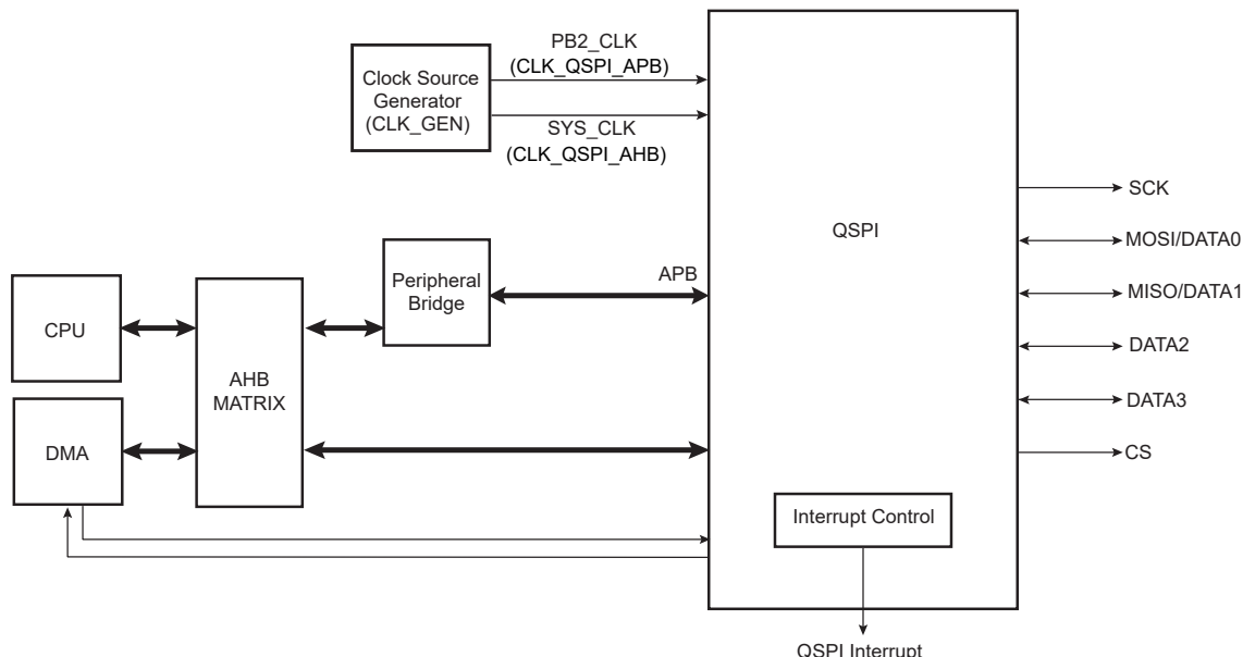
Figure 36-1. QSPI Block Diagram
