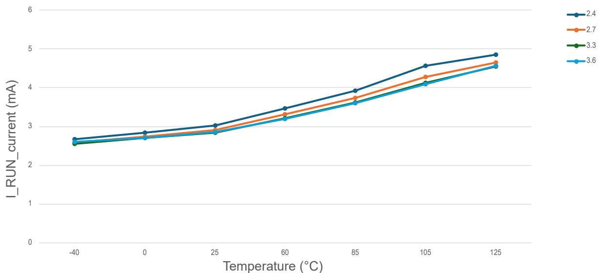
Figure 49-4. Run Mode Current Consumption in Buck Mode at FRC 8 MHz
