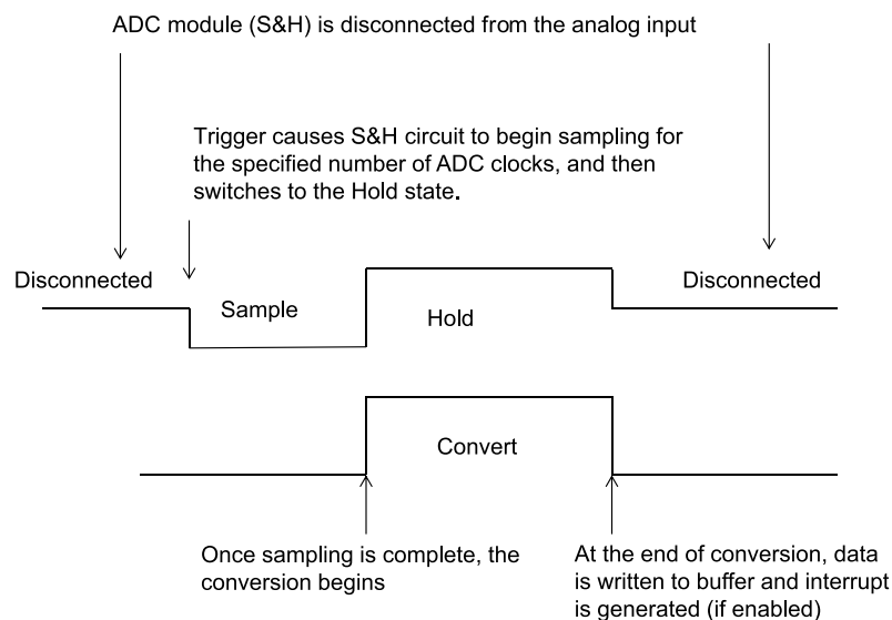
Figure 37-3. Sample and Conversion Sequence for Shared ADC Cores
