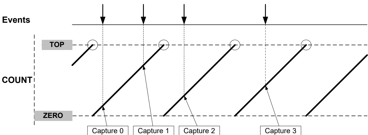
Figure 41-12. Input Capture Timing
