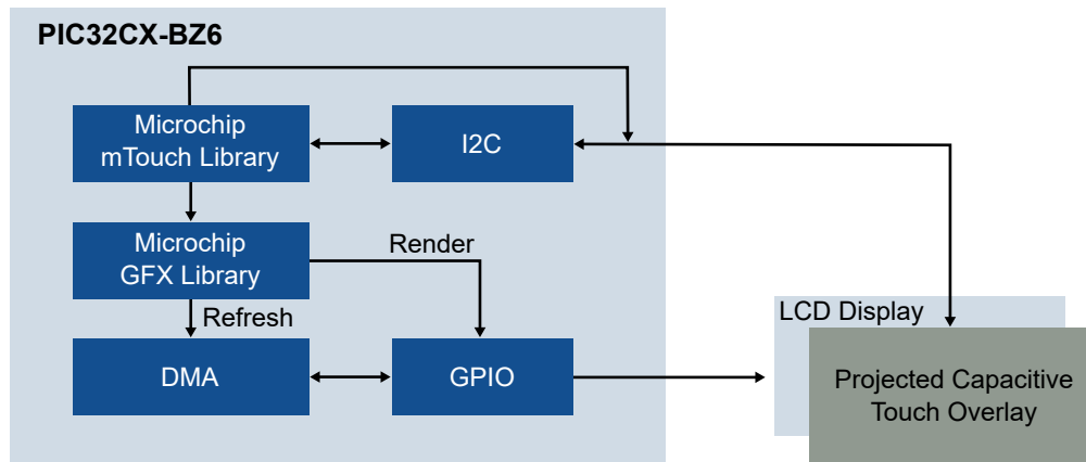
Figure 47-1. Block Diagram of Low-Cost Controllerless Graphics Implementation Using GFX Library
