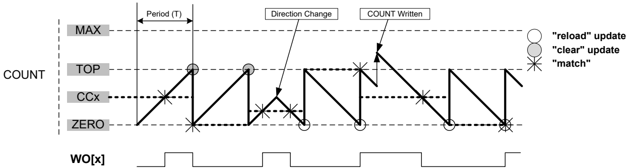
Figure 42-4. Normal Frequency Operation
