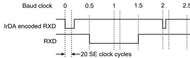
Figure 33-11. IrDA Receive Decoding
