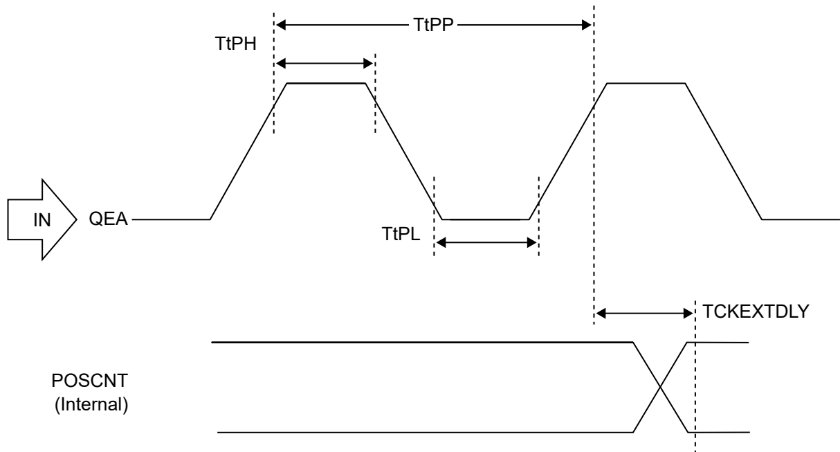
Figure 49-32. Quadrature Encoder (QEI) Counter Mode AC Timing Diagram
