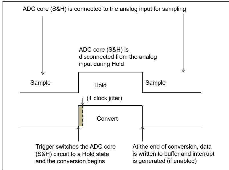
Figure 37-2. Sample and Conversion Sequence for Dedicated ADC Cores
