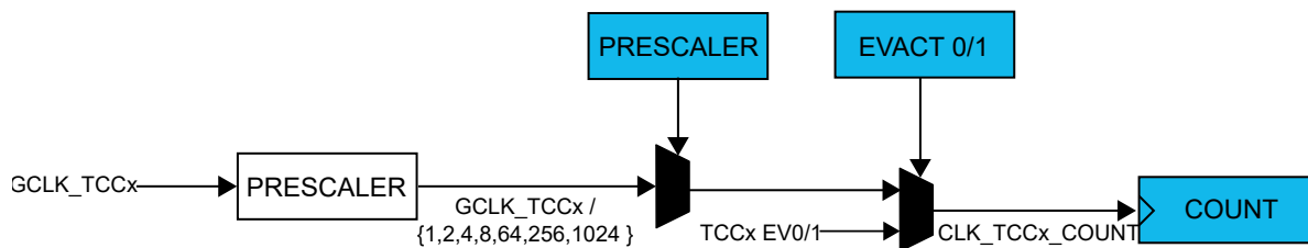
Figure 42-2. Prescaler
