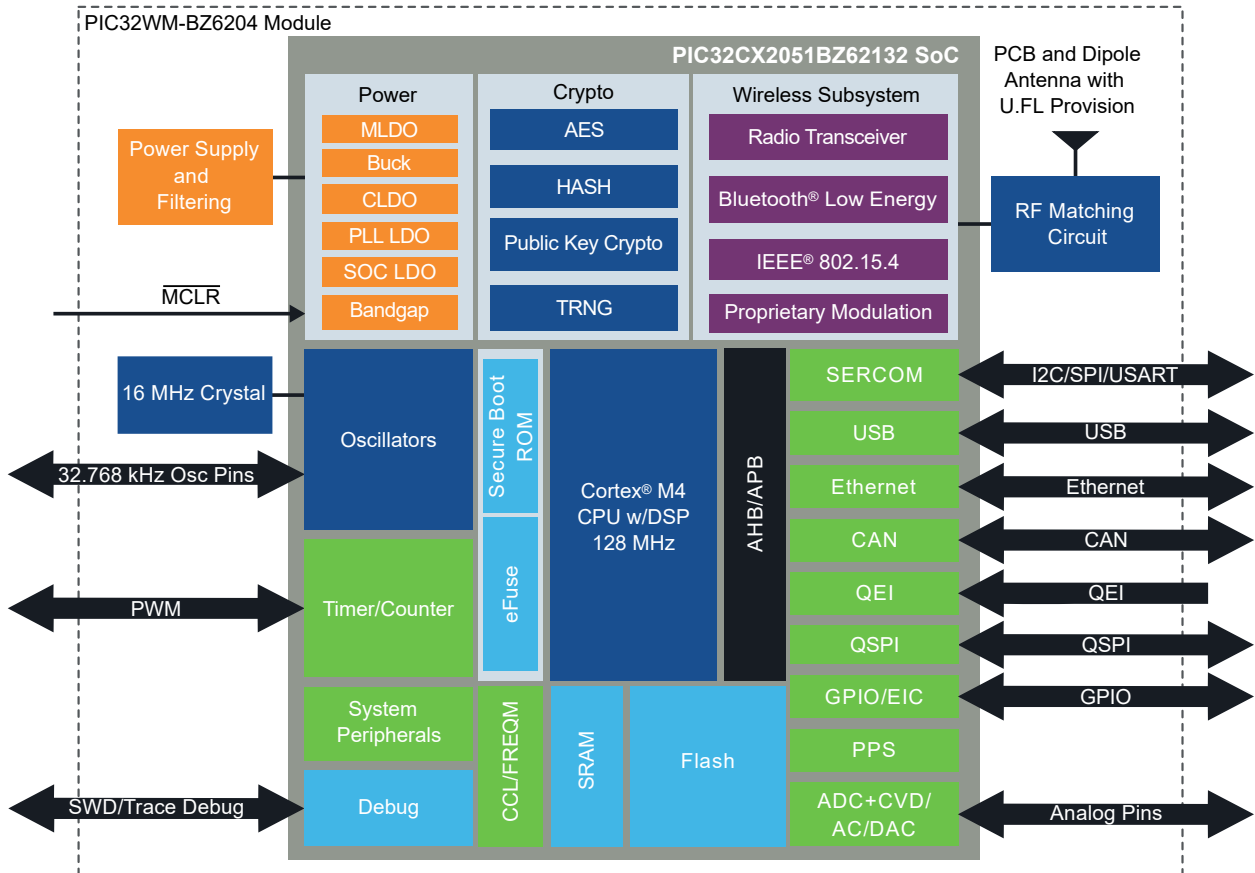
Figure 5-1. PIC32WM-BZ6204 Module Block Diagram
