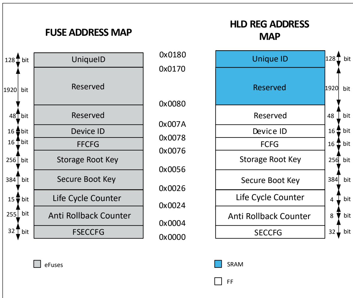
Figure 14-1. Memory Map of the Fuse Panels
