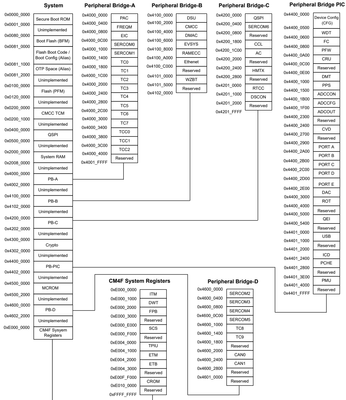
Figure 9-1. Product Mapping
