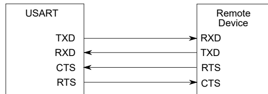
Figure 33-7. Connection with a Remote Device for Hardware Handshaking
