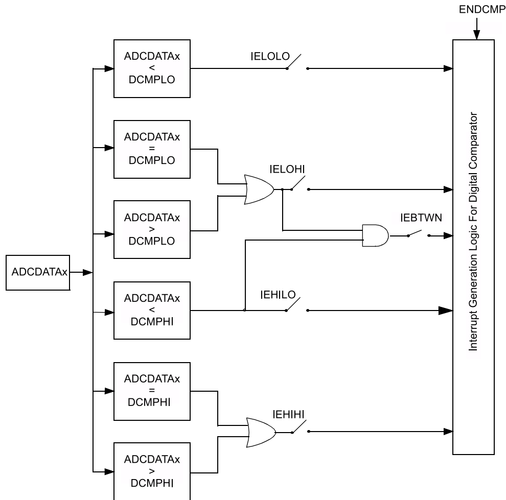
Figure 37-8. Digital Comparator
