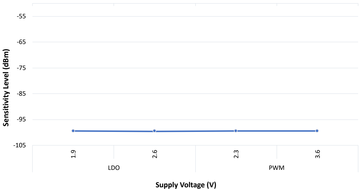
Figure 49-40. Bluetooth Low Energy Receive Sensitivity vs. Voltage
