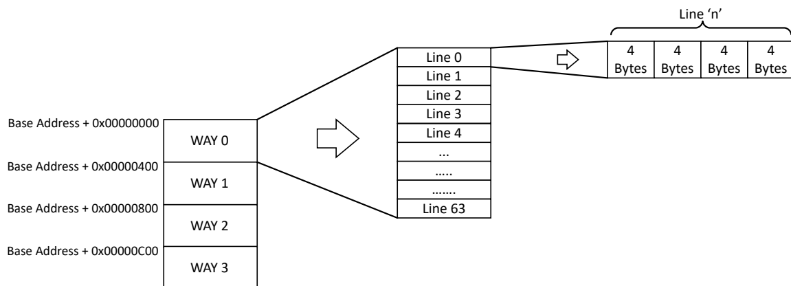
Figure 12-2. CMCC Organization
