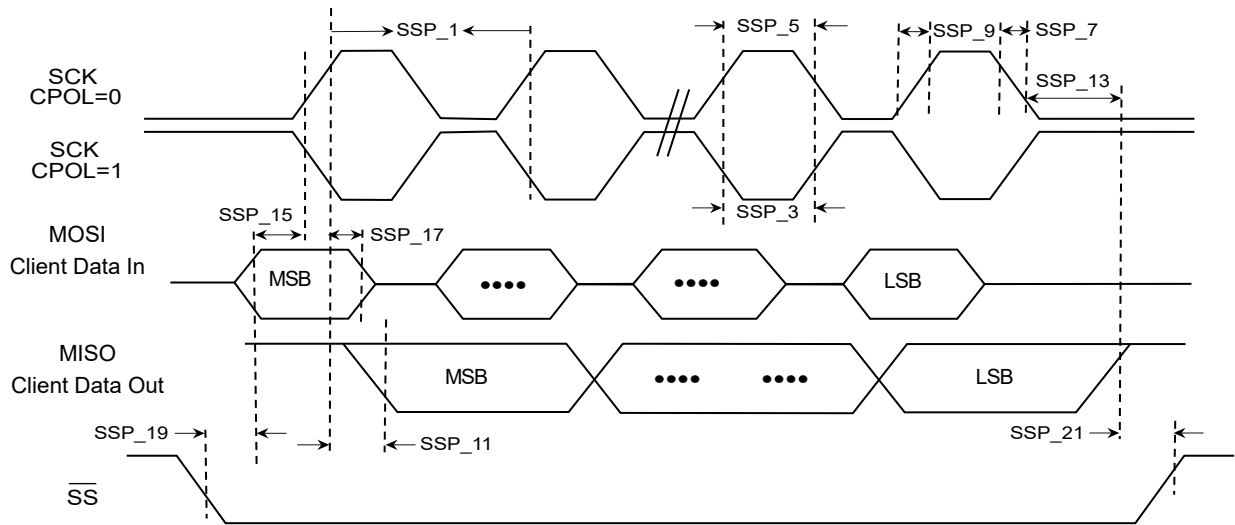
Figure 49-21. SPI Client Module CPHA = 1 Timing Diagrams
