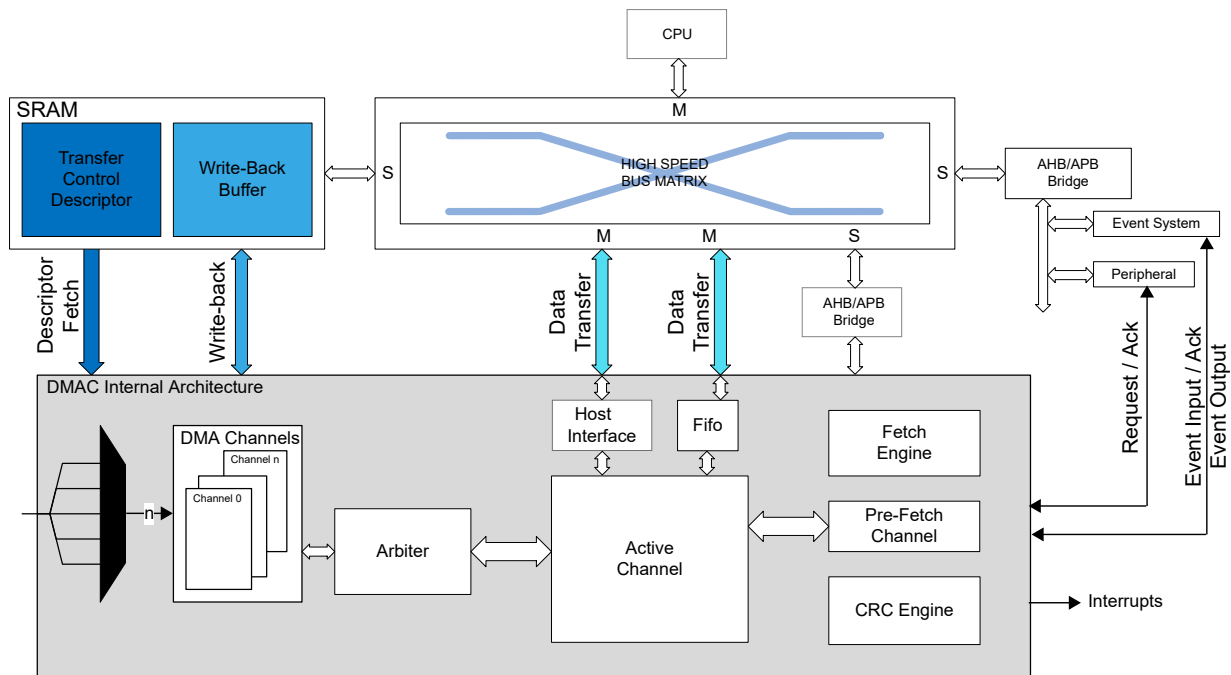
Figure 27-1. DMAC Block Diagram
