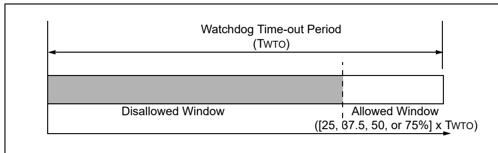
Figure 20-2. Programmable Windowed WDT
