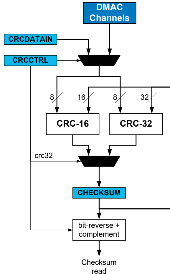
Figure 27-19. CRC Generator Block Diagram
