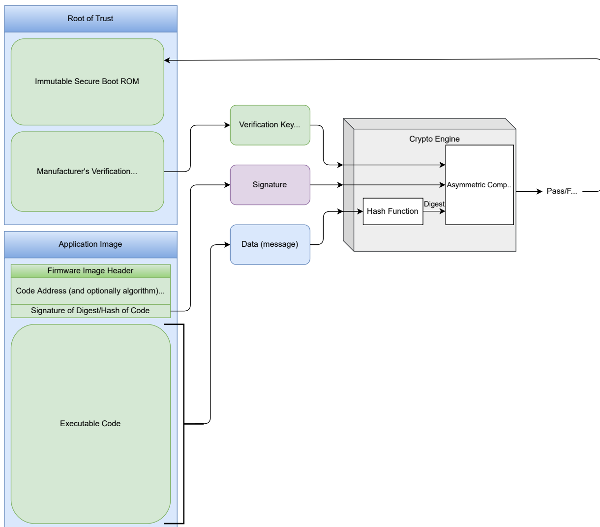
Figure 13-2. Secure Boot Firmware Validation
