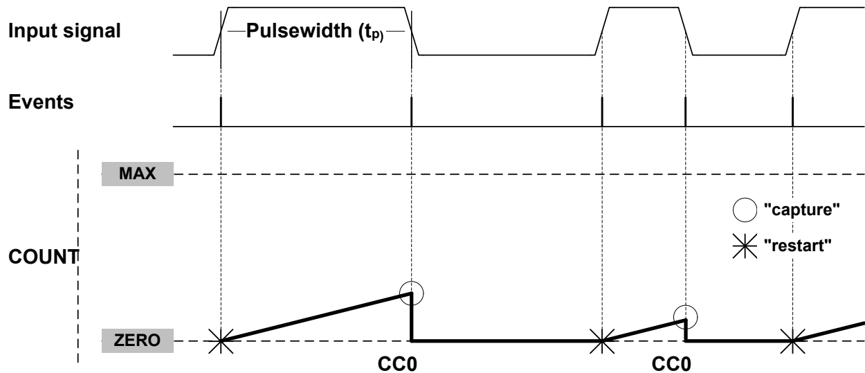
Figure 41-14. Pulse-Width Capture on Channel 0
