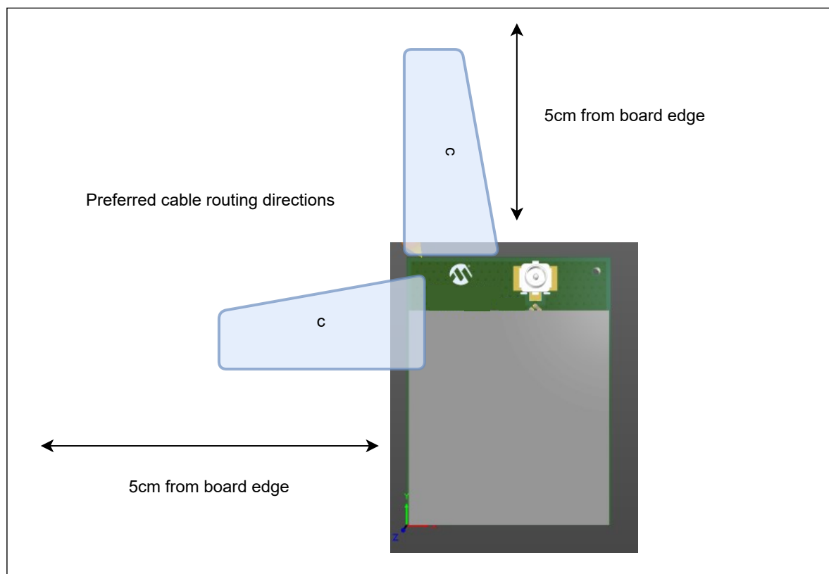
Figure 5-6. PIC32WM-BZ6 Antenna Placement Guidelines
