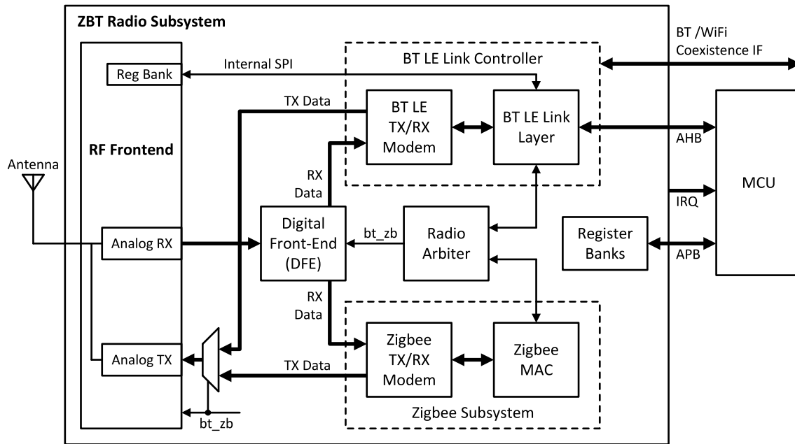
Figure 48-1. Wireless Subsystem Top Level Diagram
