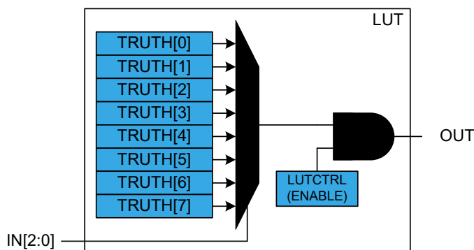
Figure 29-2. Truth Table Output Value Selection
