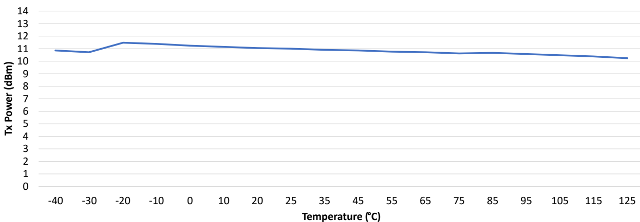
Figure 49-35. Bluetooth Low Energy Transmit Power vs. Temperature
