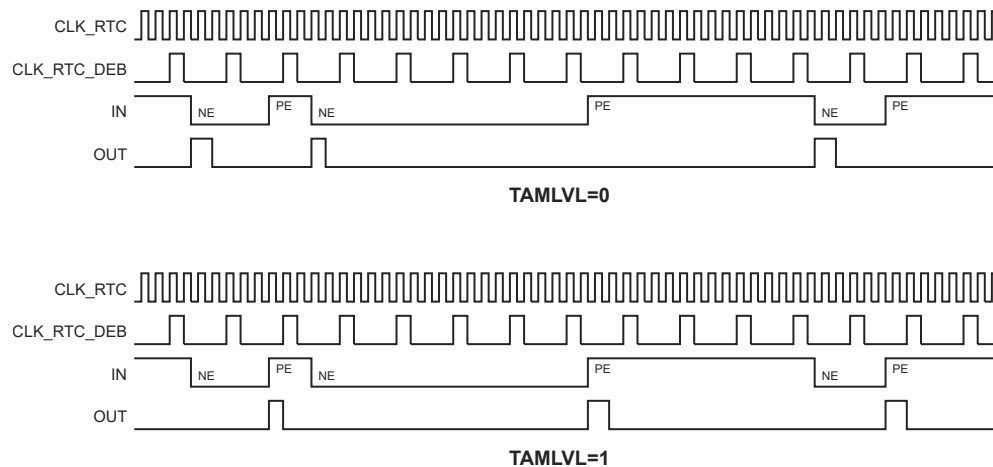
Figure 26-6. Edge Detection with Debouncer Disabled
