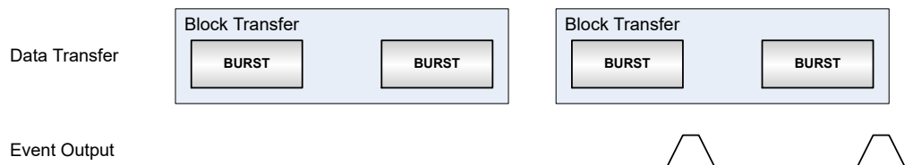
Figure 27-17. Burst Event Output Generation
