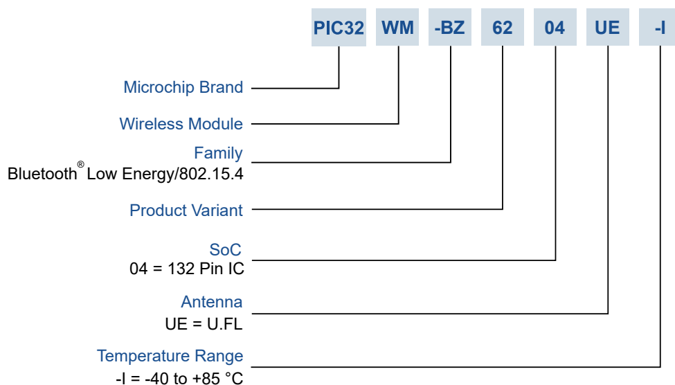
Figure 2-2. PIC32WM-BZ6 Module Ordering Information
