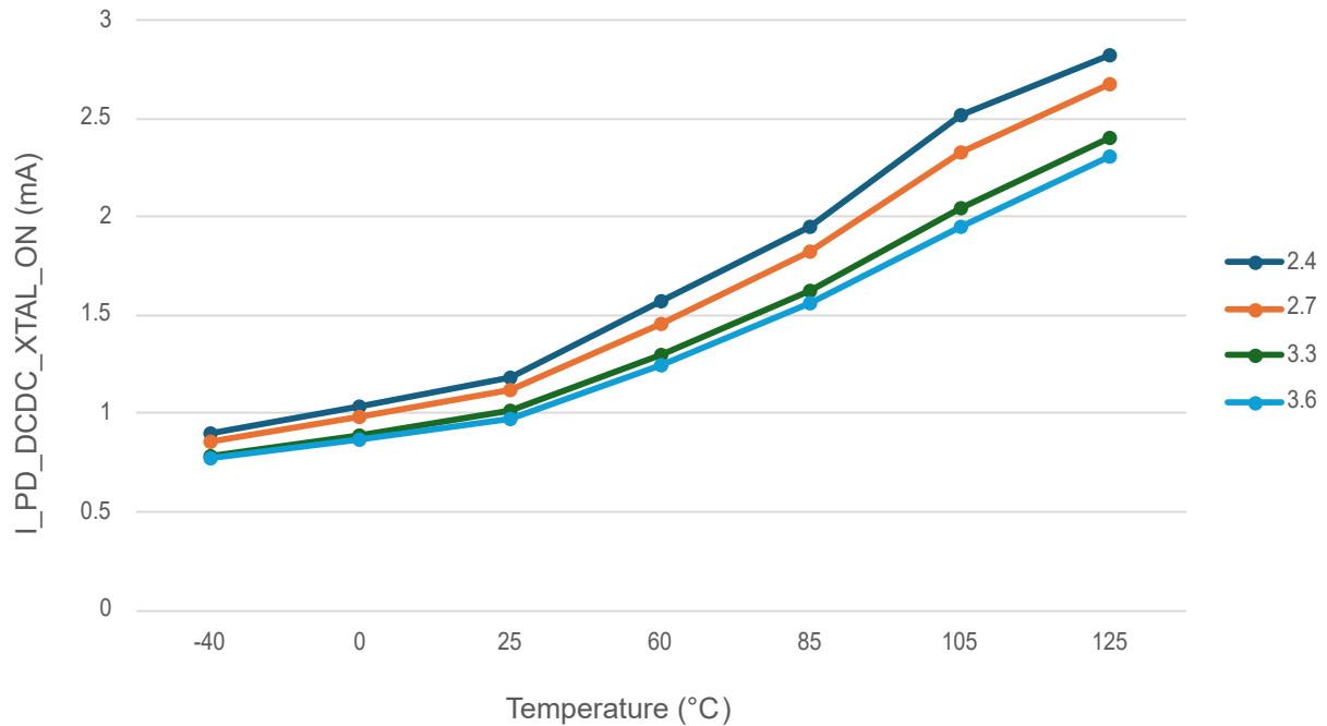
Figure 49-12. Sleep Current with BUCK_XTAL_ON
