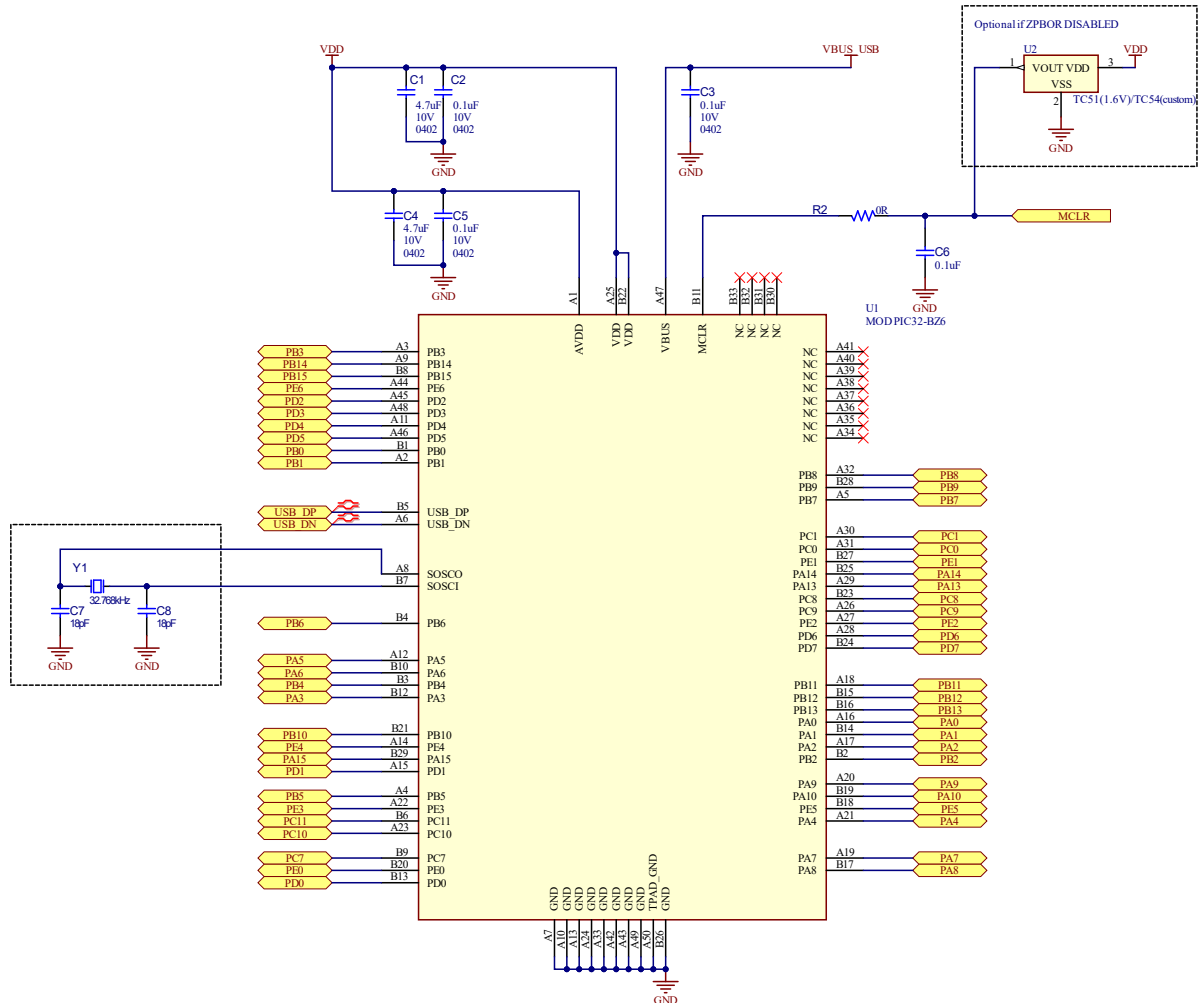
Figure 5-2. Module Basic Connection and Interface Diagram for PIC32WM-BZ6204 Module
