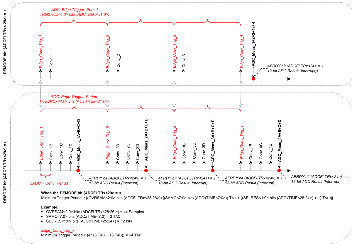
Figure 37-10. ADC Filter Comparisons Example
