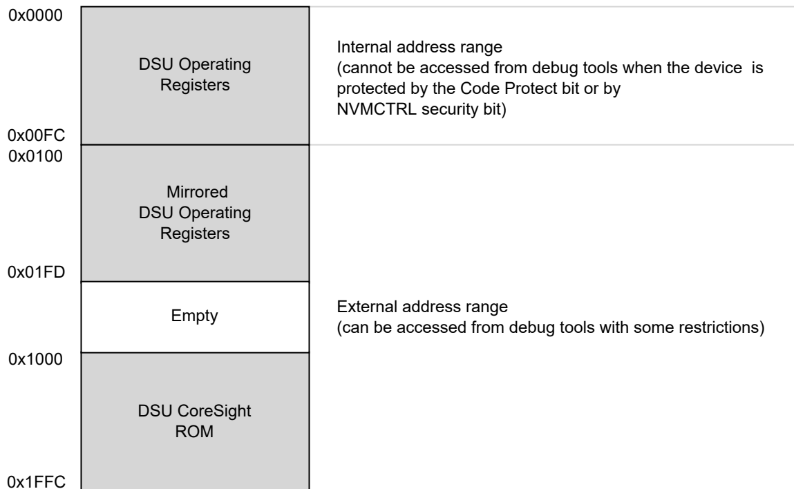
Figure 17-4. APB Memory Mapping
