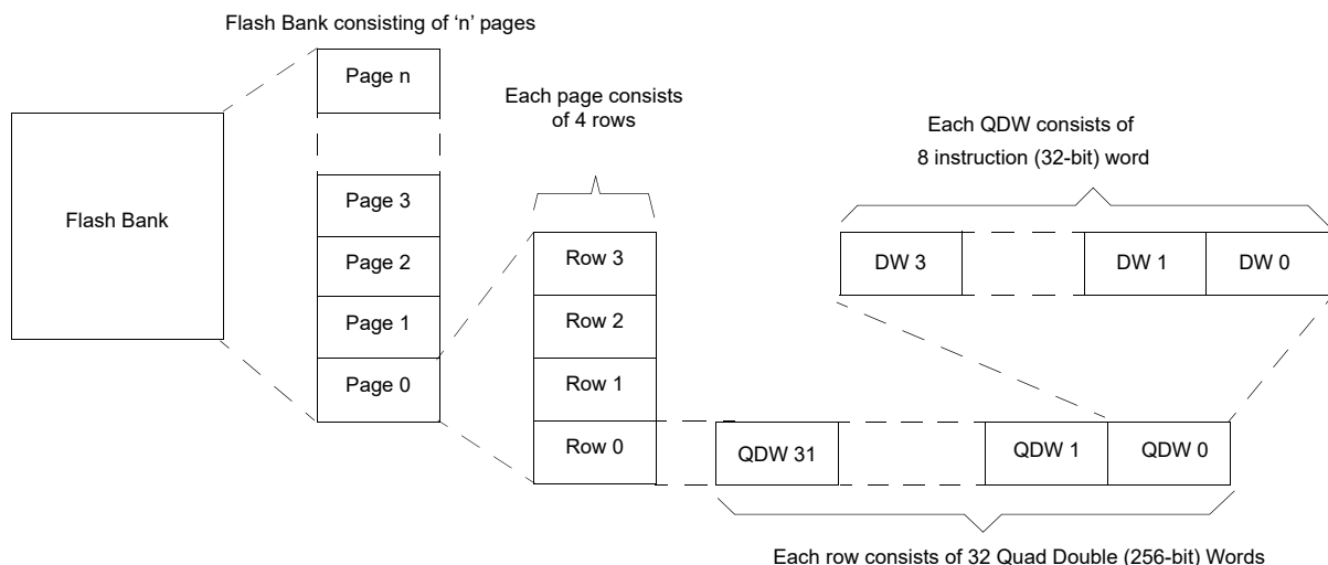
Figure 16-2. Flash Construction
