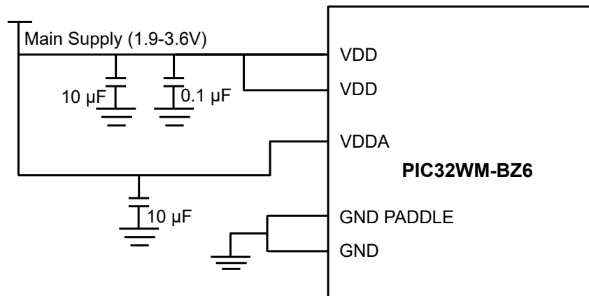
Figure 8-3. PIC32WM-BZ6 Module Schematics with VDD and Optional Bulk Capacitors
