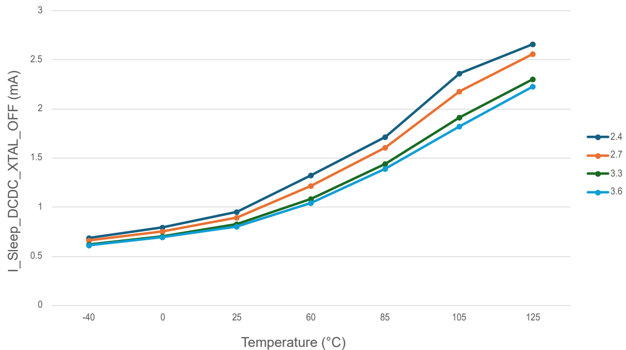
Figure 49-11. Sleep Current with BUCK_XTAL_OFF
