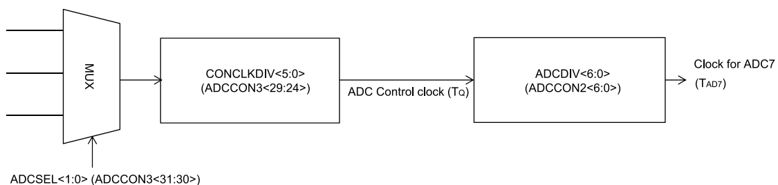
Figure 37-7. Clock Derivation for Shared ADC Cores
