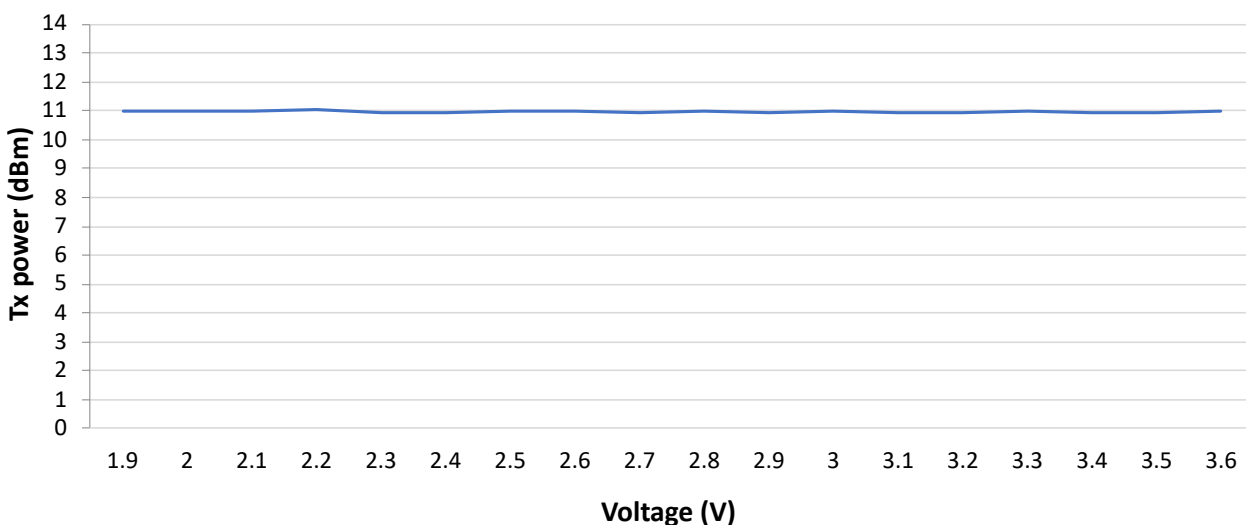
Figure 49-36. Bluetooth Low Energy Transmit Power vs. VDD Supply Voltage
