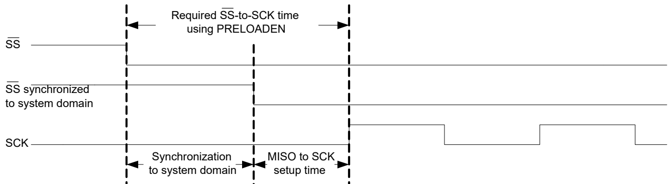
Figure 34-4. Timing Using Preloading
