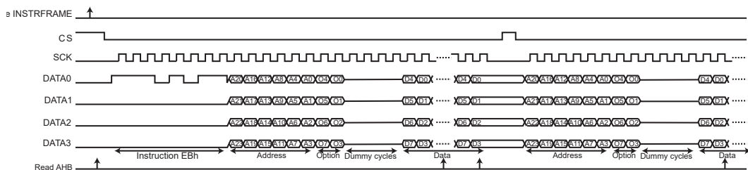
Figure 36-18. Instruction Transmission Waveform 7
