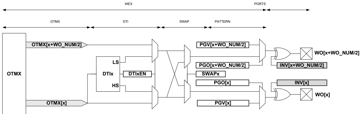
Figure 42-34. Waveform Extension Stage Details
