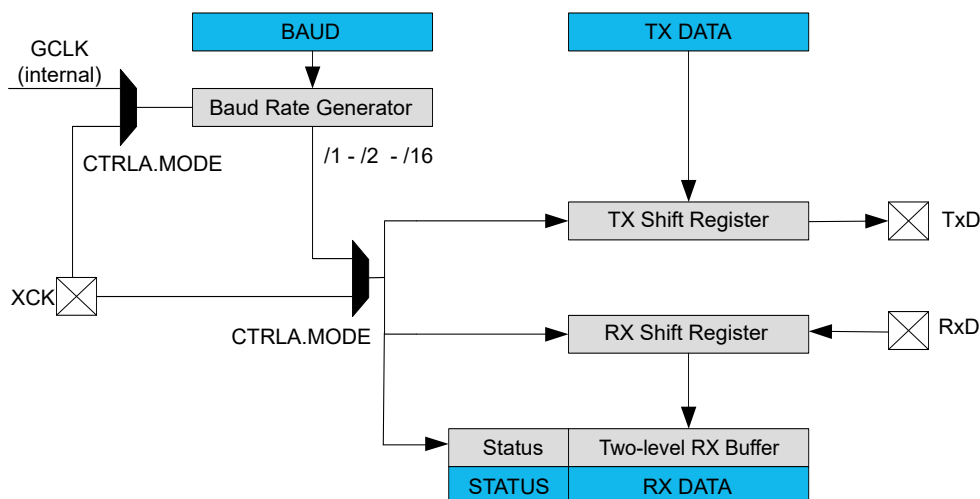
Figure 33-1. USART Block Diagram
