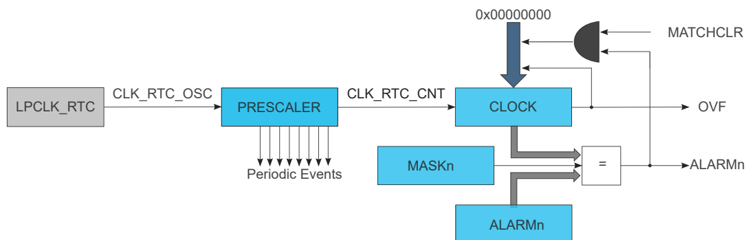
Figure 26-3. RTCC Block Diagram (Mode 2 — Clock/Calendar)
