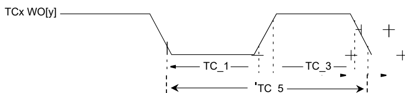
Figure 49-27. TCx Timer Capture Input Module AC Timing Diagram
