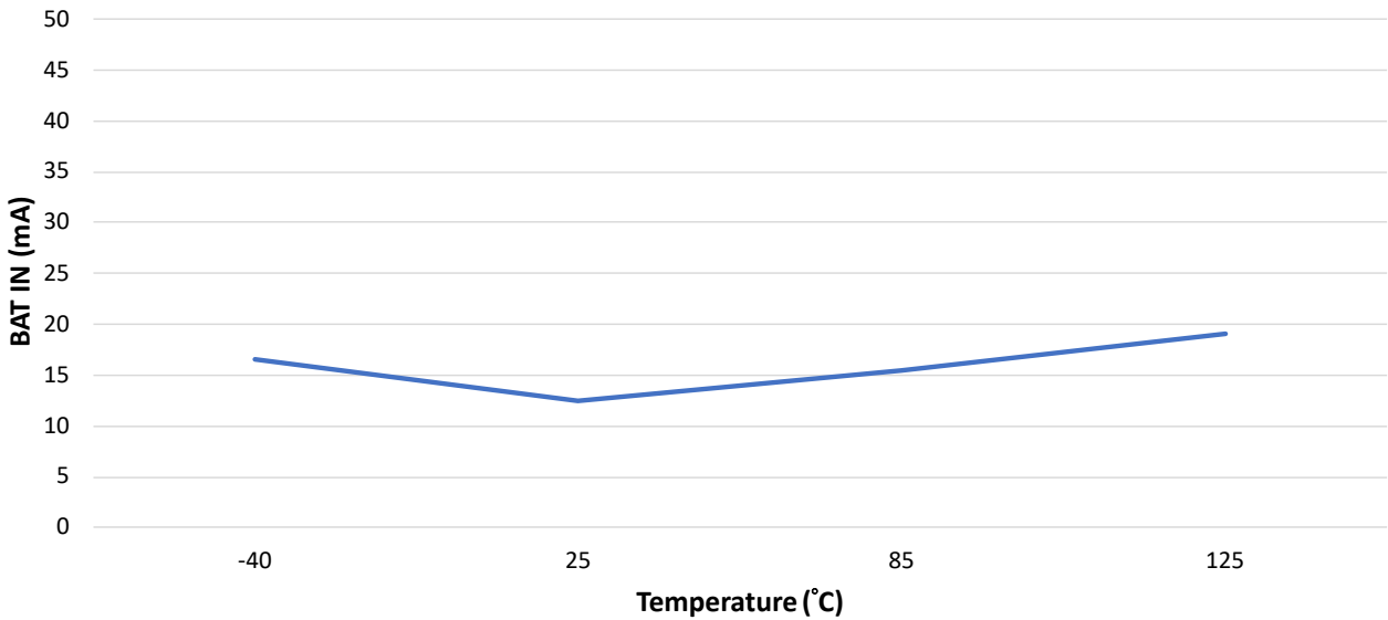
Figure 49-55. IEEE® 802.15.4 Receive Current vs. Temperature
