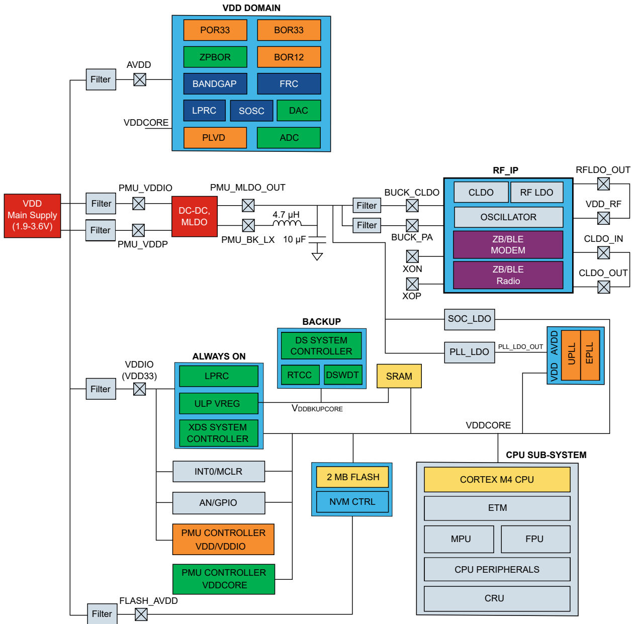
Figure 8-1. Power Subsystem Block Diagram
