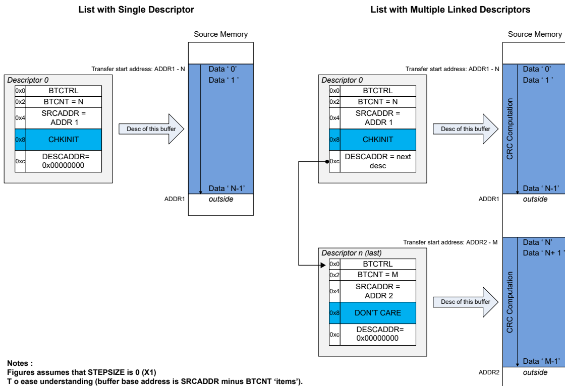
Figure 27-20. CRC Computation with Single Linked Transfers
