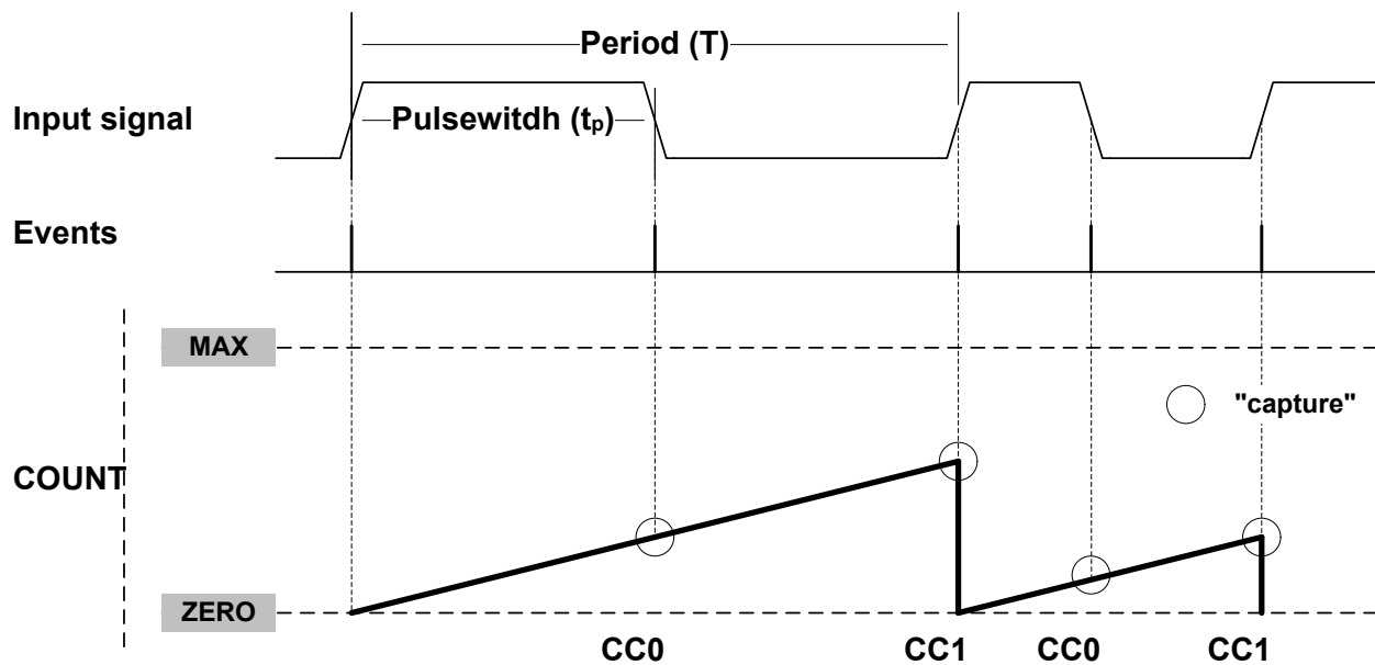
Figure 41-13. PWP Capture
