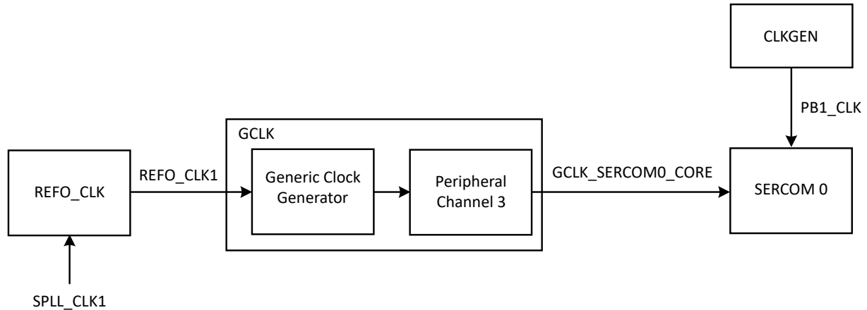
Figure 18-7. Example of SERCOM0 Clock
