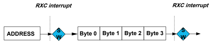
Figure 34-10. 32-Bit Extension Client Operation
