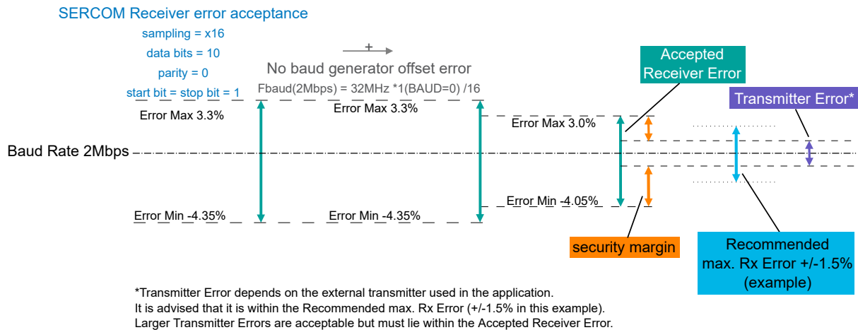
Figure 33-6. USART RX Error Calculation Example
