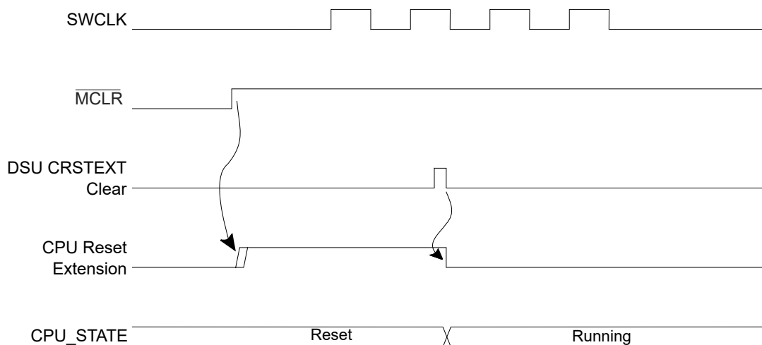
Figure 17-2. Typical CPU Reset Extension Set and Clear Timing Diagram
