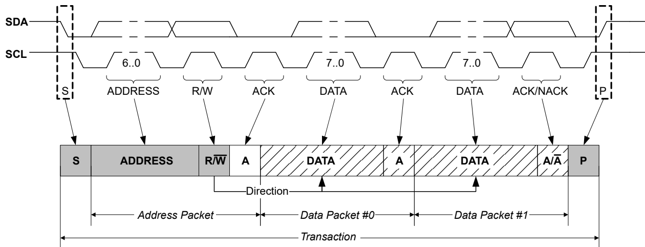
Figure 35-3. Basic I 2 C Transaction Diagram
