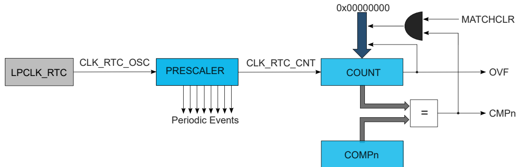
Figure 26-1. RTCC Block Diagram (Mode 0 — 32-Bit Counter)
