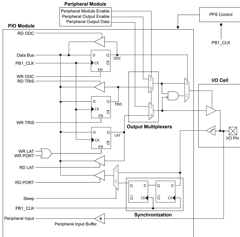
Figure 7-1. Typical Multiplexed Port Structure Block Diagram
