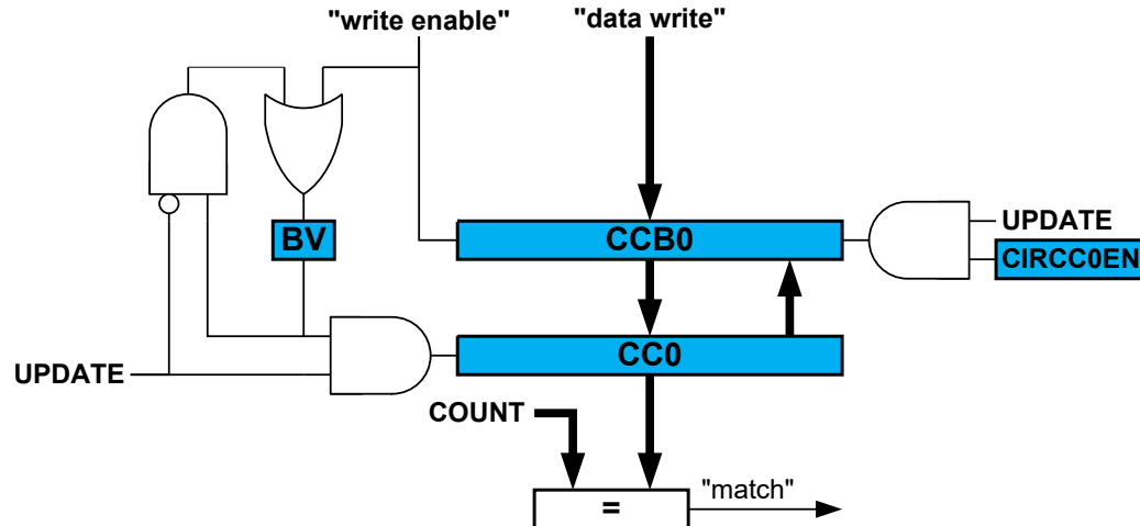
Figure 42-17. Circular Buffer on Channel 0
