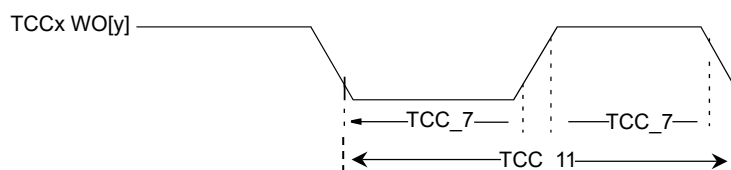
Figure 49-30. TCCx Timer Capture Output Module AC Timing Diagram
