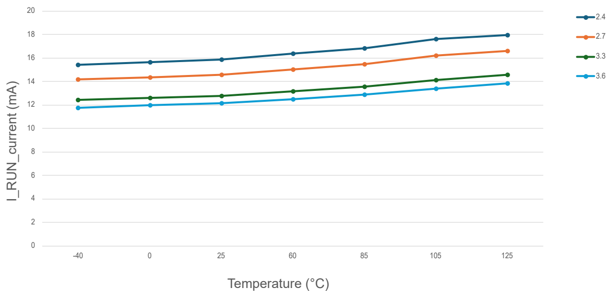
Figure 49-4. Run Mode Current Consumption in Buck Mode at FRC 8 MHz
