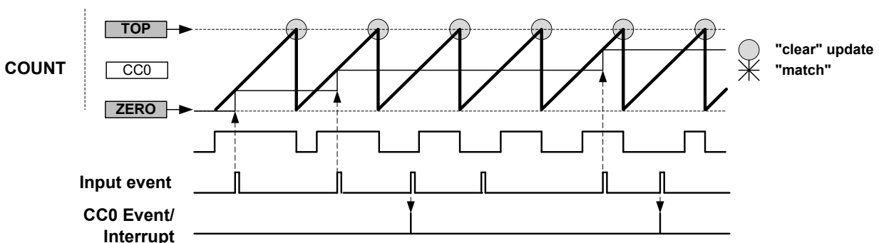
Figure 41-16. Maximum Capture Operation with CC0 Initialized with ZERO Value
