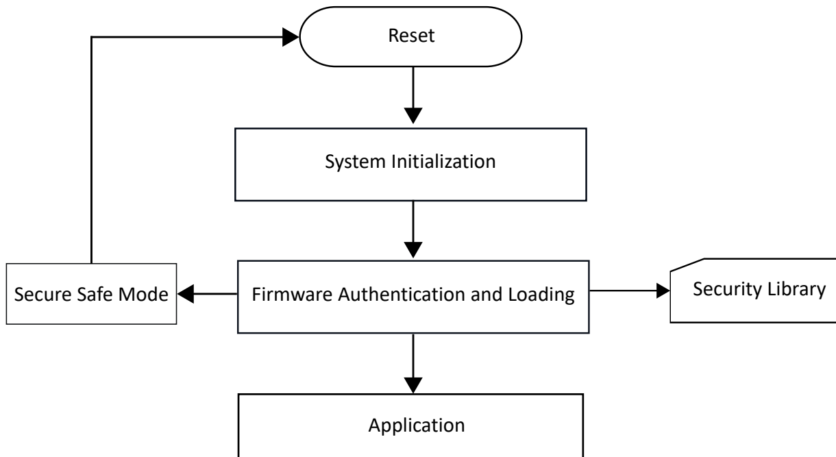
Figure 13-1. Boot ROM Flow
