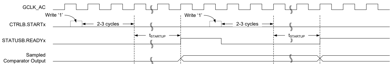
Figure 39-3. Single-Shot Example
