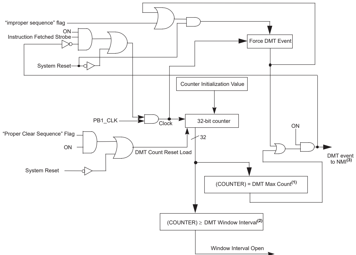
Figure 21-1. Deadman Timer Block Diagram
