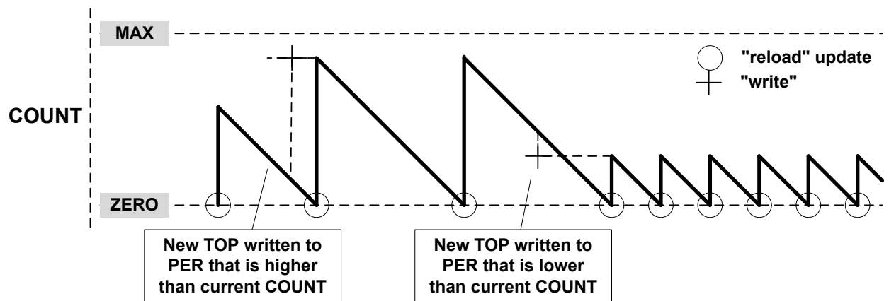
Figure 41-9. Unbuffered Single-Slope Down-Counting Operation
