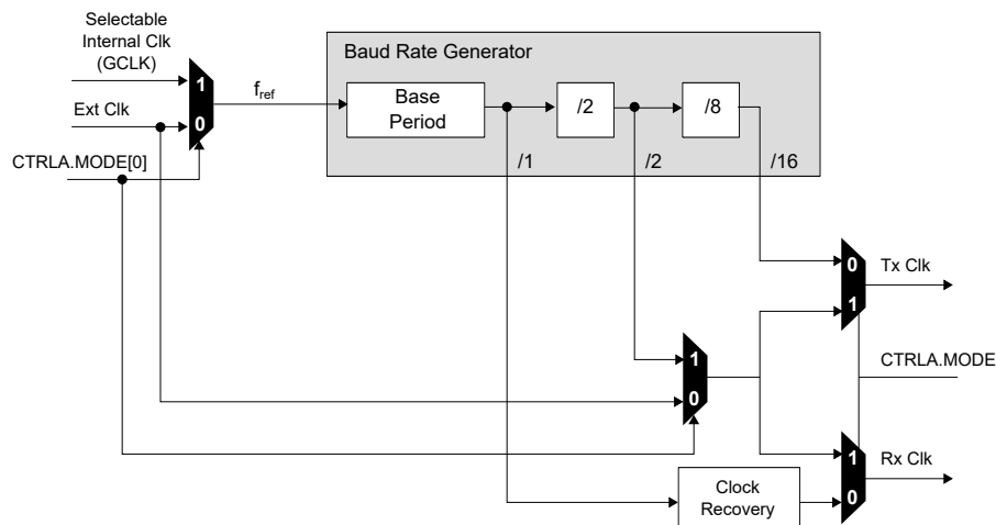
Figure 32-3. Baud Rate Generator
