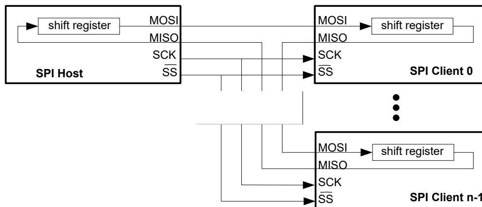
Figure 34-6. Multiple Clients in Series
