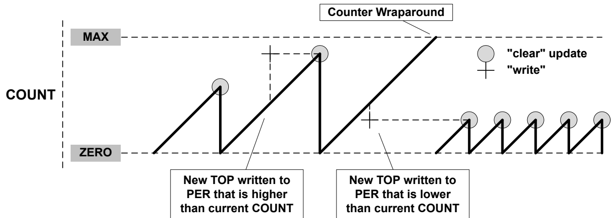
Figure 41-8. Unbuffered Single-Slope Up-Counting Operation
