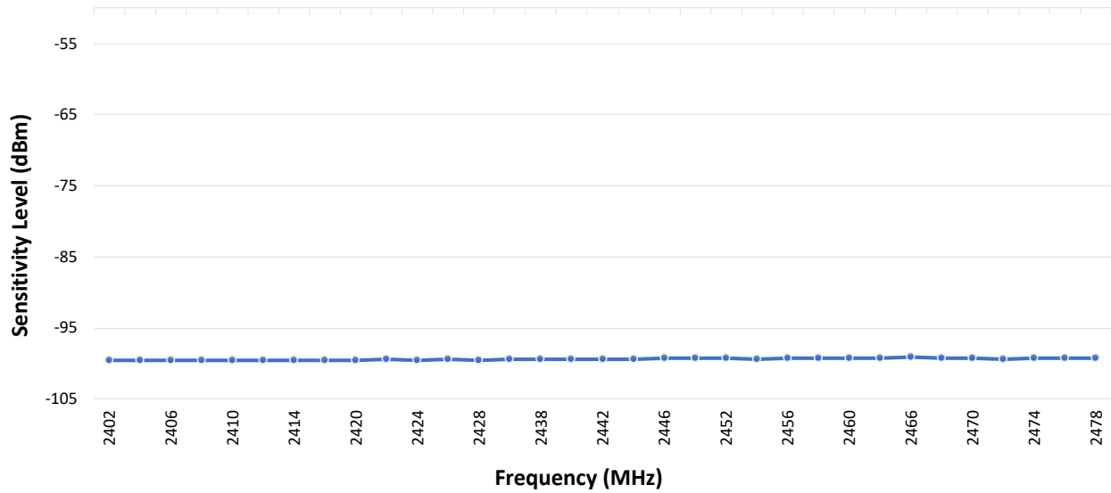
Figure 49-41. Bluetooth Low Energy Receive Sensitivity vs. Frequency
