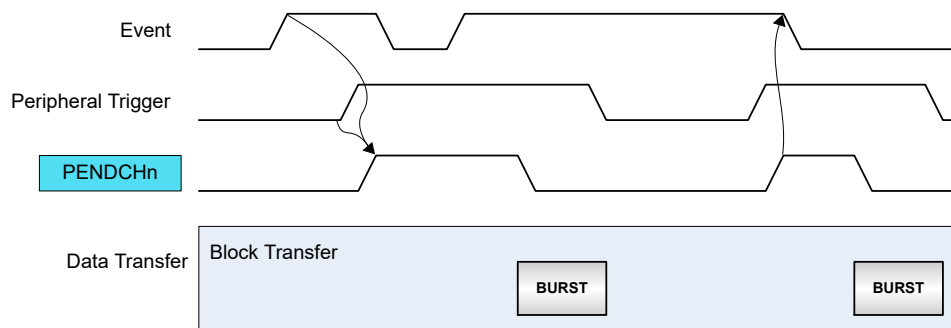
Figure 27-14. Conditional Event with Burst Peripheral Triggers
