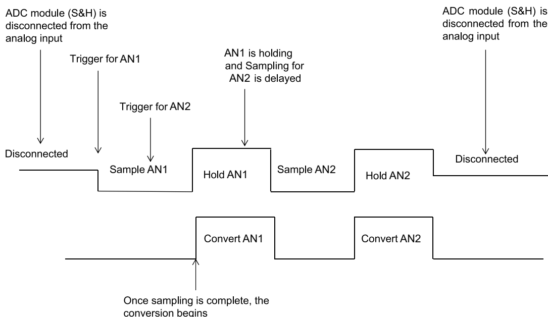
Figure 37-4. Multiple Independent Class 2 Trigger Conversion Sequence
