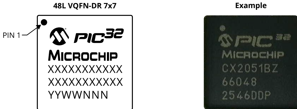
Figure 50-2. PIC32CX2051BZ66048 Package Marking
