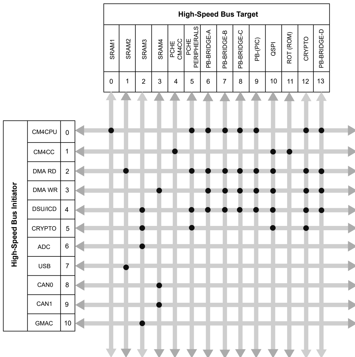
Figure 10-1. High-Speed Bus Matrix Inter-connectivity
