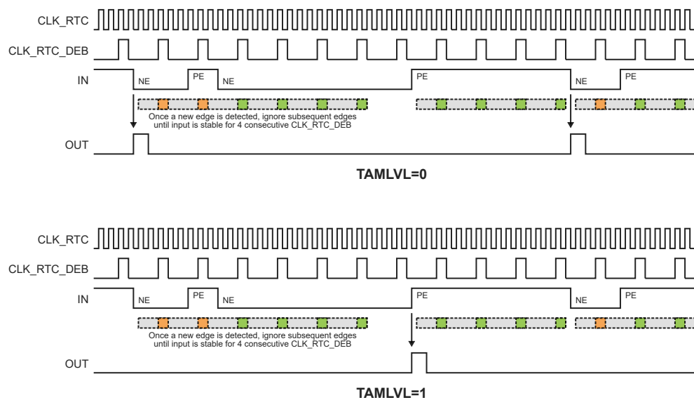
Figure 26-8. Edge Detection with Asynchronous Stability Debouncing
