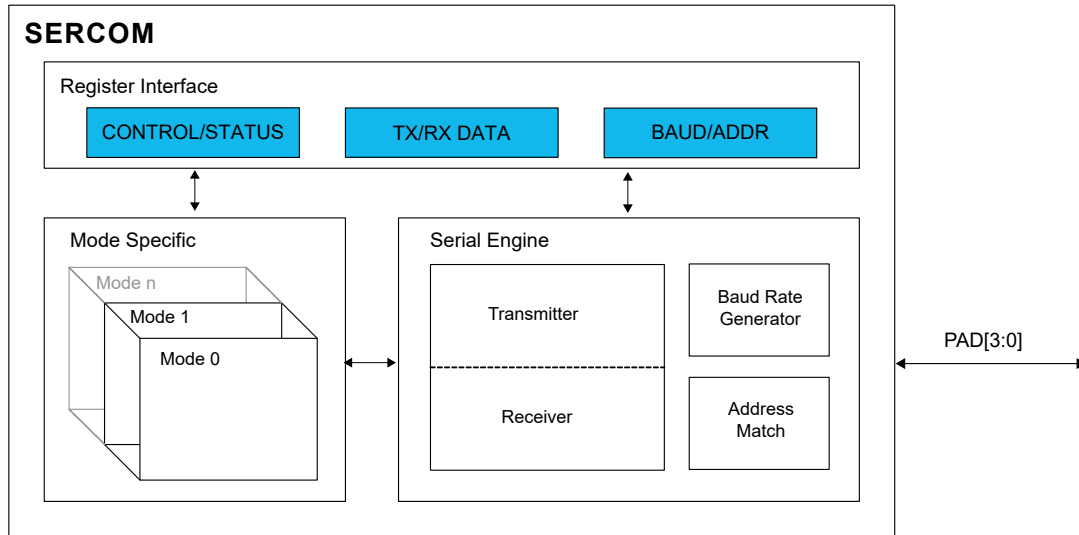
Figure 32-1. SERCOM Block Diagram
