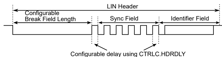
Figure 33-14. LIN Header Generation
