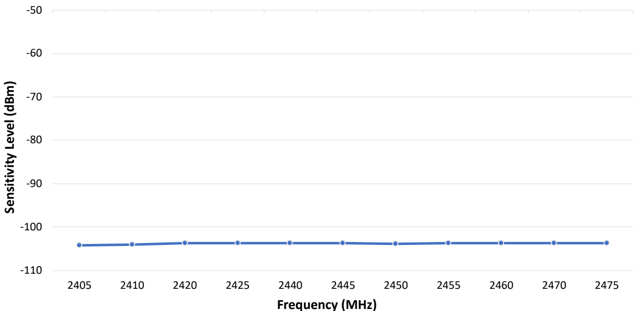
Figure 49-54. IEEE® 802.15.4 Receive Sensitivity vs. Frequency
