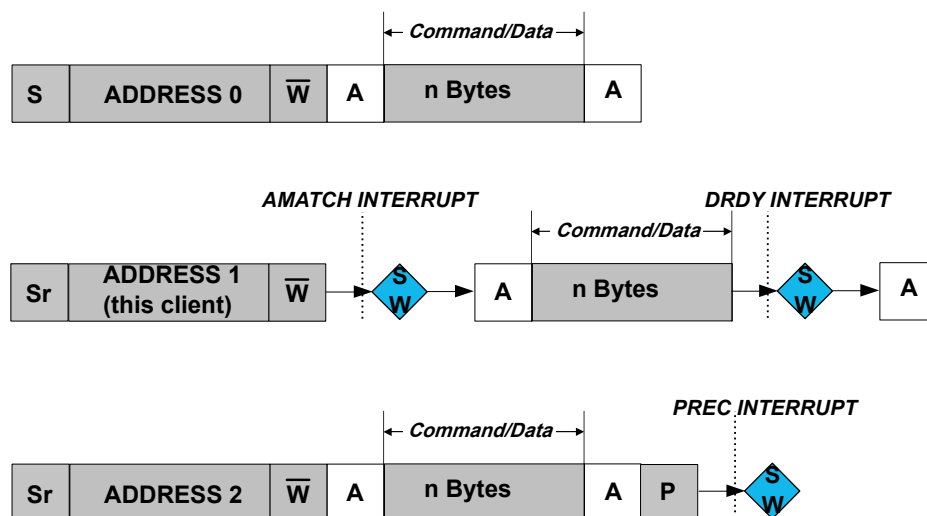
Figure 35-10. PMBus Group Command Example
