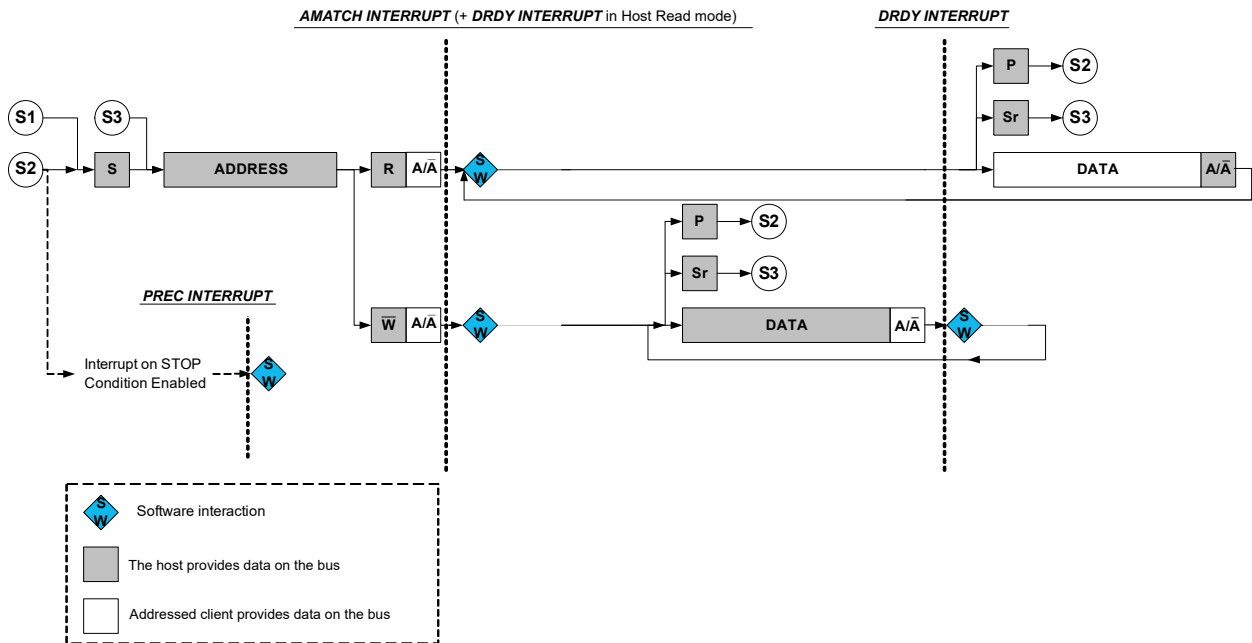
Figure 35-9. I 2 C Client Behavioral Diagram (SCLSM = 1)
