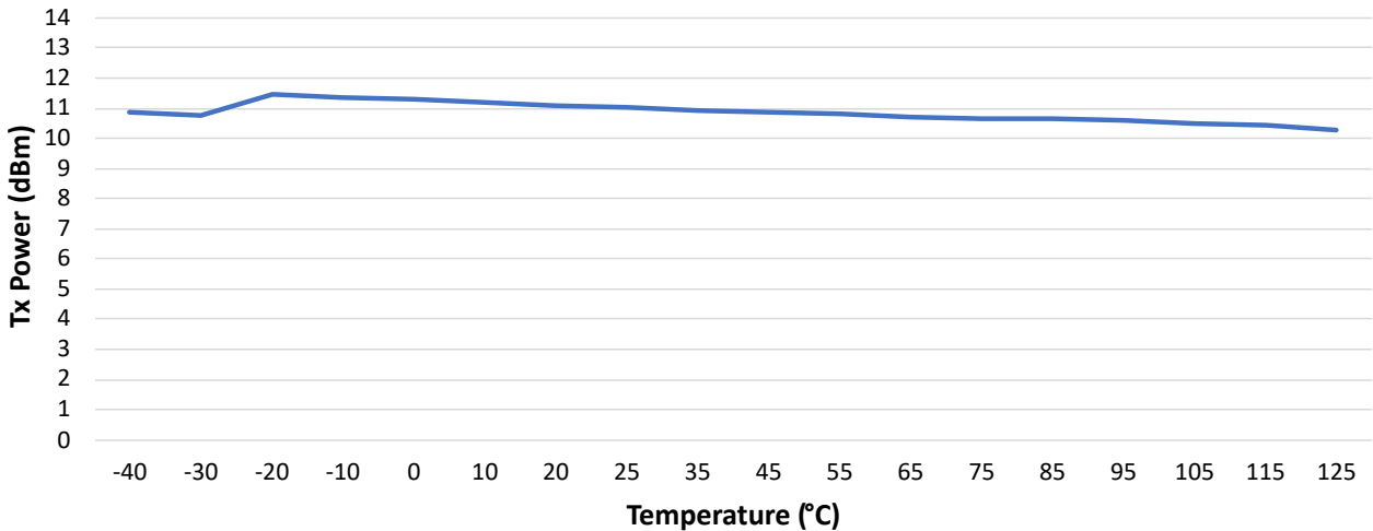
Figure 49-47. IEEE® 802.15.4 Transmit Power vs. Temperature
