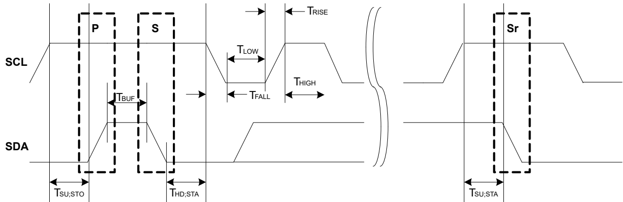
Figure 35-7. SCL Timing
