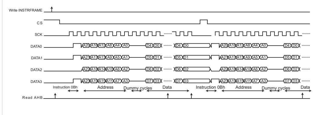
Figure 36-19. Instruction Transmission Waveform 8
