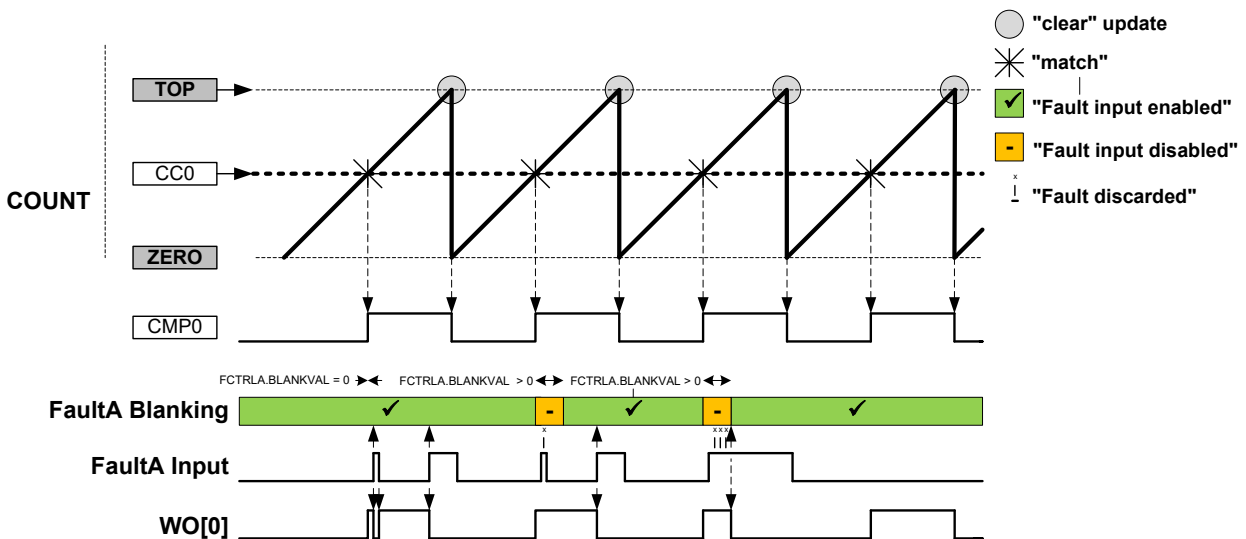
Figure 42-22. Fault Blanking in RAMP1 Operation with Inverted Polarity
