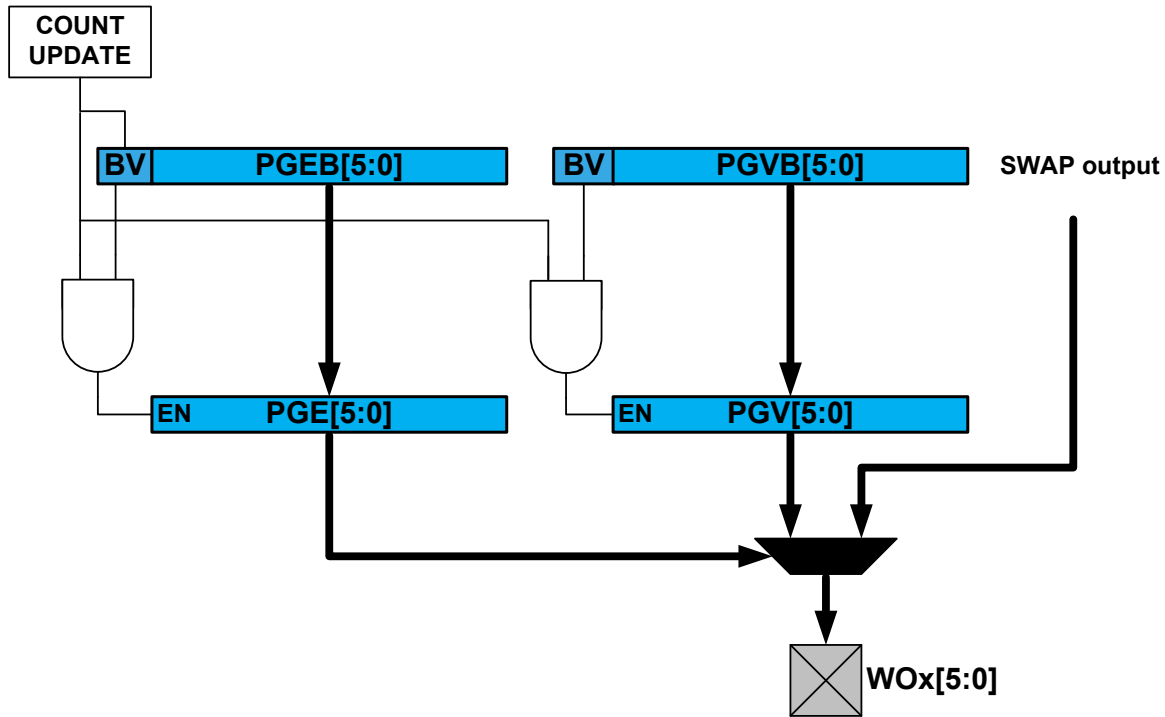
Figure 42-37. Pattern Generator Block Diagram
