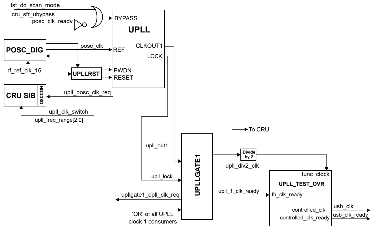
Figure 18-4. USB PLL Subsystem
