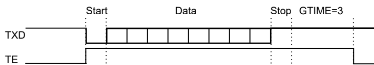
Figure 33-16. Example of TE Drive with Guard Time
