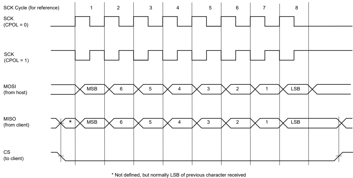
Figure 36-4. QSPI Transfer Modes (BAUD.CPHA = 1, 8-bit transfer)
