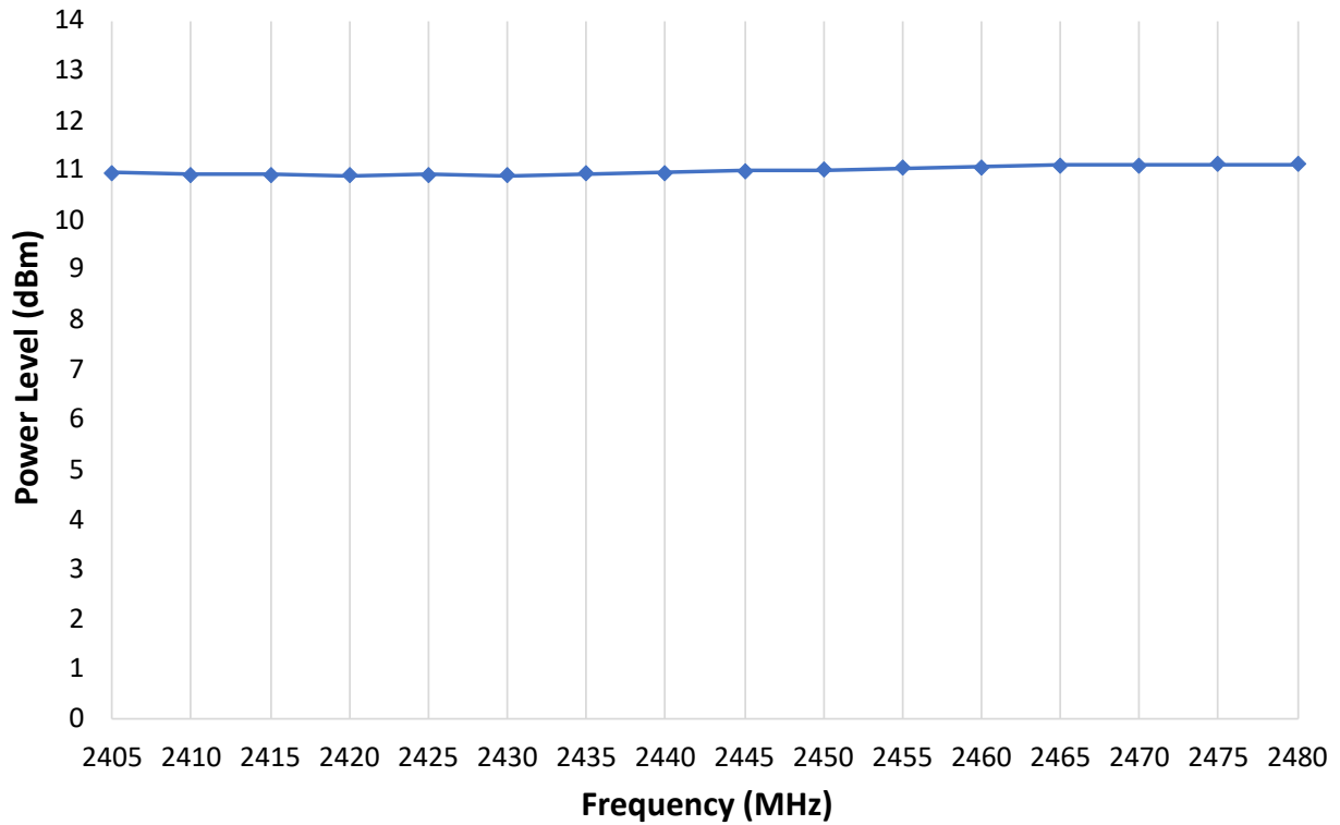
Figure 49-49. IEEE® 802.15.4 Transmit Power vs. Frequency
