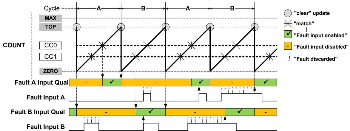
Figure 42-24. Fault Qualification in RAMP2 Operation with Inverted Polarity
