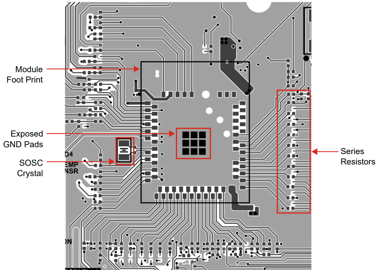
Figure 5-5. Example of Host Board on Top Layer
