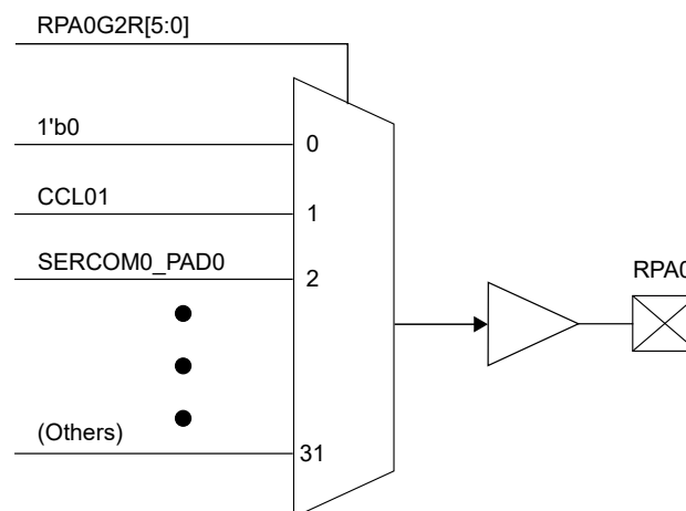
Figure 7-3. Example Multiplexing of Remappable Output Signal for RPA0 (Map Output Function to Pin)
