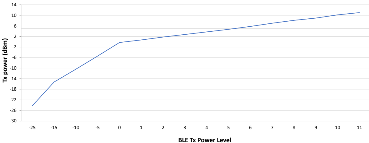
Figure 49-38. Bluetooth Low Energy Transmit Power vs. Power Level
