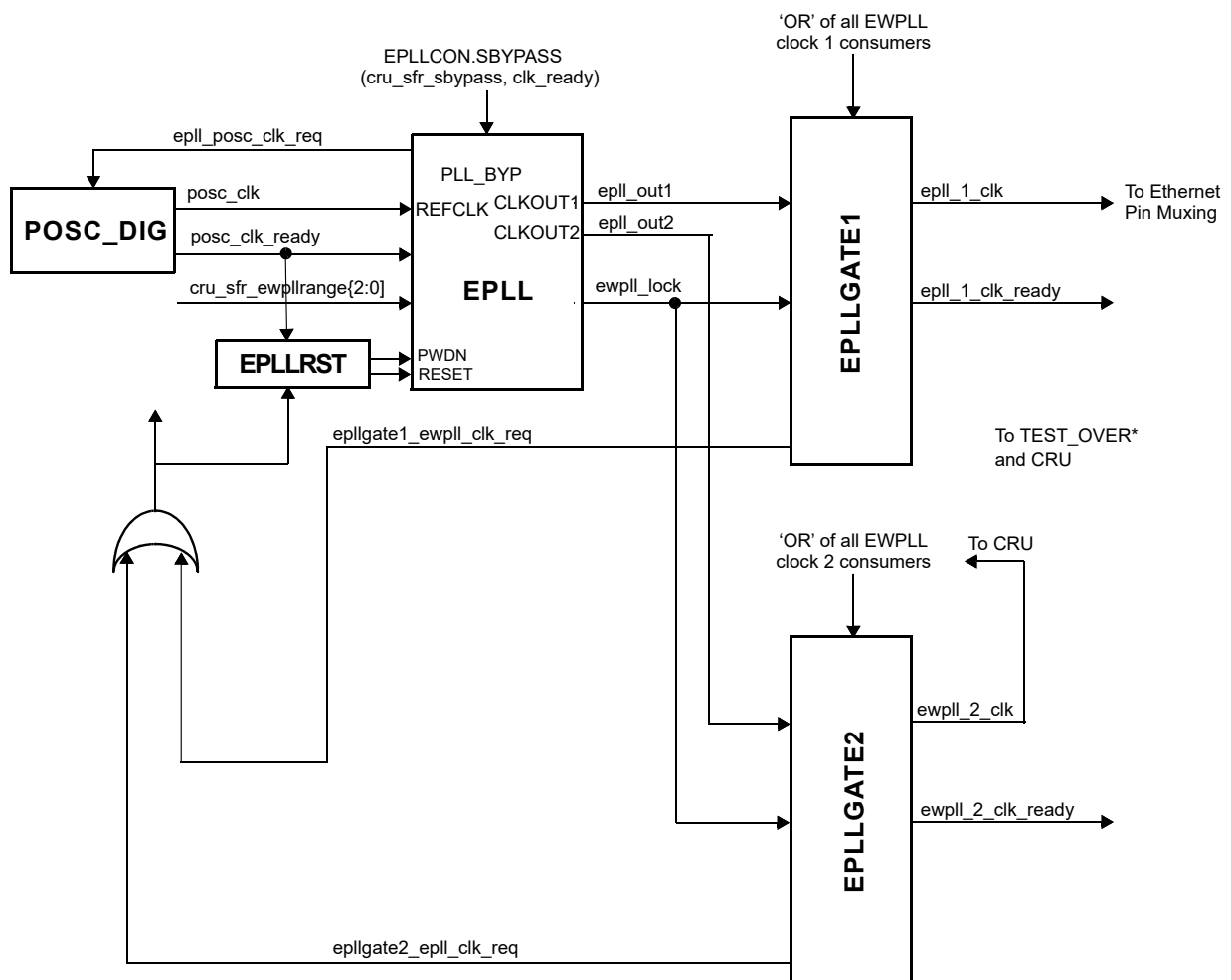
Figure 18-3. Ethernet PLL Subsystem
