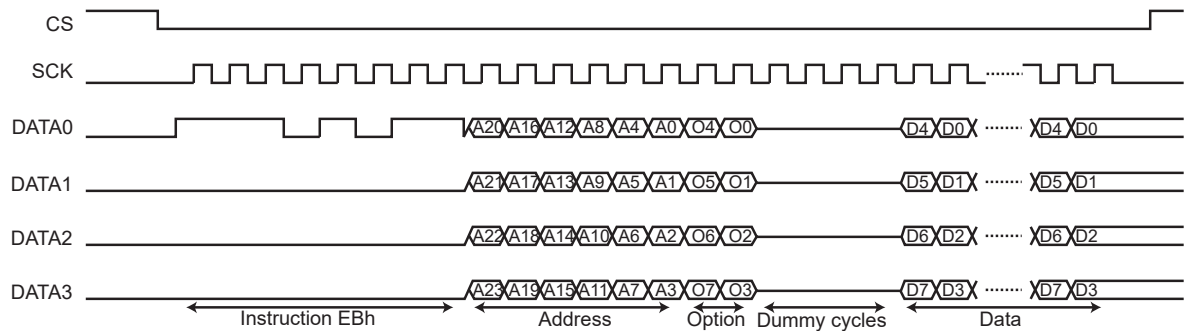
Figure 36-9. Instruction Frame
