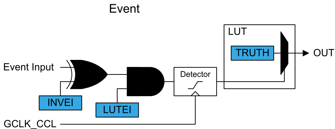
Figure 29-6. Event Input Selection
