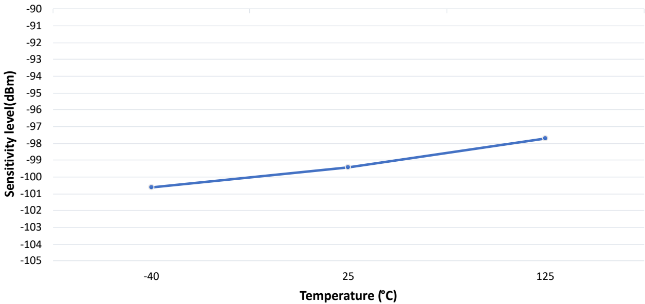
Figure 49-53. IEEE® 802.15.4 Receive Sensitivity vs. Temperature
