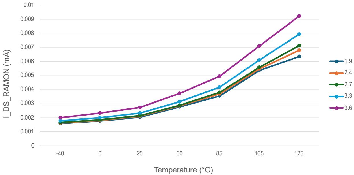
Figure 49-14. Deep Sleep Current RAM ON
