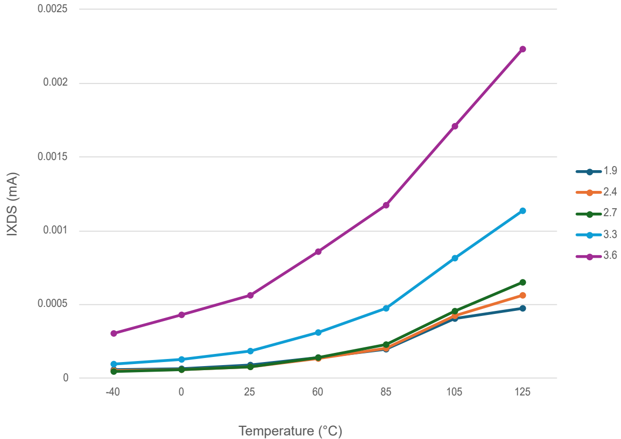
Figure 49-15. Extreme Deep Sleep Current
