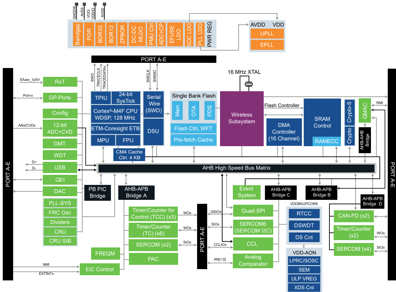
Figure 4-1. PIC32CX2051BZ62132 SoC Block Diagram
