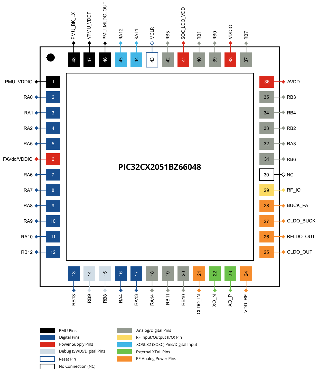
Figure 4-3. PIC32CX2051BZ66048 Pinout Diagram
