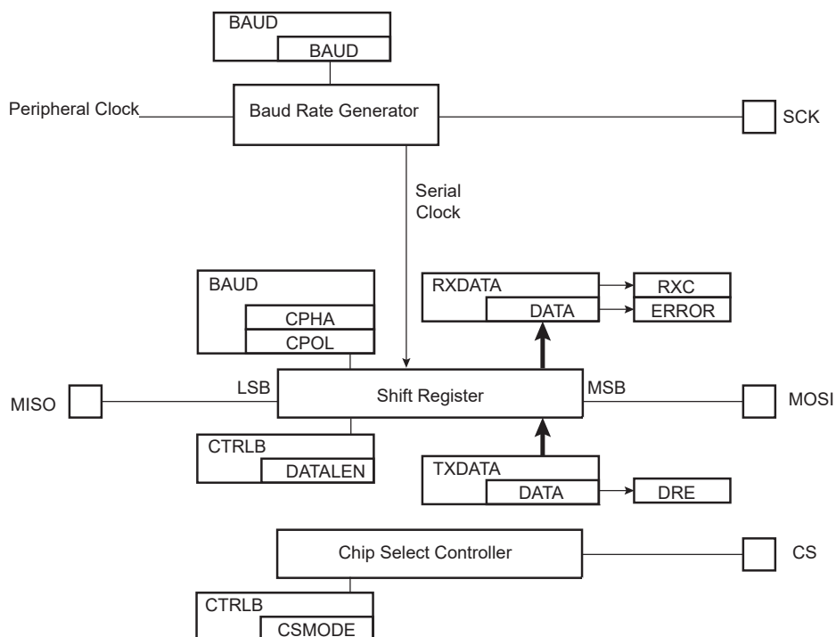
Figure 36-6. SPI Mode Block Diagram
