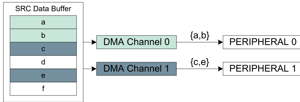
Figure 27-8. Source Address Increment
