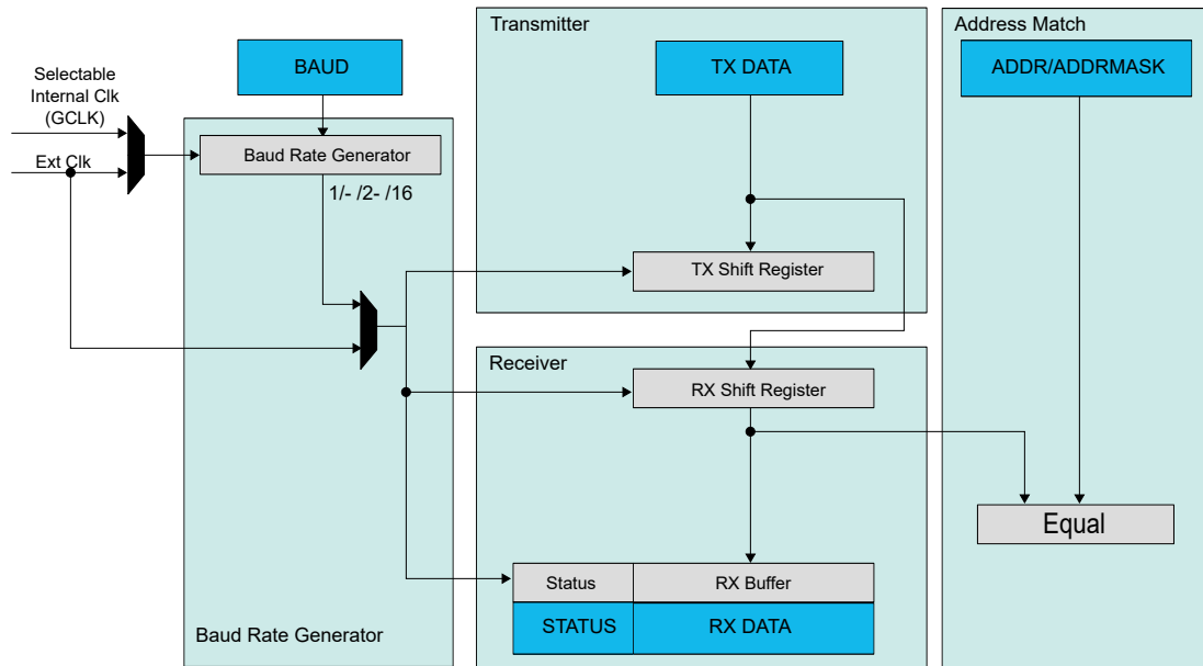
Figure 32-2. SERCOM Serial Engine
