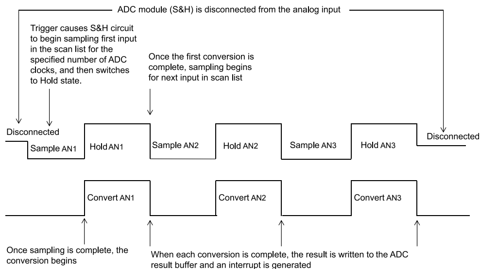
Figure 37-5. Input Scan Conversion Sequence for Three Class 2 Inputs
