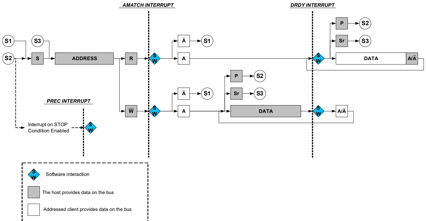
Figure 35-8. I 2 C Client Behavioral Diagram (SCLSM = 0)
