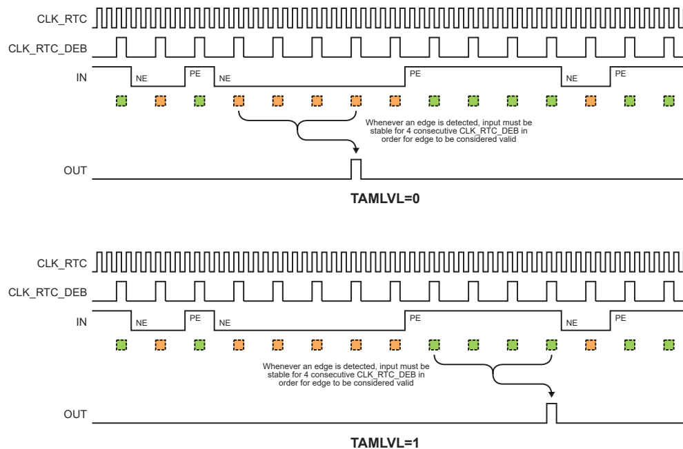
Figure 26-7. Edge Detection with Synchronous Stability Debouncing
