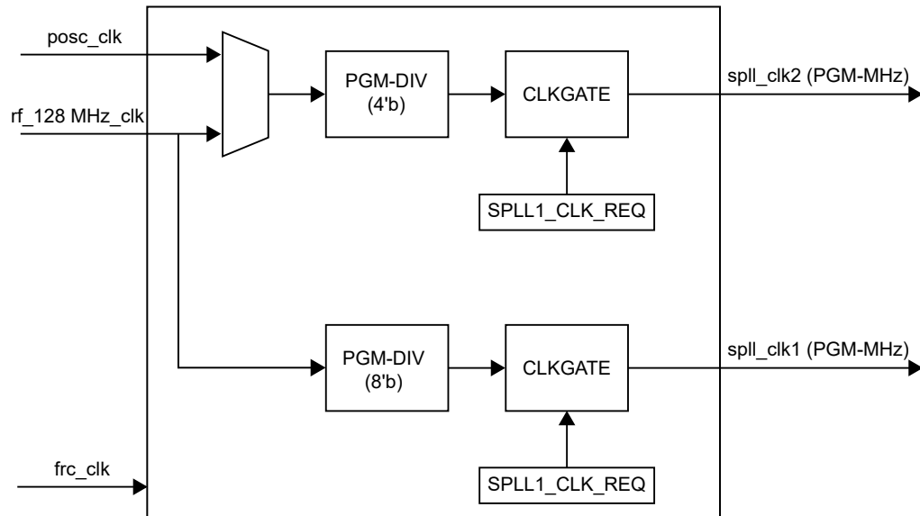
Figure 18-3. Ethernet PLL Subsystem
