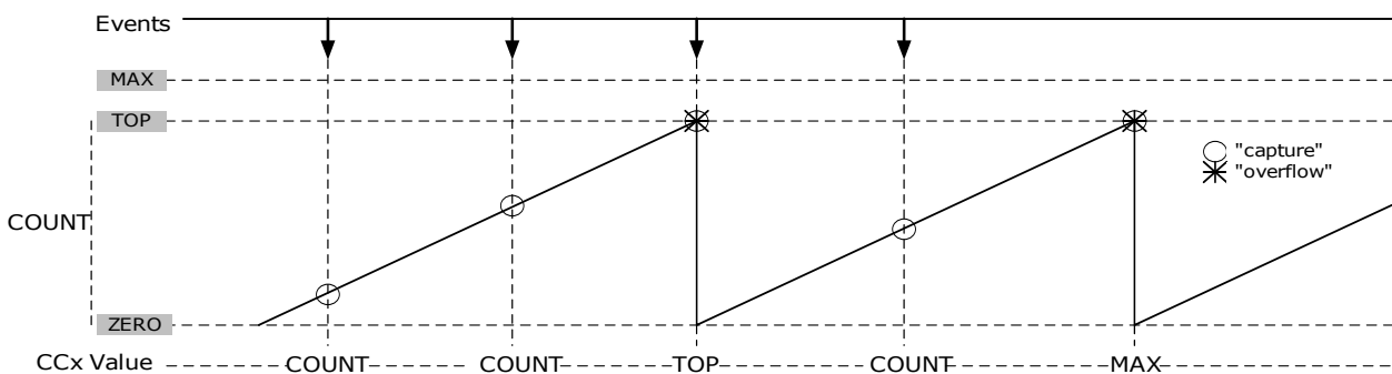
Figure 42-33. Time Stamp
