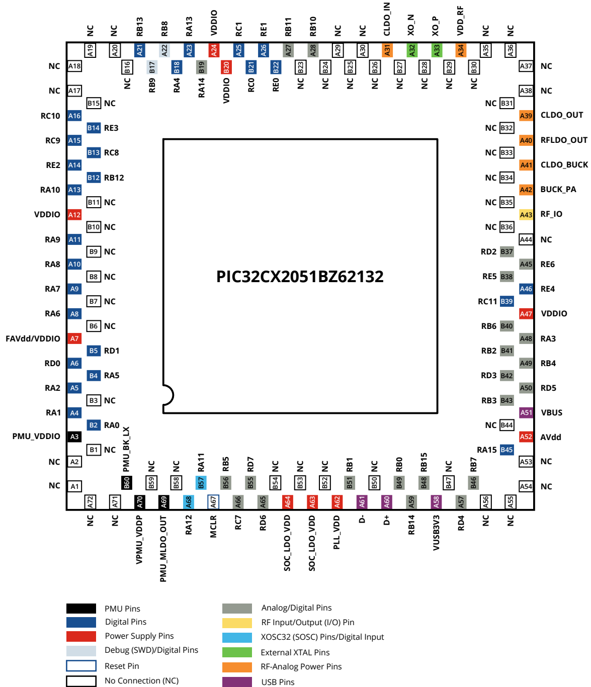
Figure 4-4. PIC32CX2051BZ62132 Pinout Diagram
