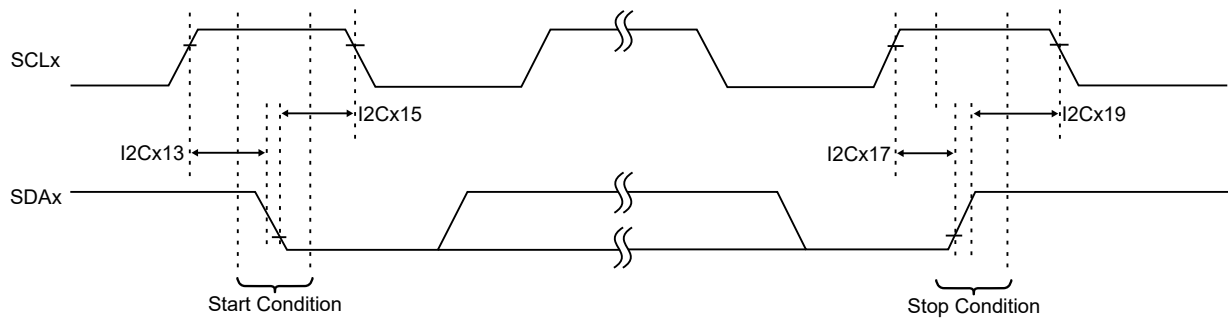
Figure 49-23. I 2 C Bus Data Host Mode AC Timing Diagram
