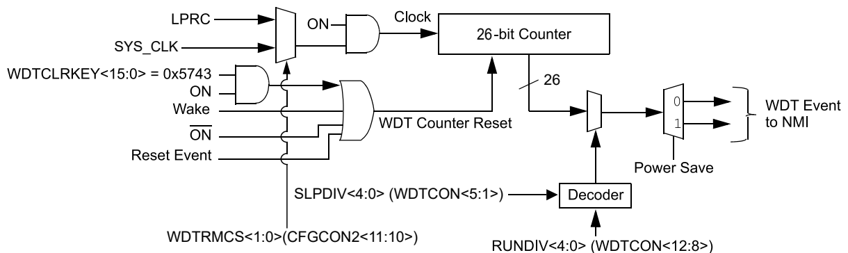
Figure 20-1. Block Diagram
