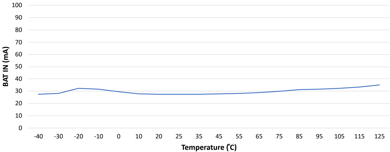
Figure 49-39. Bluetooth Low Energy Transmit Current vs. Temperature
