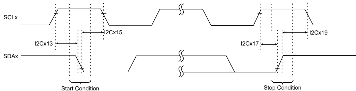
Figure 49-25. I 2 C Bus Data Client Mode AC Timing Diagram
