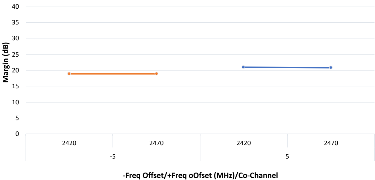
Figure 49-56. IEEE® 802.15.4 ACR 5M Margin
