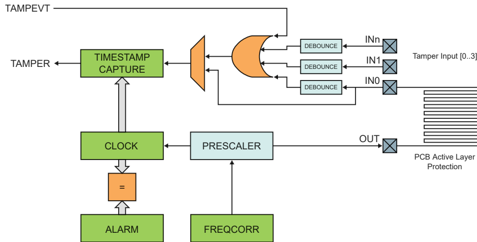
Figure 26-4. RTCC Block Diagram (Tamper Detection)
