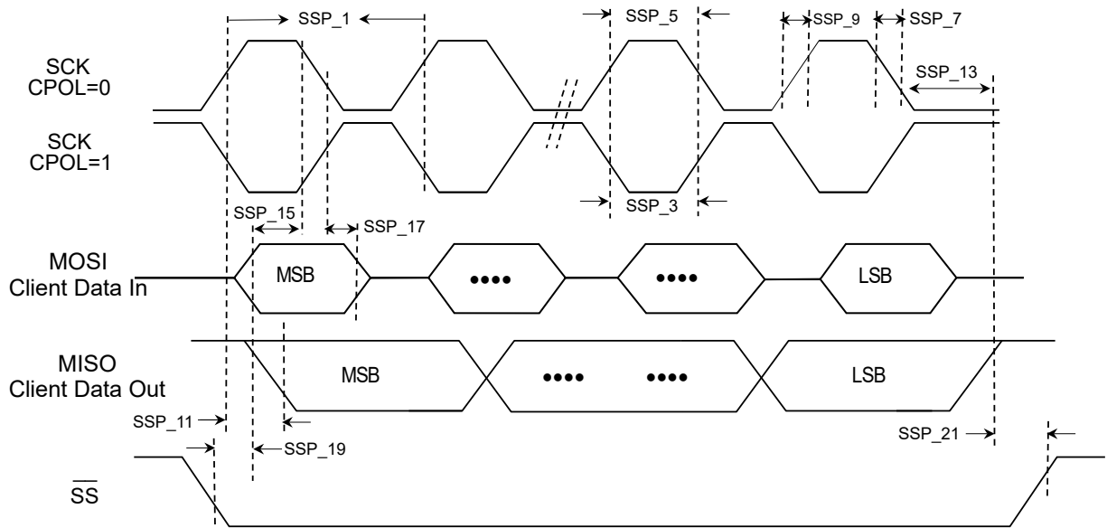
Figure 49-21. SPI Client Module CPHA = 1 Timing Diagrams
