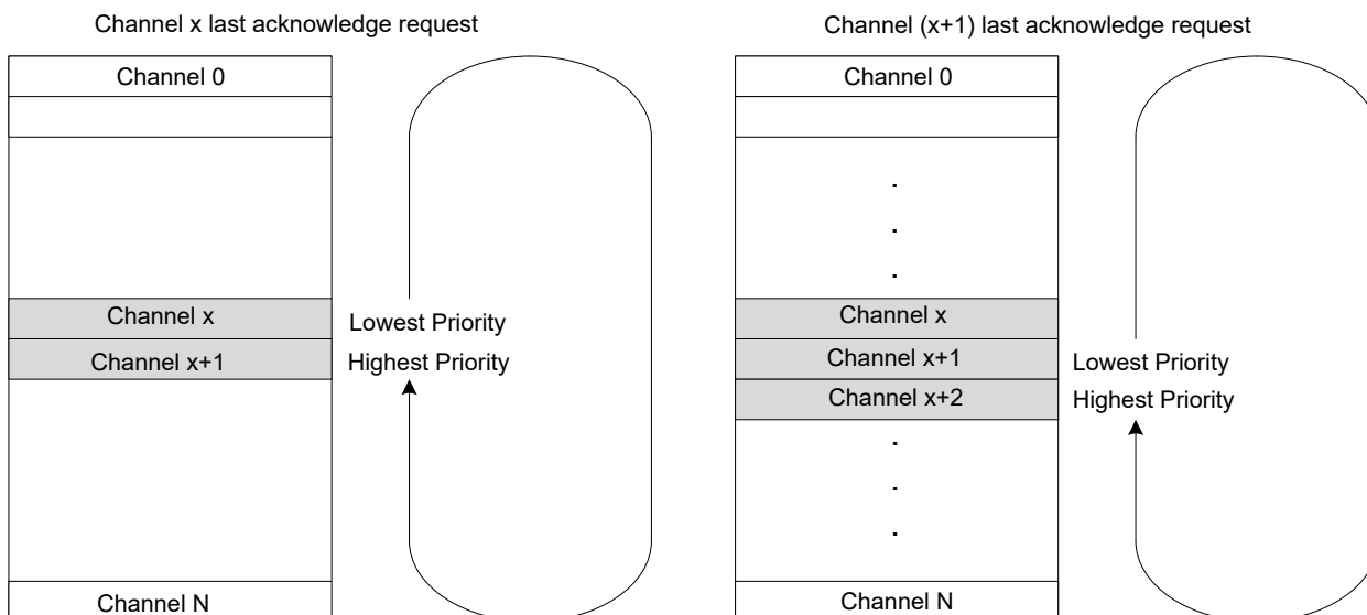
Figure 31-4. Round-Robin Scheduling
