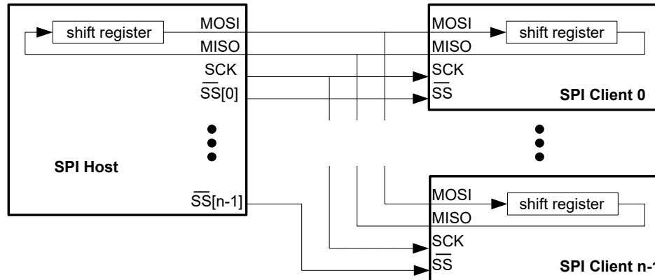
Figure 34-5. Multiple Clients in Parallel
