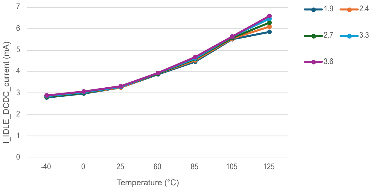
Figure 49-6. Idle Mode Current Consumption in MLDO Mode at FRC 8 MHz
