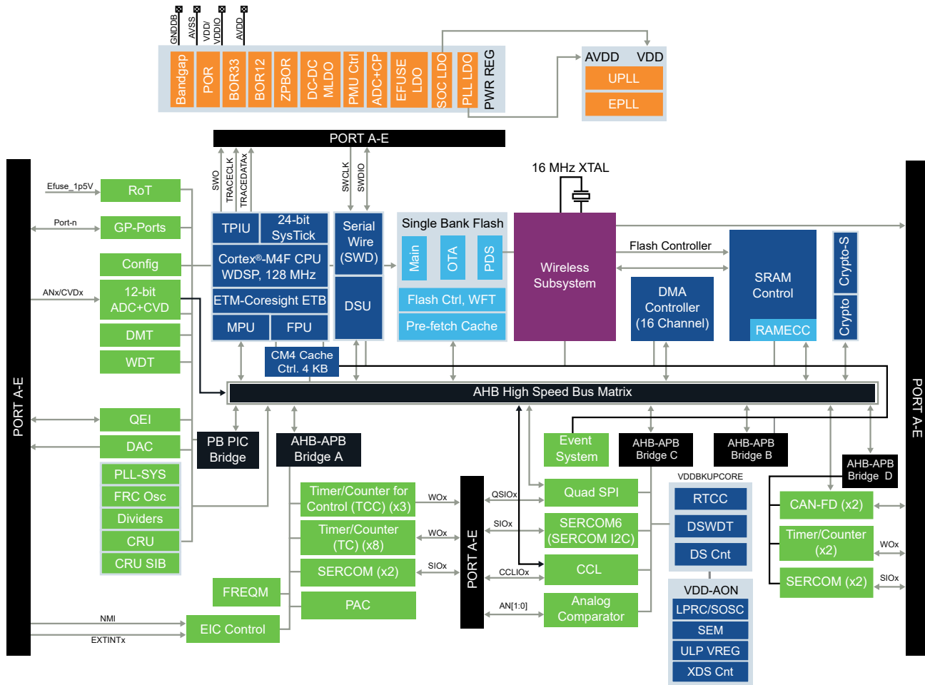
Figure 4-2. PIC32CX2051BZ66048 SoC Block Diagram
