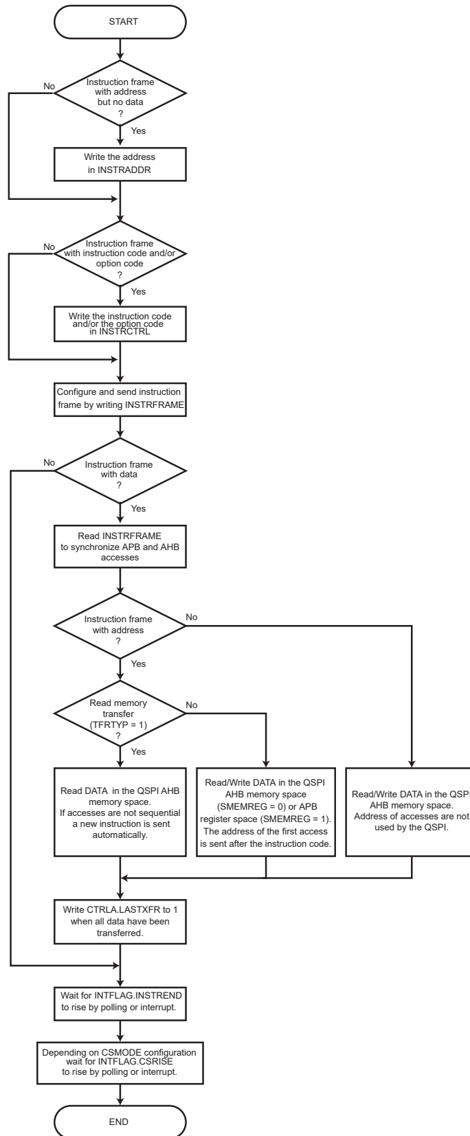
Figure 36-10. Instruction Transmission Flow Diagram
