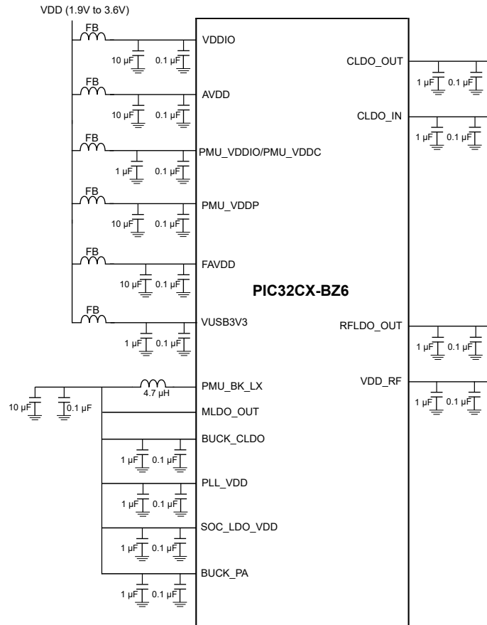
Figure 8-2. Typical Power Supply Connection for SoC
