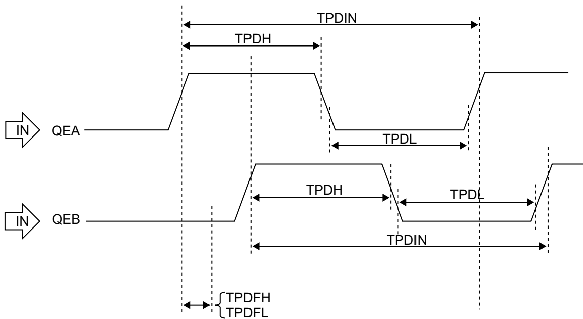
Figure 49-33. Quadrature Encoder (QEI) Input AC Timing Diagram
