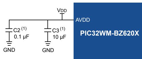
Figure 5-3. Recommended Module Power Supply Connections
