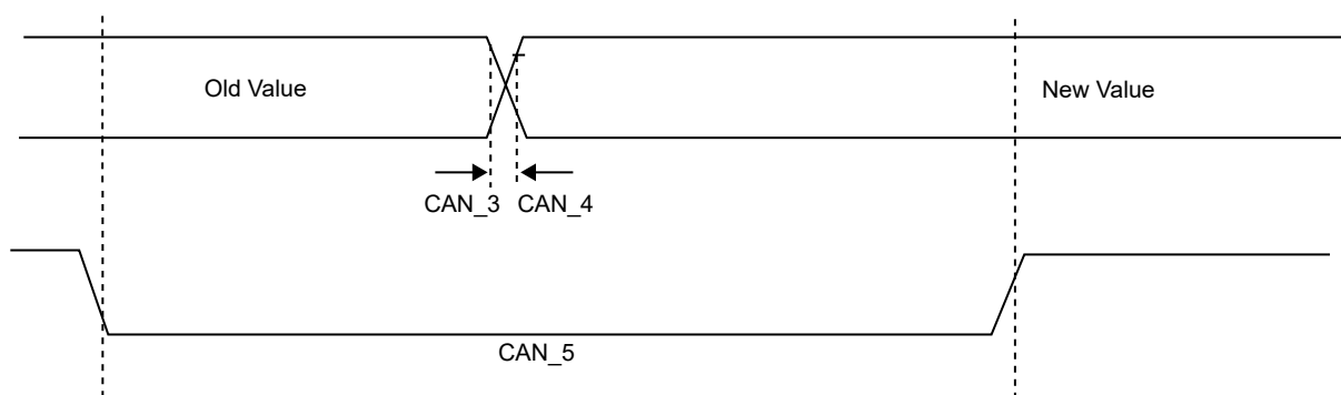
Figure 49-26. CANx Module AC Timing Diagram
