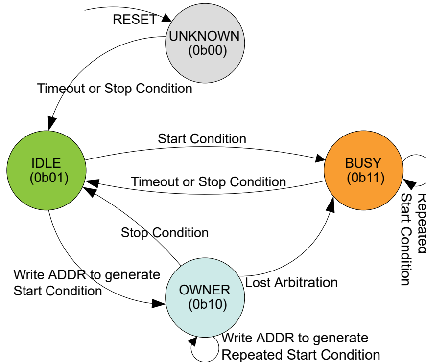
Figure 35-4. Bus State Diagram
