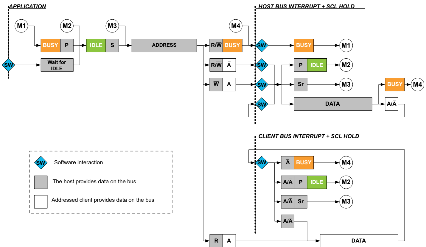
Figure 35-5. I 2 C Host Behavioral Diagram (SCLSM = 0)
