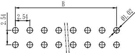
Recommended PCB Layout Top View
