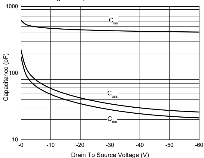
Fig. 9 - Capacitance Characteristics
