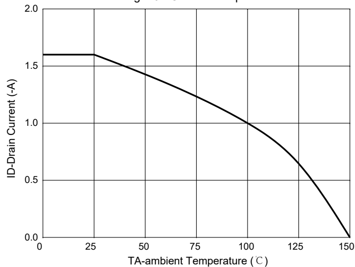
Fig. 10 - Current dissipation
