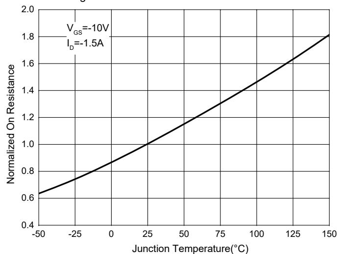
Fig.8-NormalizedOnResistanceCharacteristics
