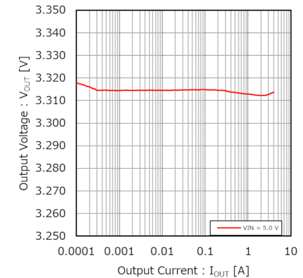
Figure 39. Output Voltage vs Output Current (Load Regulation) ( V_{OUT} = 3.3\text{ V} )
