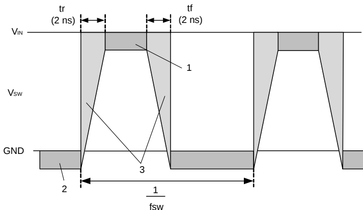
Figure 72. SW Waveform
