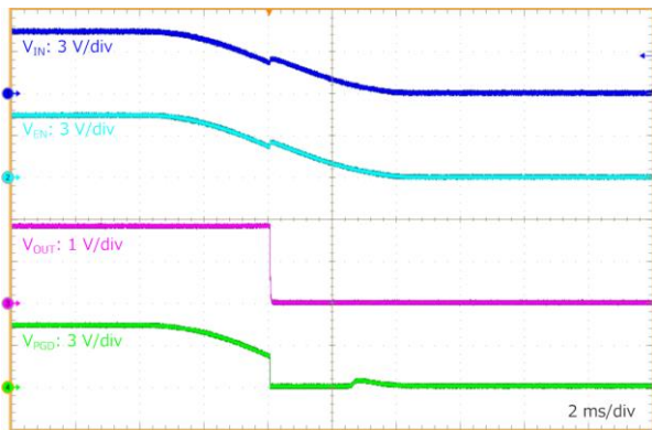
Figure 63. VIN Shutdown at RLoad = 0.45 Ω (VIN = VEN = 5 V to 0 V, VOUT = 1.8 V)
