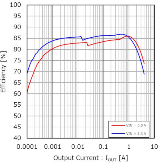
Figure 28. Efficiency vs Output Current (VOUT = 0.6 V)
