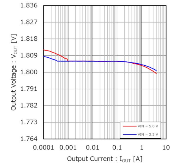
Figure 37. Output Voltage vs Output Current (Load Regulation) ( V_{OUT} = 1.8\text{ V} )
