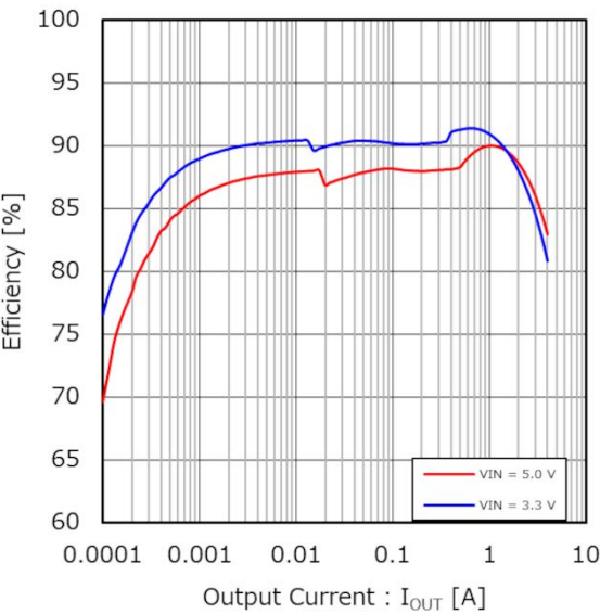
Figure 30. Efficiency vs Output Current (VOUT = 1.2 V)
