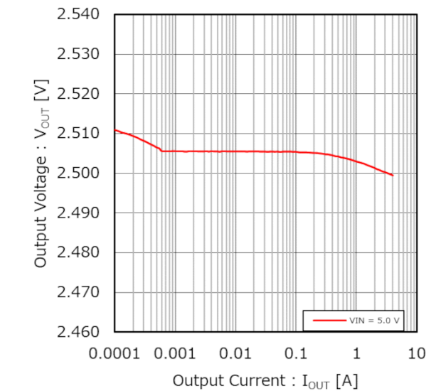
Figure 38. Output Voltage vs Output Current (Load Regulation) ( V_{OUT} = 2.5\text{ V} )
