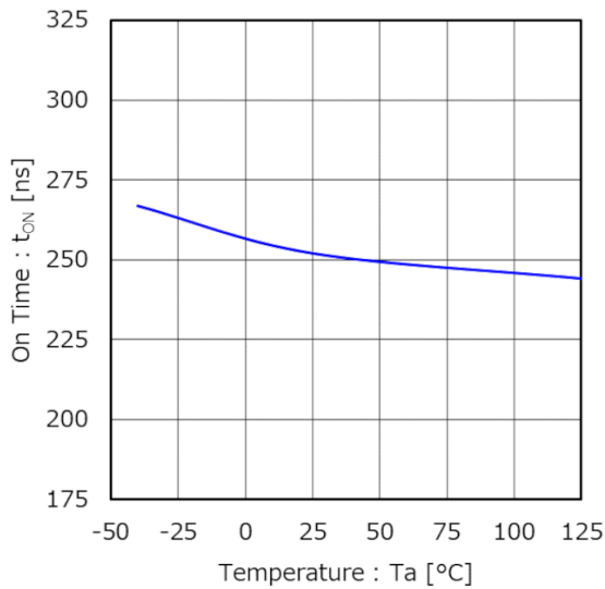
Figure 9. On Time vs Temperature ( V_{IN} = 3.3\text{ V} , V_{OUT} = 1.8\text{ V} , PWM Mode)
