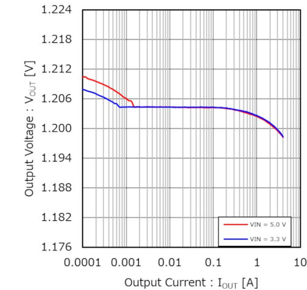
Figure 36. Output Voltage vs Output Current (Load Regulation) ( V_{OUT} = 1.2\text{ V} )
