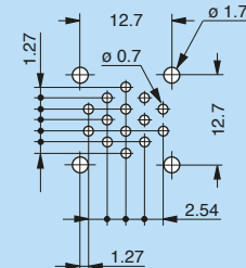
P12 - EPG.1B.314 Screw mount
