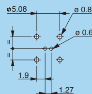
P11 - EPG-EXG (0B/1B.302) Solder mount
