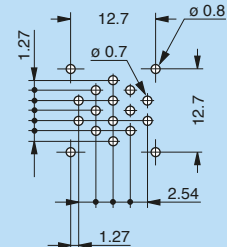
P12 - EPG.1B.314 Solder mount
