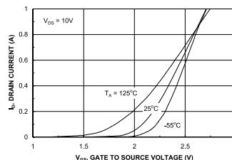
Figure 5. Transfer Characteristics.
