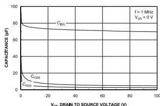
Figure 8. Capacitance Characteristics.
