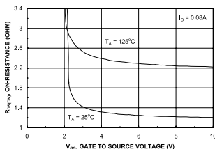
Figure 4. On-Resistance Variation with Gate-to-Source Voltage.
