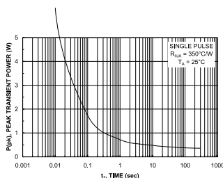
Figure 10. Single Pulse Maximum Power Dissipation.
