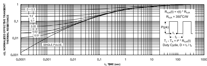
Figure 11. Transient Thermal Response Curve.
