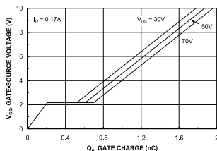
Figure 7. Gate Charge Characteristics.
