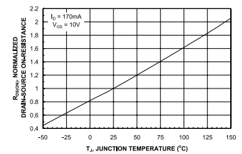
Figure 3. On-Resistance Variation with Temperature.
