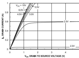
Figure 1. On-Region Characteristics.
