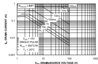
Figure 9. Maximum Safe Operating Area.
