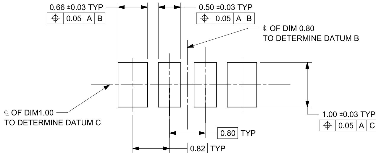
DETAIL A SCALE 20:1
