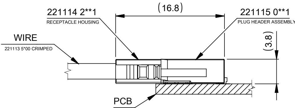
△7 MATED CONNECTORS
