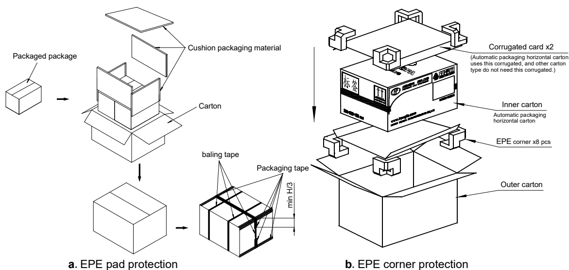
Figure 27 Reference of bulk delivery reinforced packaging
