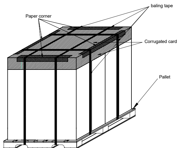
Figure 26 Pallet container packaging delivery reference
