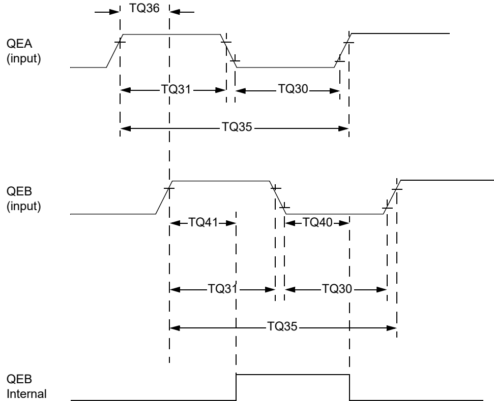
Figure 33-18. QEA/QEB Input Characteristics
