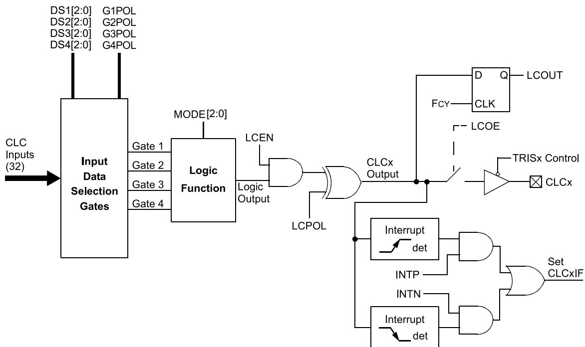
Figure 23-1. CLCx Module
