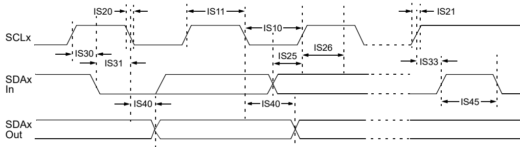
Figure 33-16. I2Cx Bus Data Timing Characteristics (Client Mode)
