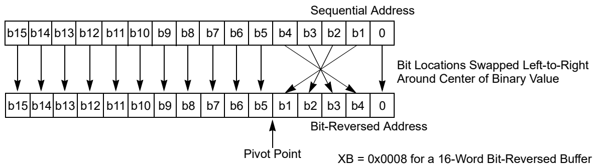
Figure 4-11. Bit-Reversed Addressing Example
