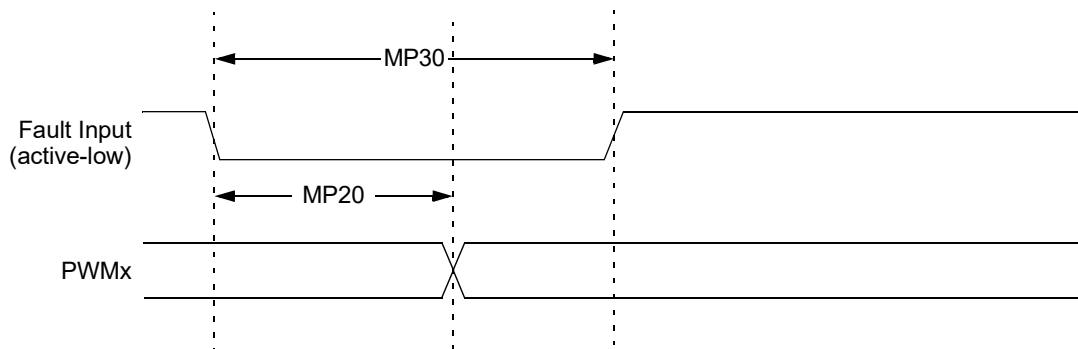
Figure 33-5. High-Speed PWMx Module Fault Timing Characteristics
