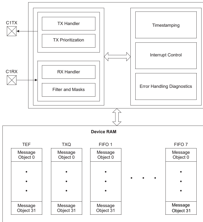
Figure 11-1. CAN FD Module Block Diagram
