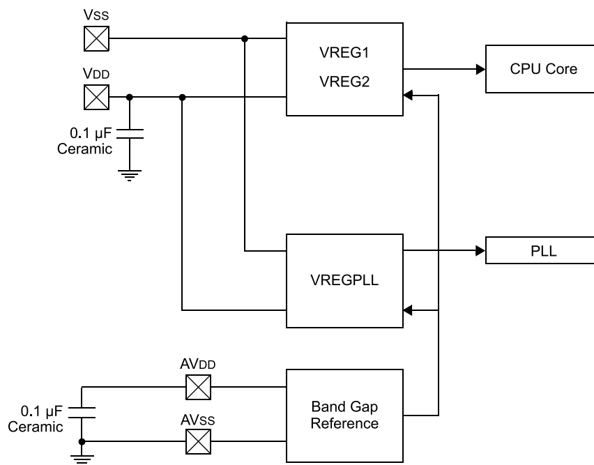
Figure 30-1. Internal Regulator
