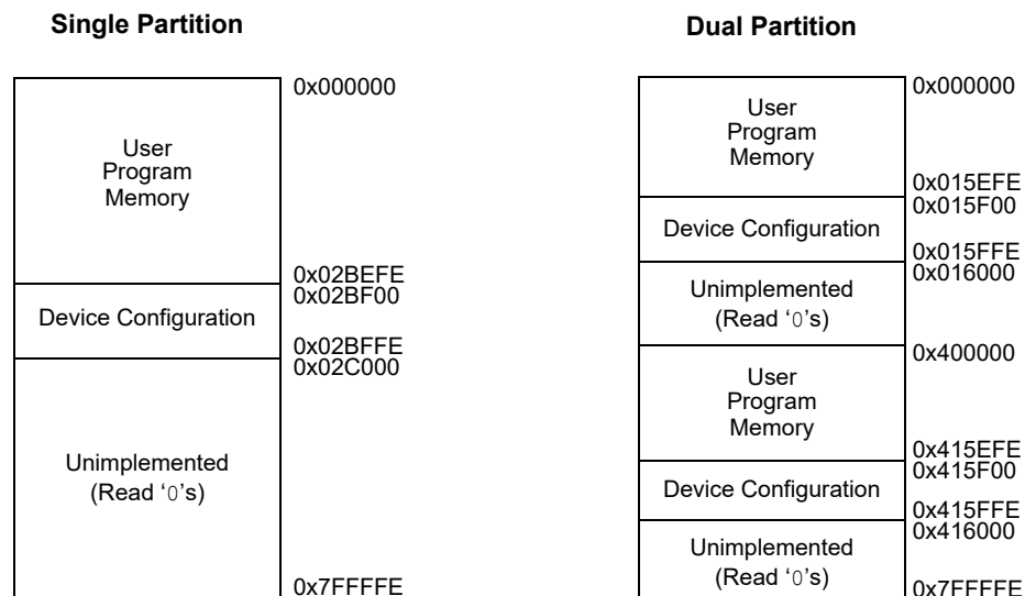
Figure 4-3. Program Memory Map for dsPIC33CK256MP60X/30X Devices (1)
