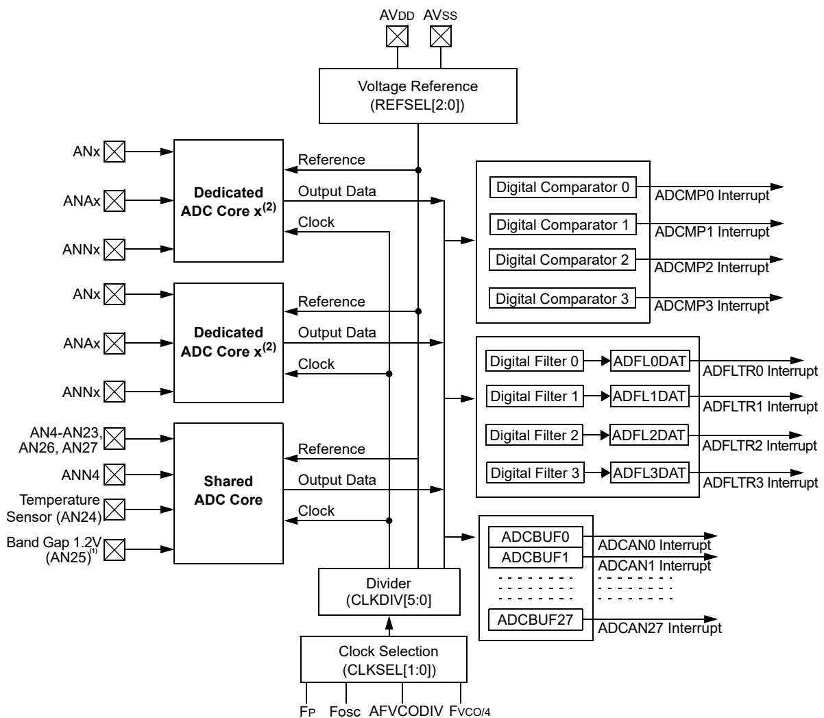
Figure 13-1. ADC Module Block Diagram
