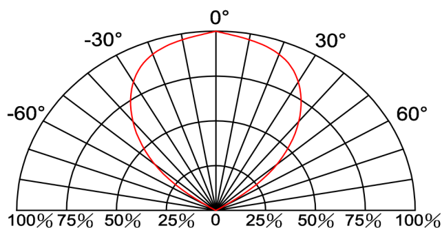
Fig.5 Directive Radiation
