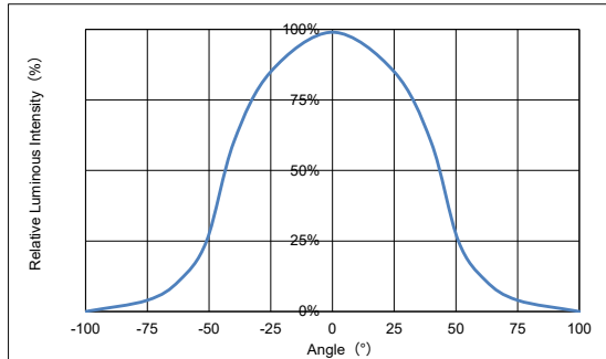
Radiation Diagram
