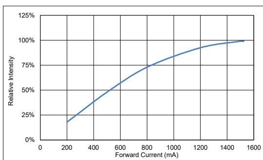
Forward Current vs. Relative Intensity
