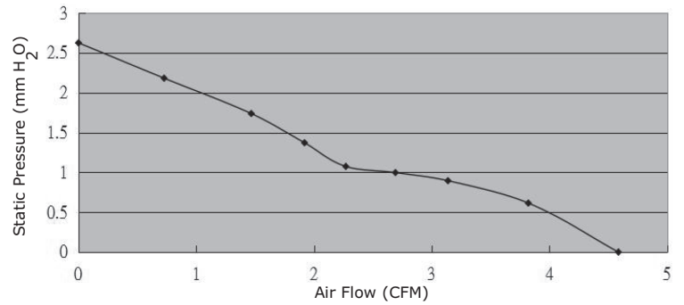
CFM-3510BF-170-222
