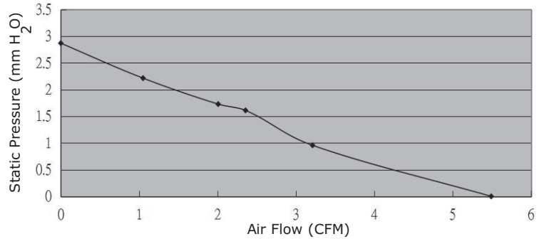
CFM-4010B-265-251
