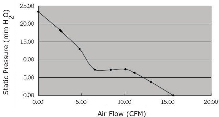
CFM-4015B-1135-415
