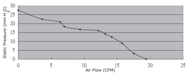
CFM-4020BG-1165-498
