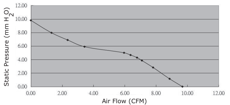
CFM-4028BG-180-369
