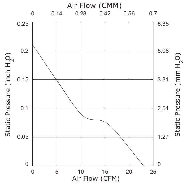
CFM-6020V-150-335
