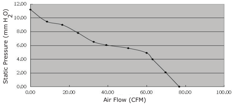
CFM-9238B-140-473
