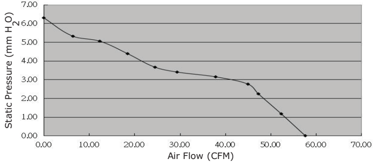
CFM-9238B-230-410
