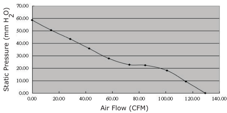
CFM-9238BF-195-628
