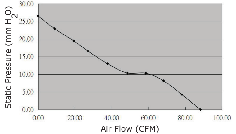
CFM-9238BF-295-628
