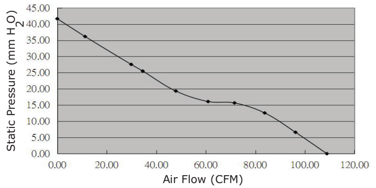
CFM-9238BF-180-585
