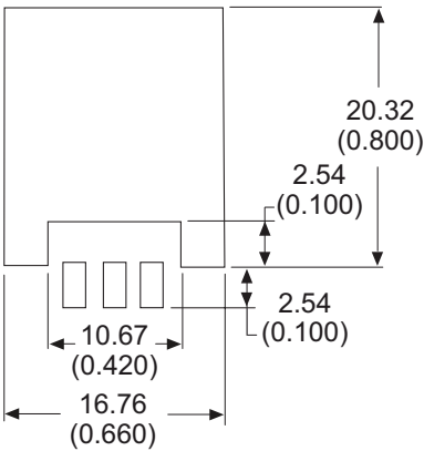
Recommended Copper Pad Layout Top View
