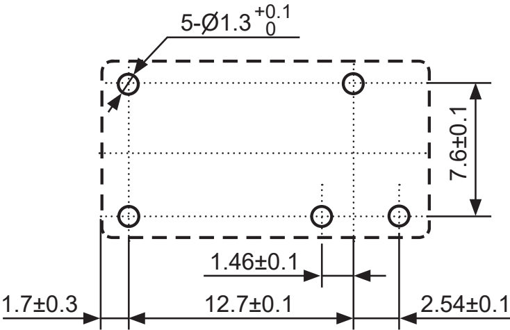
Recommended PCB Layout Bottom View
