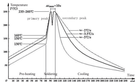
Double-wave Soldering Curve
