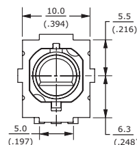
ITEM DESCRIPTION MATERIAL PLATING/COLOR A base PBT [UL94V-0] black B shaft PC [UL94V-0] black C reed nickel-zinc alloy D bracket iron bright tin E terminals cold rolled steel dark tin
