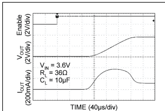
FIGURE 2-36: MIC94042 Turn-On/Turn-Off Timing.
