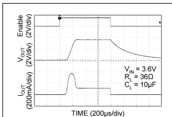
FIGURE 2-35: MIC94042 Turn-On/Turn-Off Timing.
