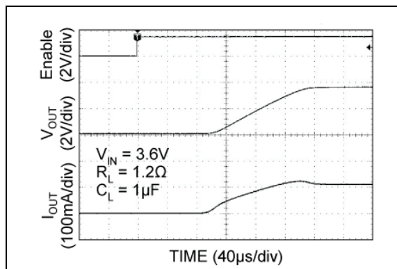
FIGURE 2-34: MIC94042 Turn-On/Turn-Off Timing.
