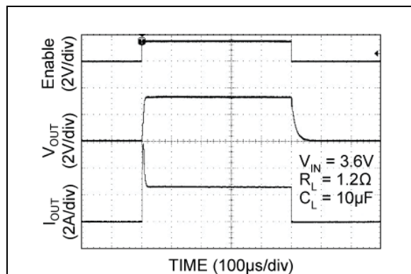
FIGURE 2-31: MIC94041 Turn-On/Turn-Off Timing.
