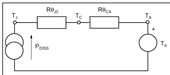
FIGURE 4-2: Simple Thermal Circuit.
