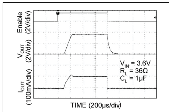
FIGURE 2-33: MIC94042 Turn-On/Turn-Off Timing.
