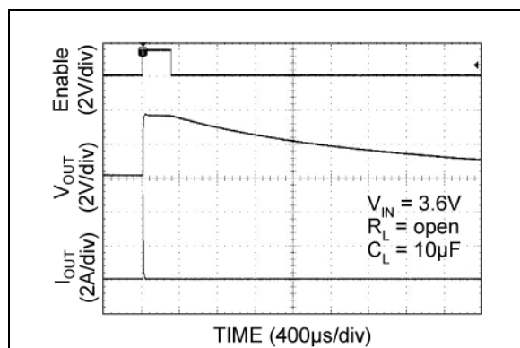
FIGURE 2-32: MIC94041 Turn-On/Turn-Off Timing.
