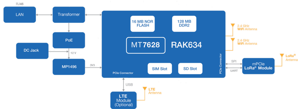
Figure 1: WisGate Edge Lite 2 Block Diagram
