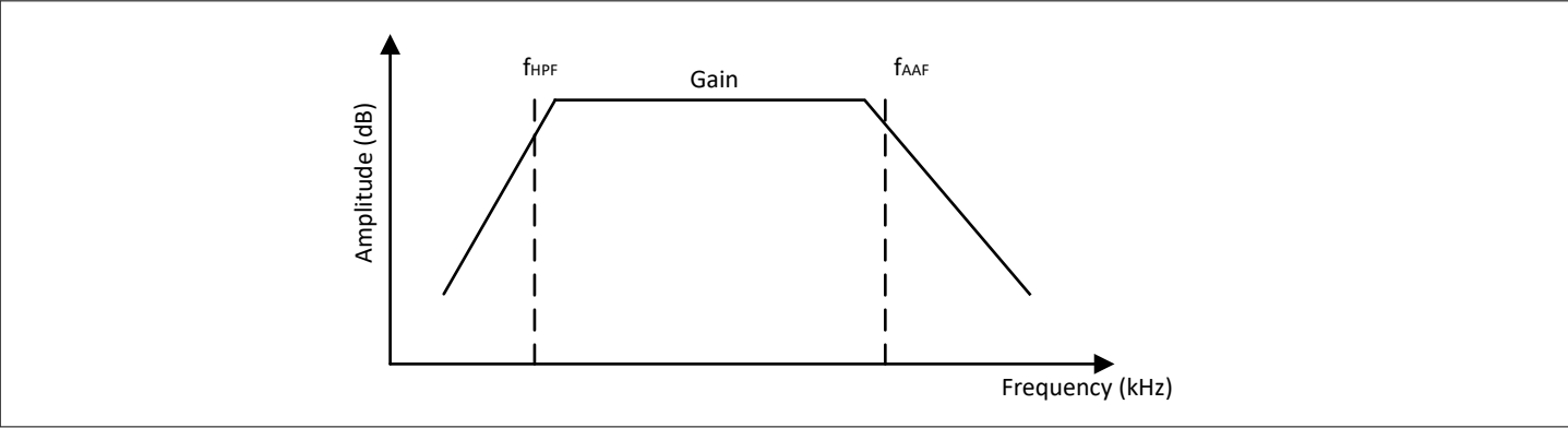
Figure 13 Baseband bandpass characteristic
