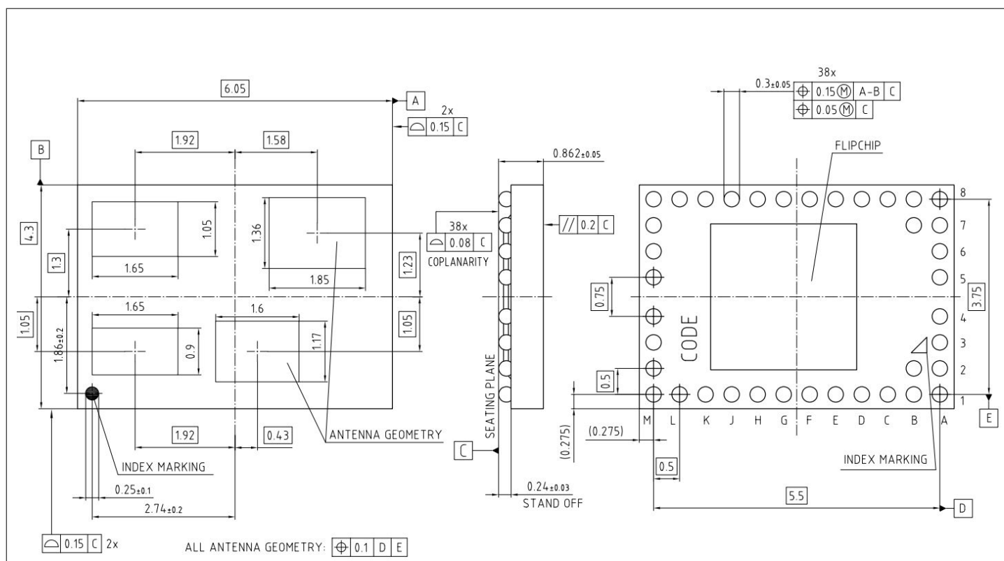
Figure 16 Package outline of PG-VF2BGA-38-1
