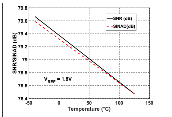
FIGURE 2-17: SNR/SINAD vs. Temperature: V_{REF} = 1.8\text{V} .
