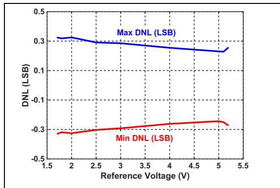
FIGURE 2-6: DNL vs. Reference Voltage.
