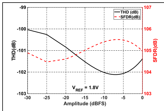
FIGURE 2-28: THD/SFDR vs. Input Amplitude: V_{REF} = 1.8\text{V} .
