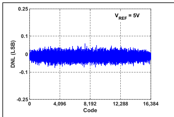
FIGURE 2-4: DNL vs. Output Code: V_{REF} = 5\text{V} .
