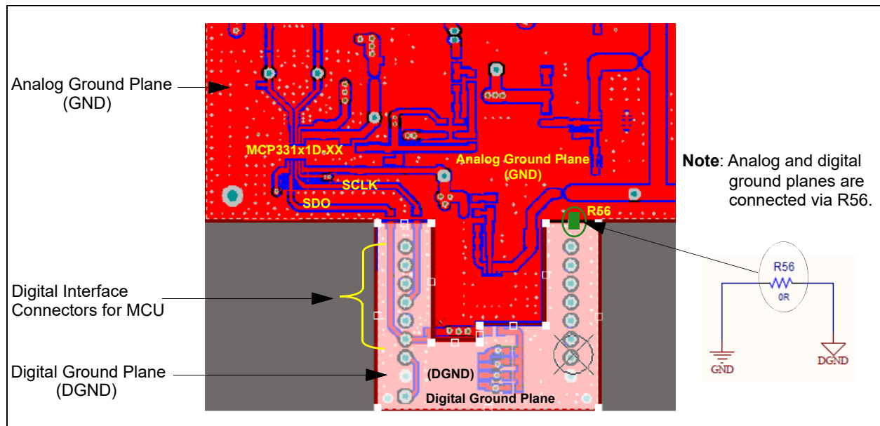
FIGURE 7-2: PCB Layout Example: Analog and Digital Ground Planes.
