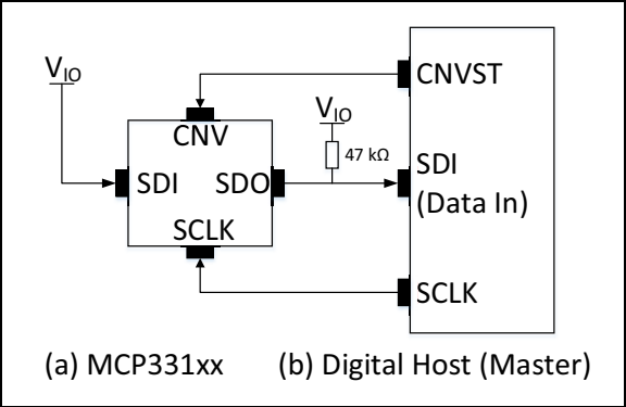
FIGURE 6-1: Connection Diagram for 3-Wire CS Mode without BUSY Status Indicator Output Bit.
