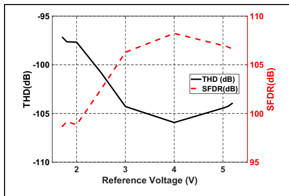
FIGURE 2-16: THD/SFDR vs. Reference Voltage.
