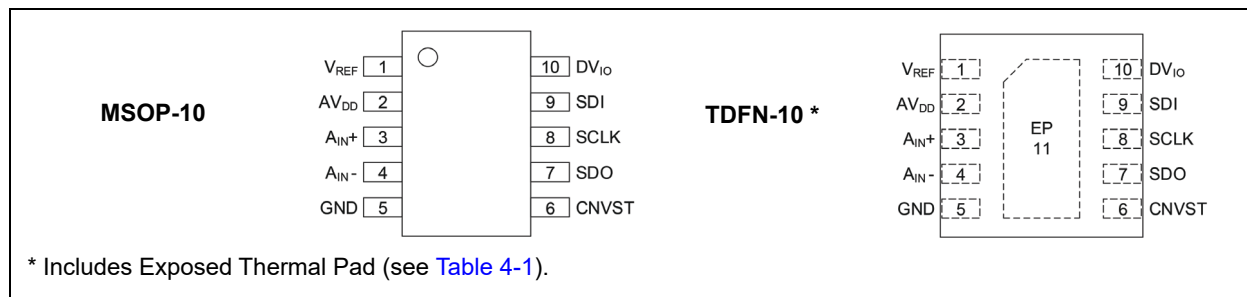
FIGURE 4-1: Pin Configurations.
