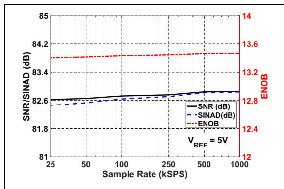
FIGURE 2-26: SNR/SINAD/ENOB vs. Sample Rate: V_{REF} = 5\text{V} .
