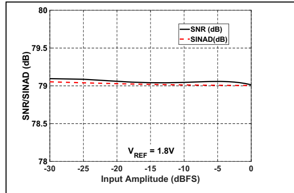
FIGURE 2-24: SNR/SINAD vs. Input Amplitude: V_{REF} = 1.8\text{V} .
