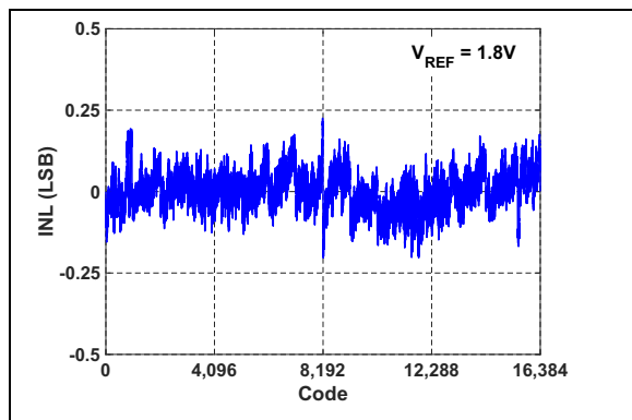
FIGURE 2-2: INL vs. Output Code: V_{REF} = 1.8\text{V} .
