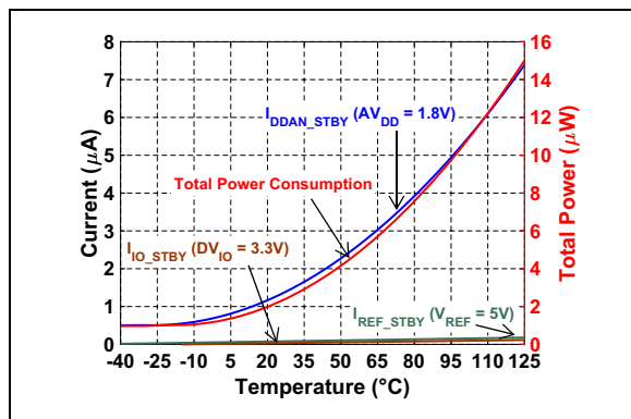
FIGURE 2-38: Power Consumption vs. Temperature during Shutdown (Standby).
