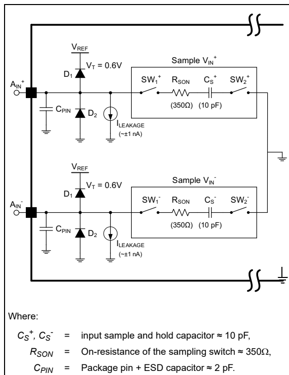
FIGURE 5-1: Simplified Equivalent Analog Input Circuit.
