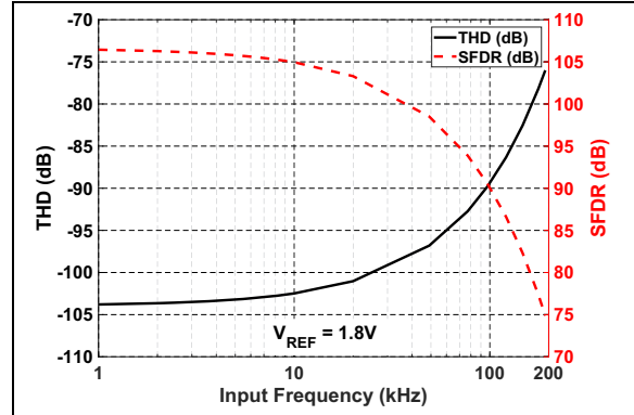
FIGURE 2-23: THD/SFDR vs. Input Frequency: V_{REF} = 1.8\text{V} .
