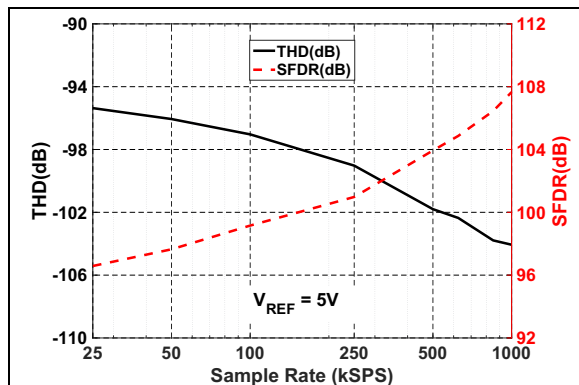
FIGURE 2-27: THD/SFDR vs Sample Rate: V_{REF} = 5\text{V} .
