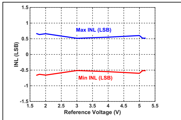
FIGURE 2-3: INL vs. Reference Voltage.
