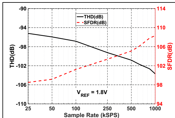
FIGURE 2-30: THD/SFDR vs Sample Rate: V_{REF} = 1.8\text{V} .
