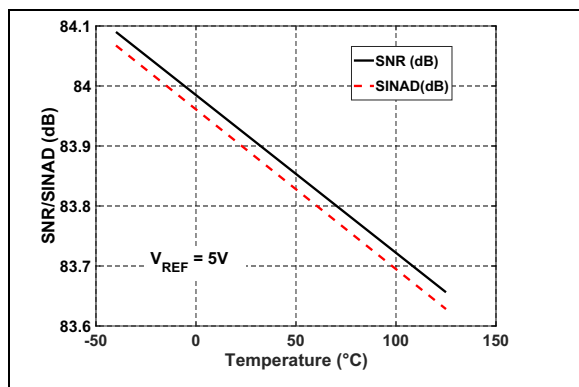
FIGURE 2-14: SNR/SINAD vs. Temperature: V_{REF} = 5\text{V} .
