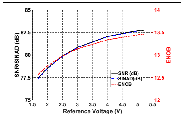
FIGURE 2-13: SNR/SINAD/ENOB vs. Reference Voltage.
