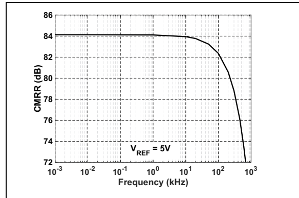
FIGURE 2-34: CMRR vs. Input Frequency: V_{REF} = 5\text{V} .
