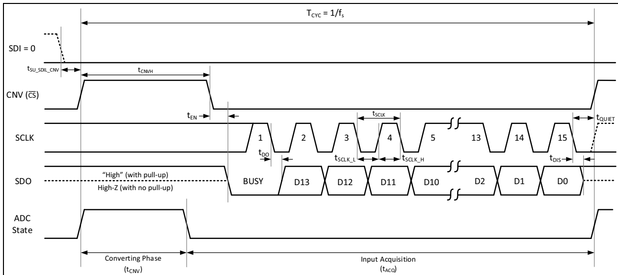
FIGURE 6-7: Timing Diagram for 3-Wire \overline{\text{CS}} Mode with BUSY Status Indicator Output Bit, Late CNV.
