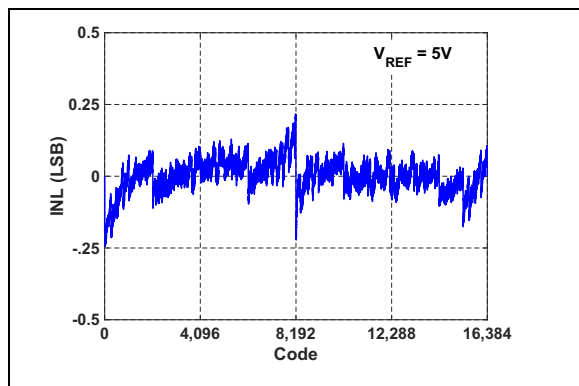
FIGURE 2-1: INL vs. Output Code: V_{REF} = 5\text{V} .
