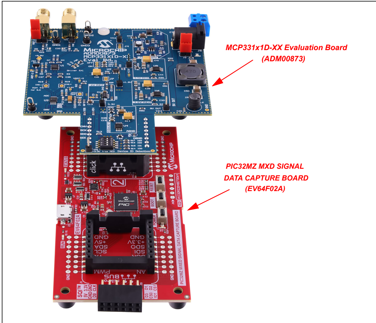
FIGURE 7-1: MCP331x1D-XX Evaluation Kit.
