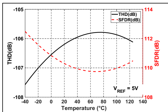
FIGURE 2-15: THD/SFDR vs. Temperature: V_{REF} = 5\text{V} .
