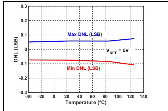
FIGURE 2-10: DNL vs. Temperature.
