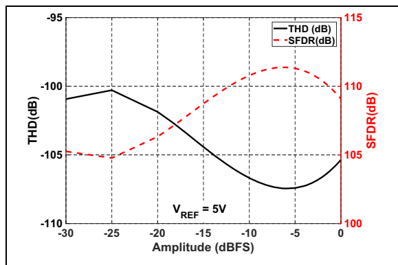
FIGURE 2-25: THD/SFDR vs. Input Amplitude: V_{REF} = 5\text{V} .
