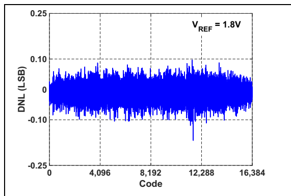
FIGURE 2-5: DNL vs. Output Code: V_{REF} = 1.8\text{V} .
