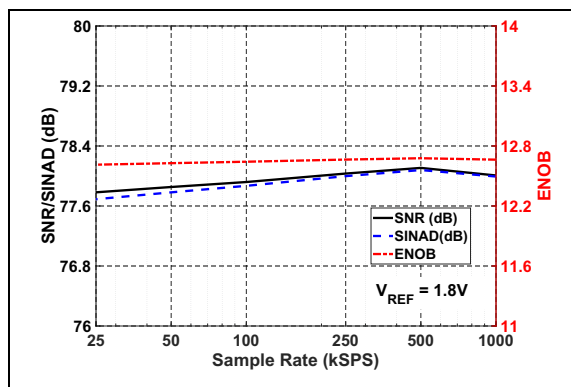
FIGURE 2-29: SNR/SINAD/ENOB vs. Sample Rate: V_{REF} = 1.8\text{V} .
