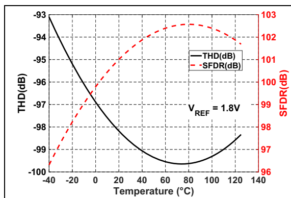
FIGURE 2-18: THD/SFDR vs. Temperature: V_{REF} = 1.8\text{V} .
