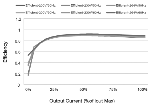
Efficiency Curve
