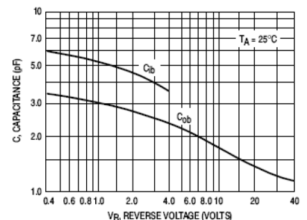
Figure 5. Capacitances
