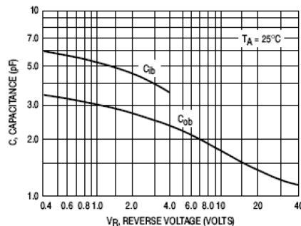
Figure 5. Capacitances
