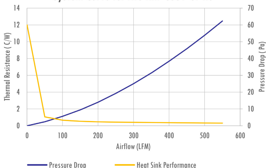
System Curve for ATS-KRP-3559-C1-R0
