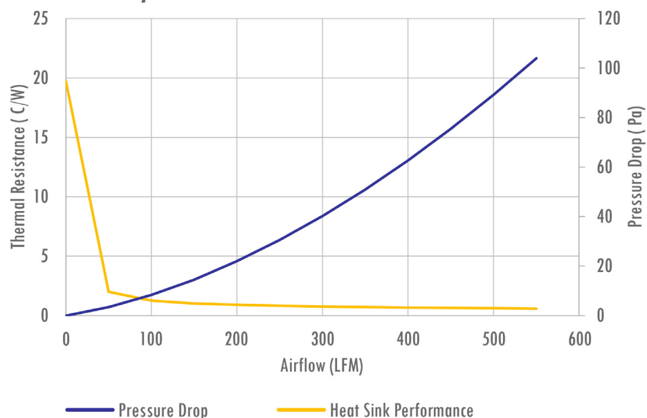
System Curve for ATS-KRP-3567-C1-R0
