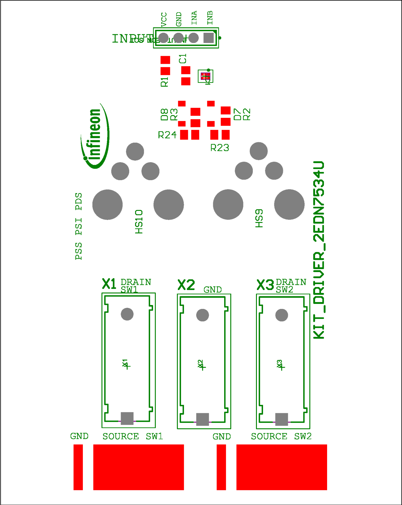
Figure 4 PCB top
