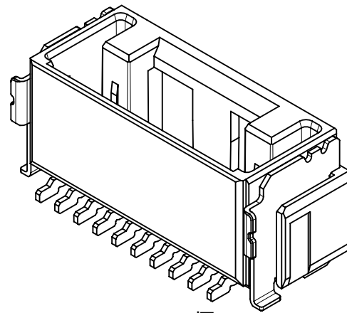
9-10極 9-10 CIRCUIT
