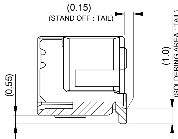
SECTION X-X
