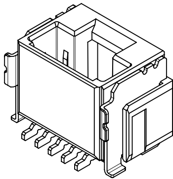
3-5極 3-5 CIRCUIT
