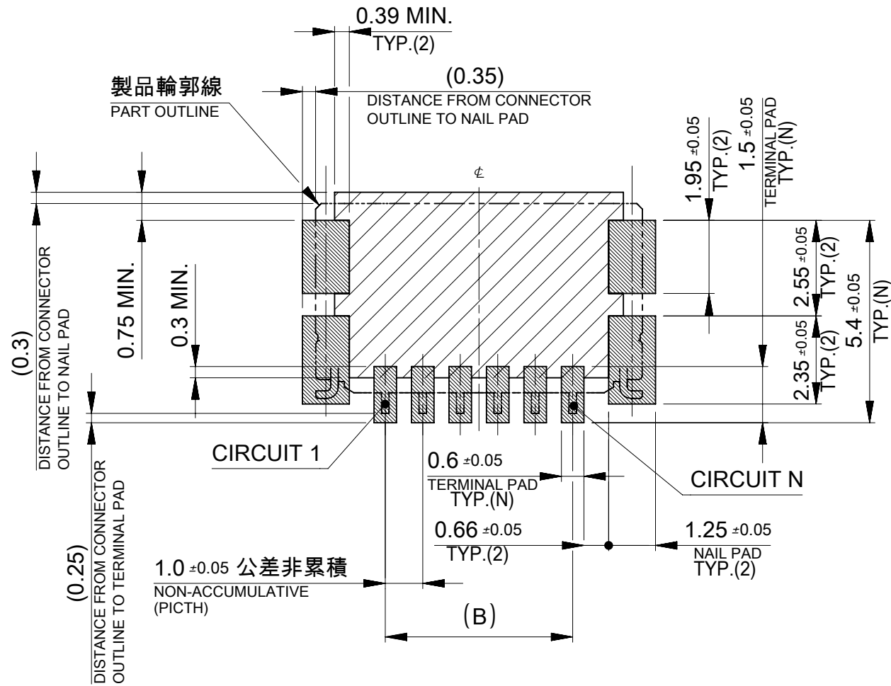
3-5極 3-5 CIRCUIT
