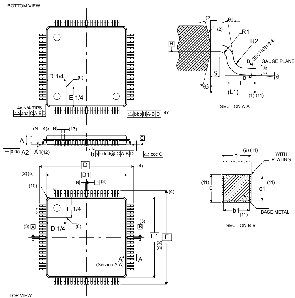
Figure 54. LQFP80 - Outline (15.)
