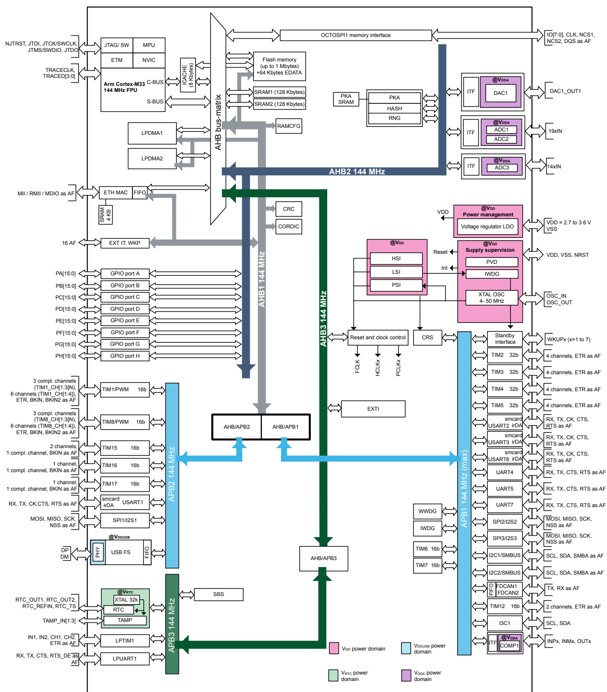
Figure 1. STM32C59xxx block diagram
