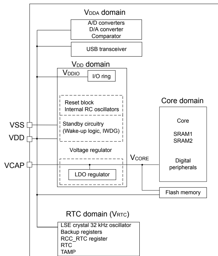
Figure 2. STM32C59xxx power supply overview
