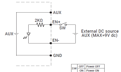
(C) Using external voltage source
