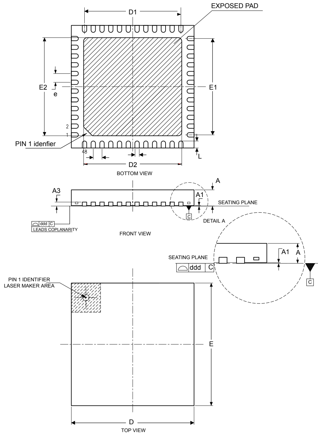
Figure 41. UFQFPN48 - Outline
