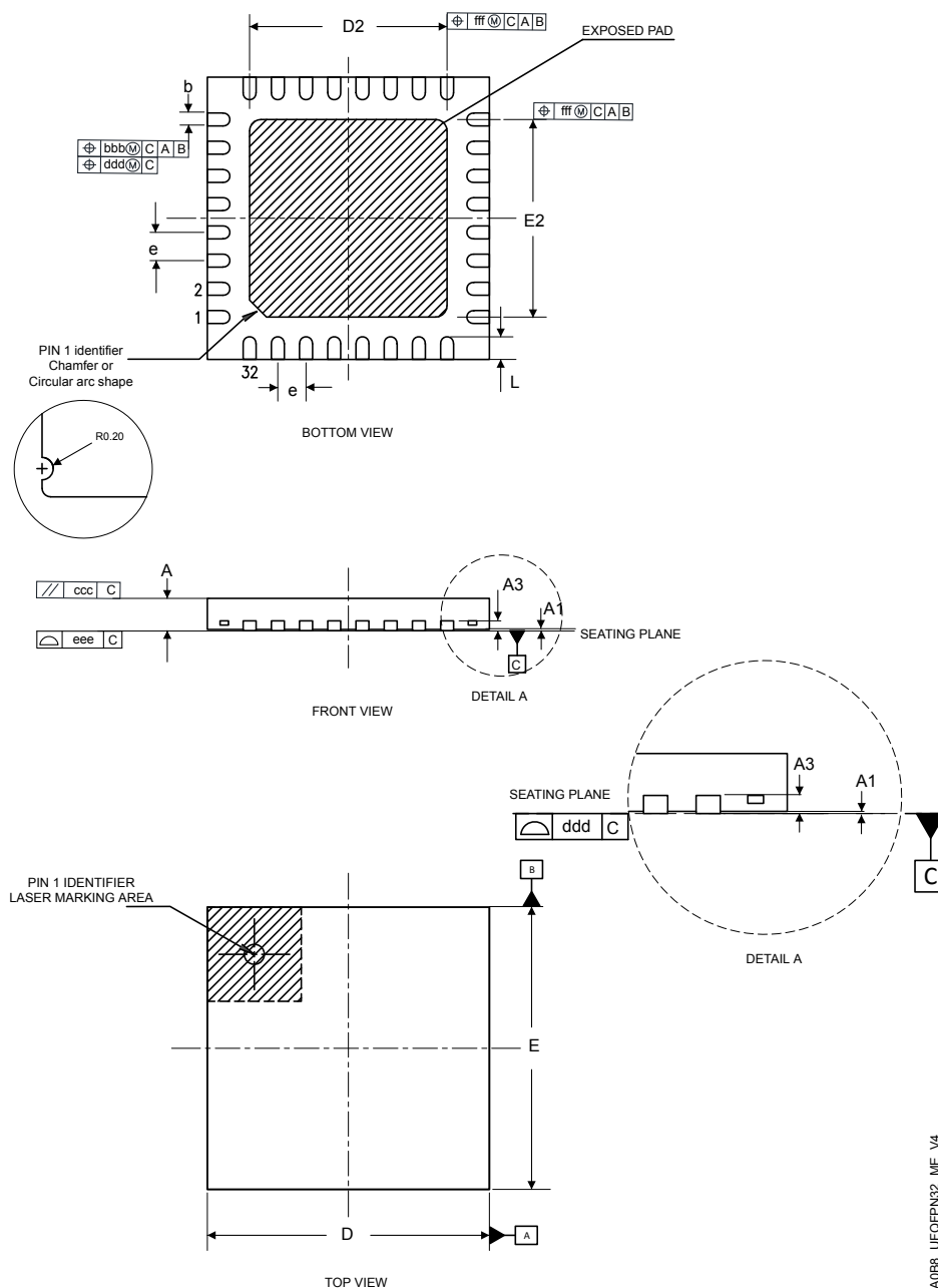
Figure 34. UFQFPN32 - Outline
