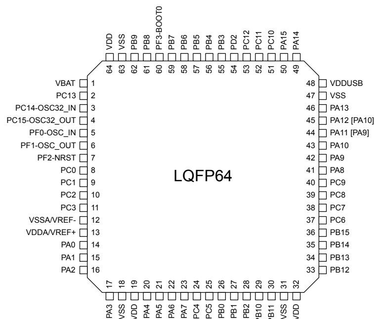
Figure 7. LQFP64 pinout
