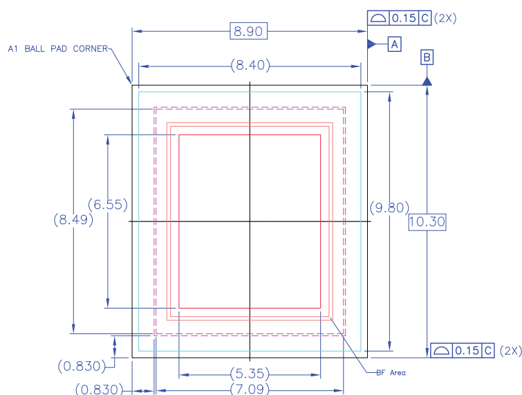
Figure 29. Top view
