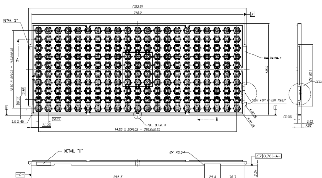
Figure 35. Tray dimensions
