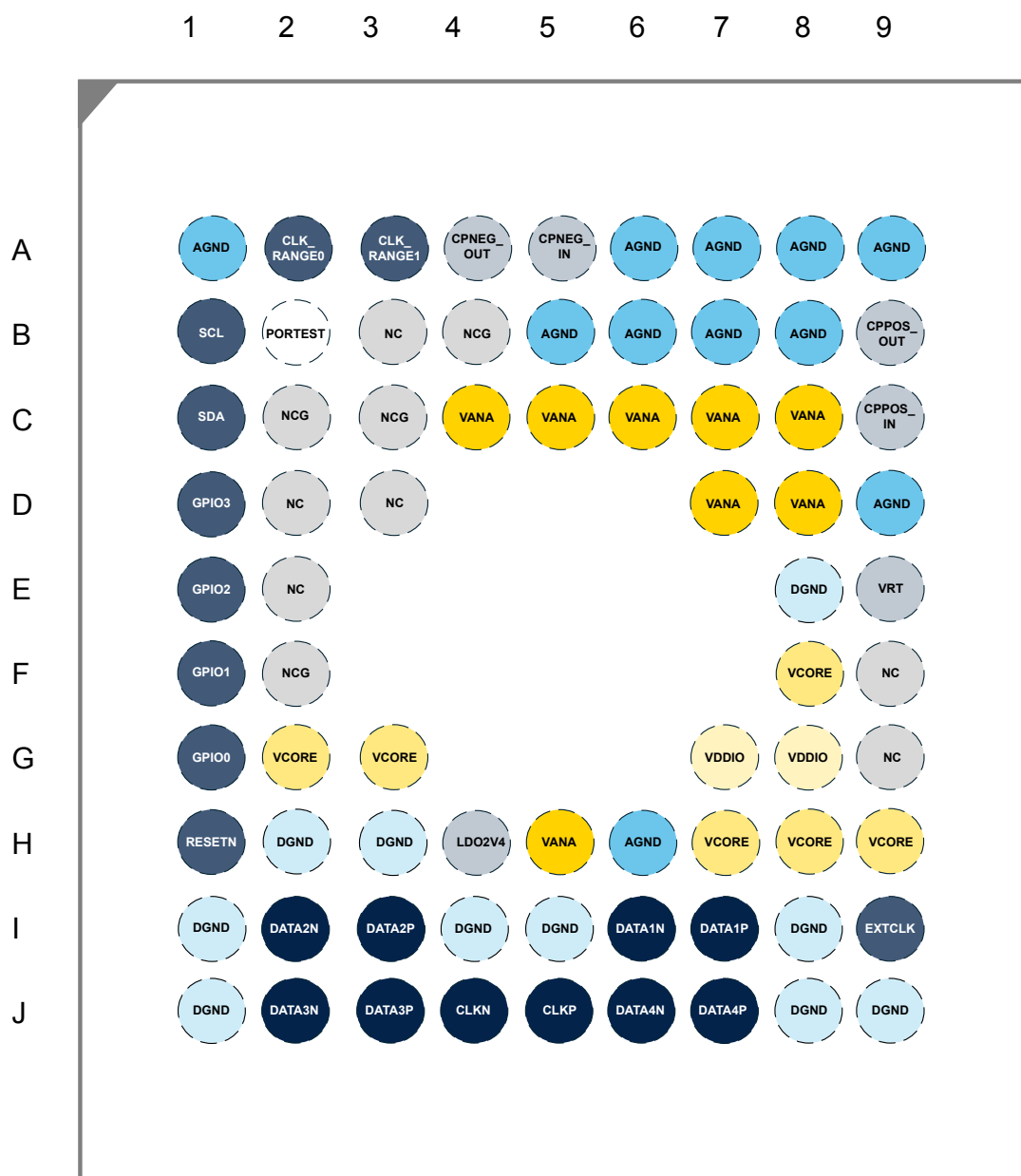
Figure 7. Ball assignment (see-through view)
