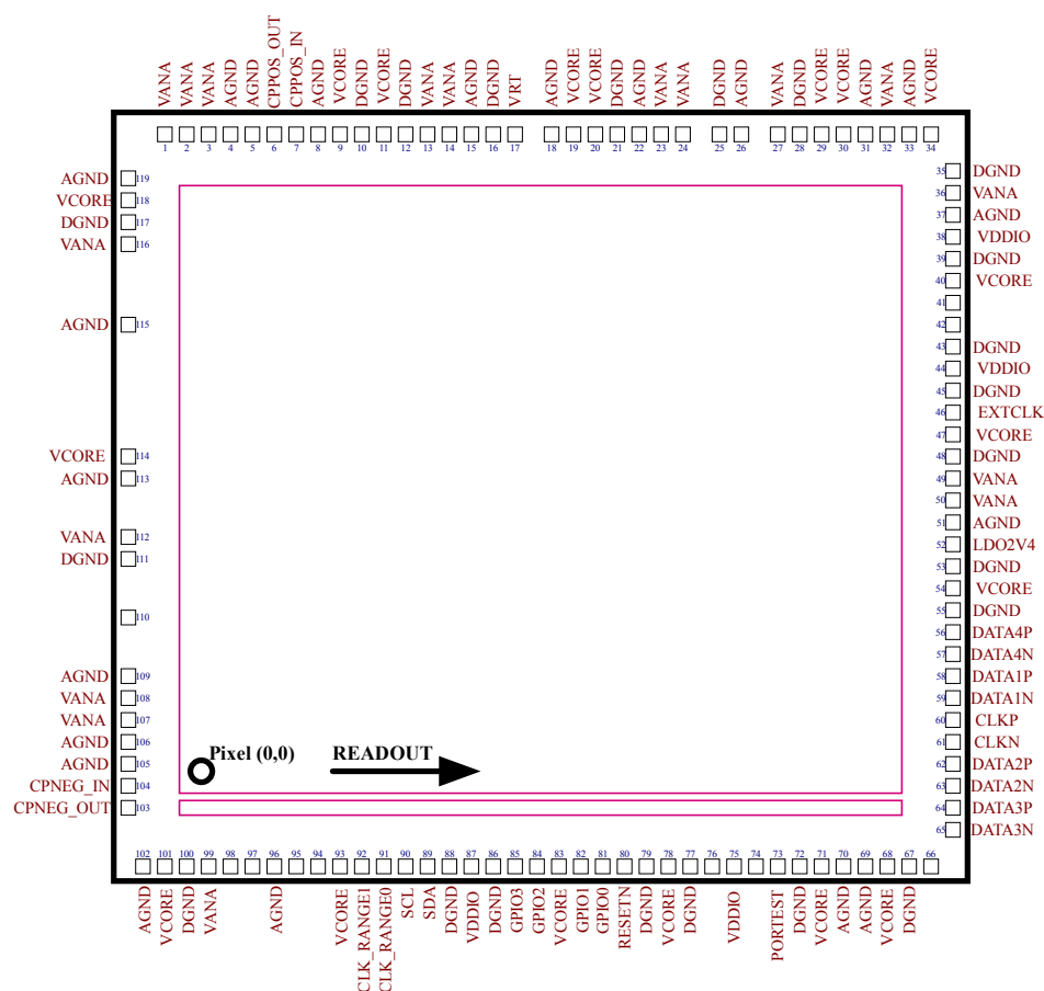
Figure 9. Pad assignment
