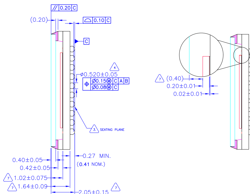
Figure 31. Side view
