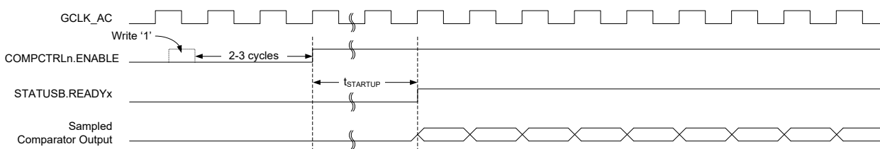
Figure 38-10. Continuous Mode SleepWalking
