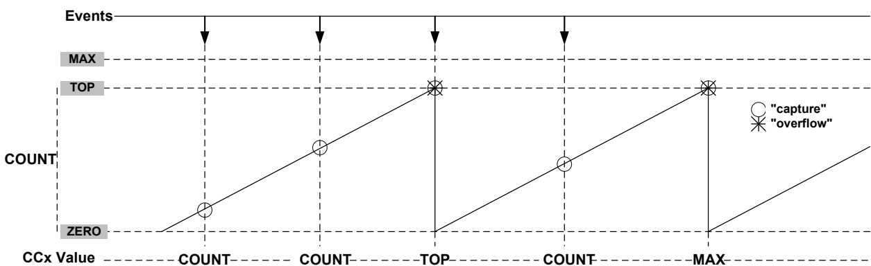
Figure 34-15. Time-Stamp
