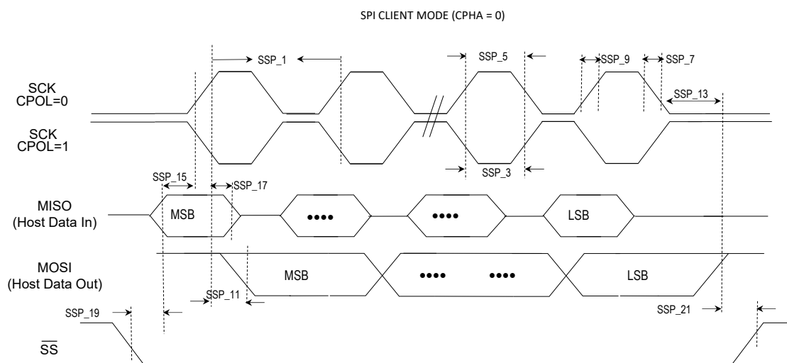
Figure 47-6. SPIx Client Module CPHA = 0 Timing Diagram
