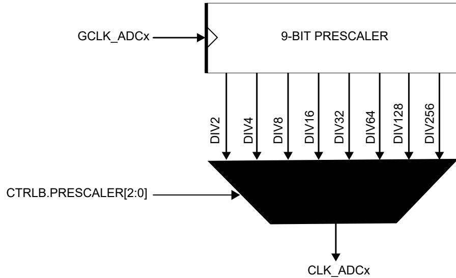
Figure 37-2. ADC Prescaler
