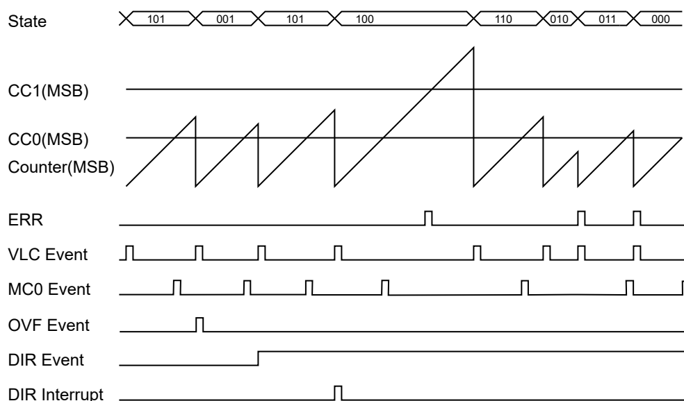
Figure 42-10. Hall Waveforms
