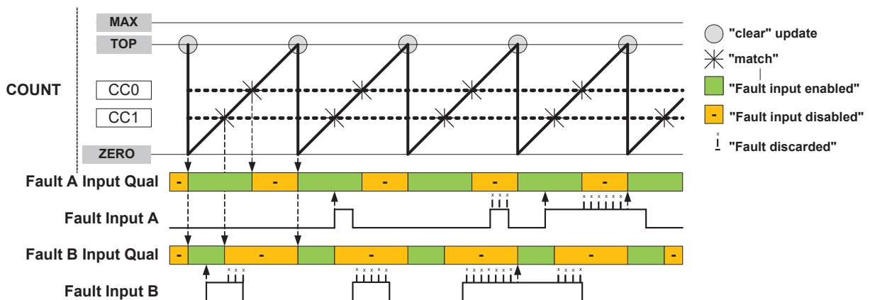
Figure 35-25. Fault Qualification in RAMP1 Operation
