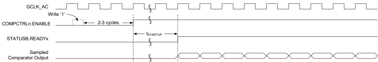
Figure 38-3. Continuous Measurement Example
