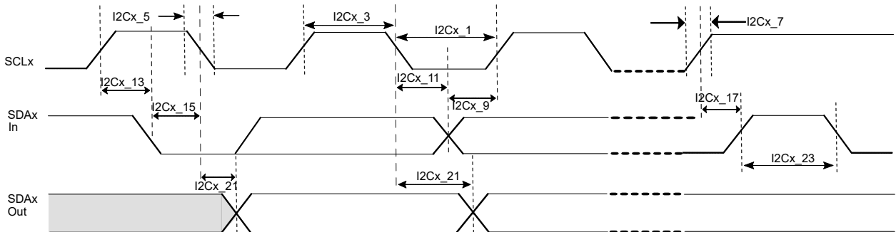
Figure 46-12. SERCOM I 2 C Bus Data Host Mode Timing Diagrams
