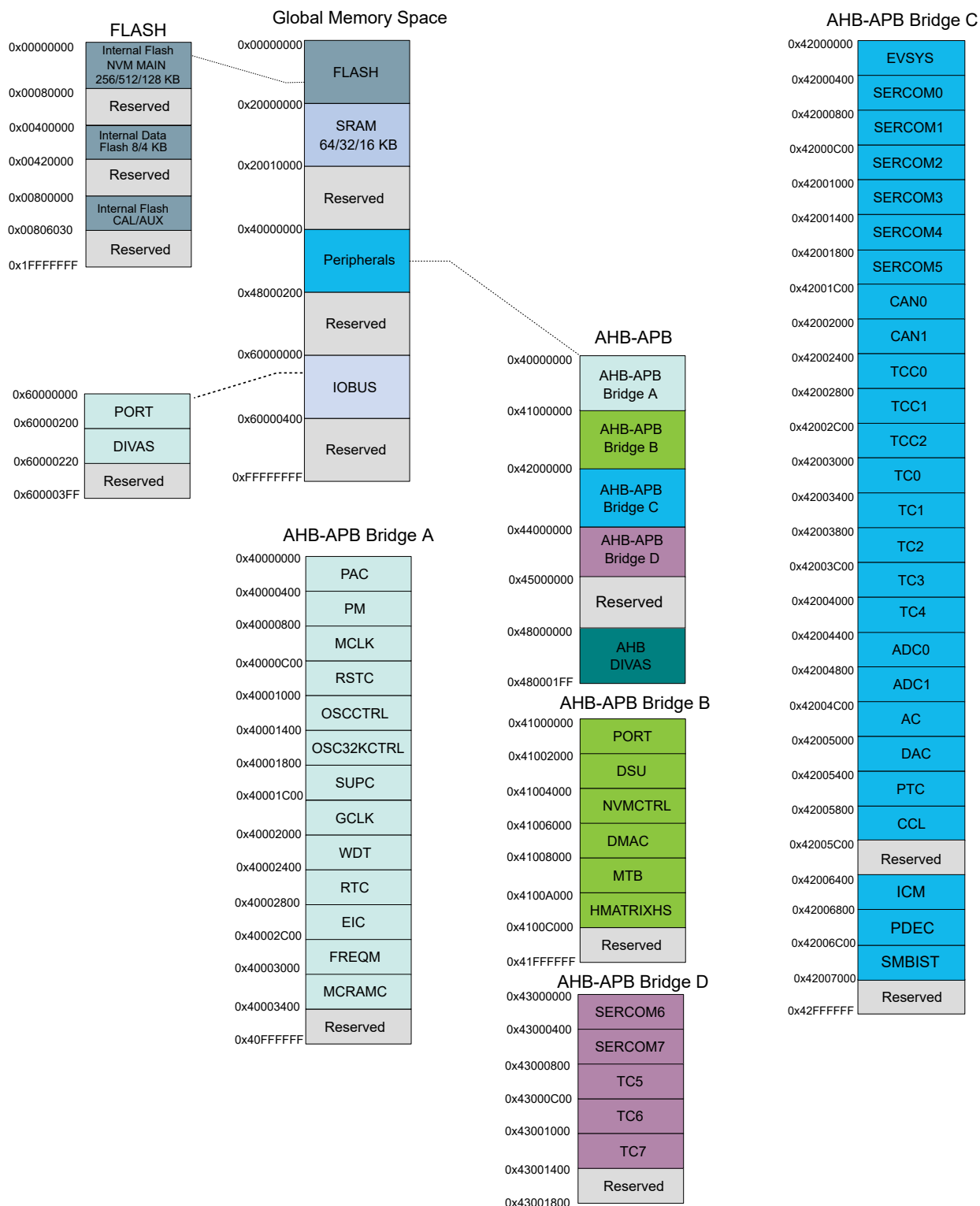
Figure 8-1. PIC32CM JH00/JH01 Product Mapping
