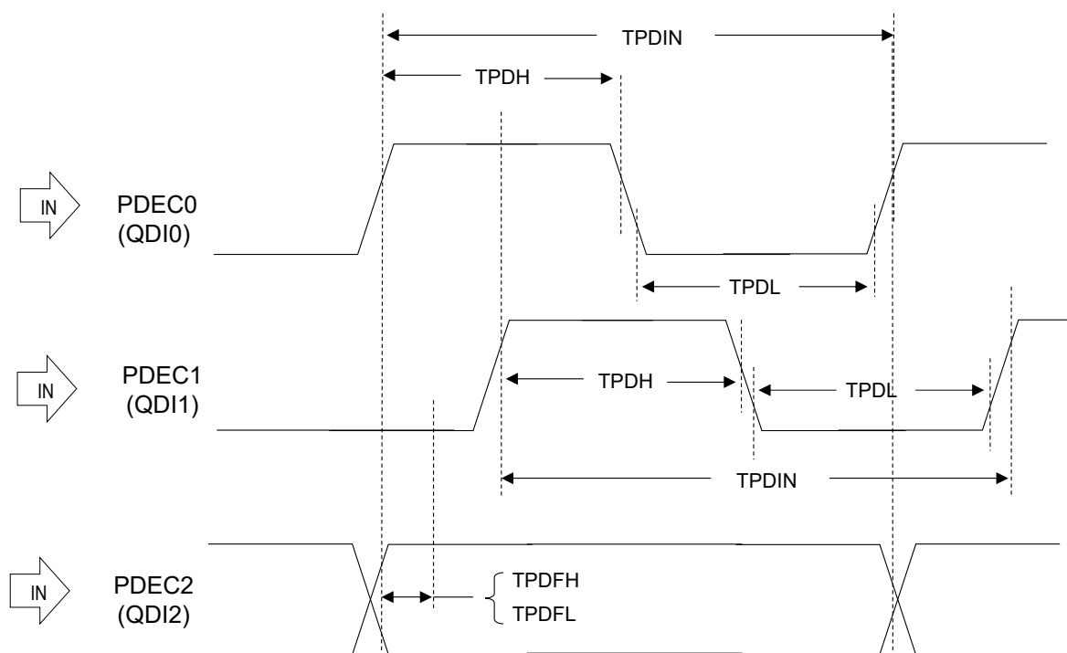
Figure 46-21. Quadrature Encoder QDI[0]/QDI[1] Input Characteristics
