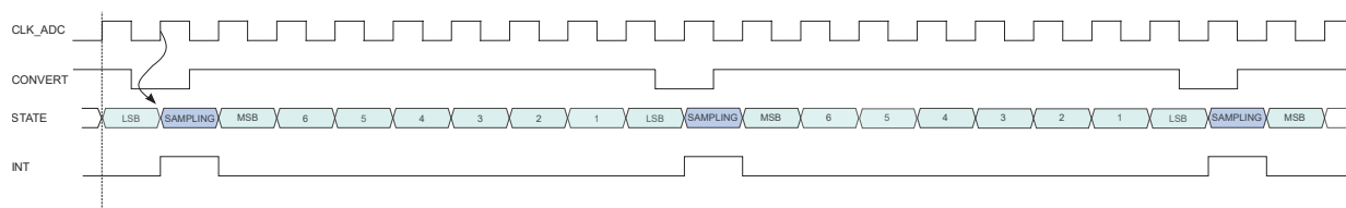
Figure 37-7. ADC Timing for Free Running in 8-bit Resolution
