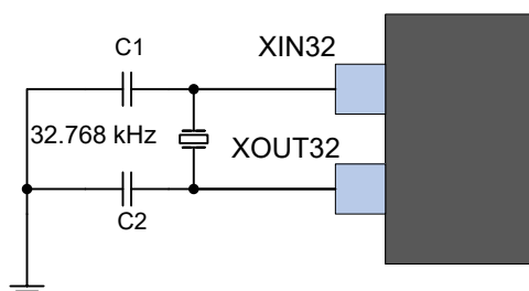
Figure 49-10. 32.768 kHz Crystal Oscillator with Load Capacitor
