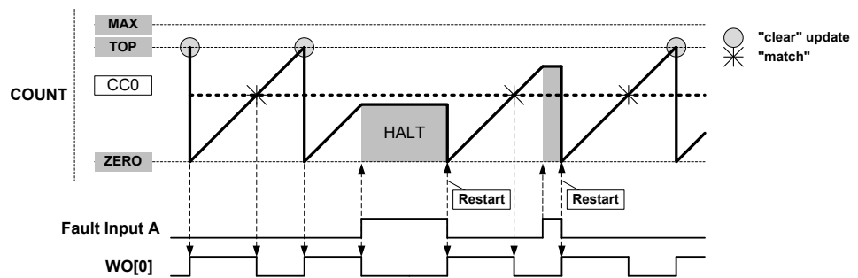
Figure 35-33. Waveform Generation with Fault Qualification, Halt, and Restart Actions
