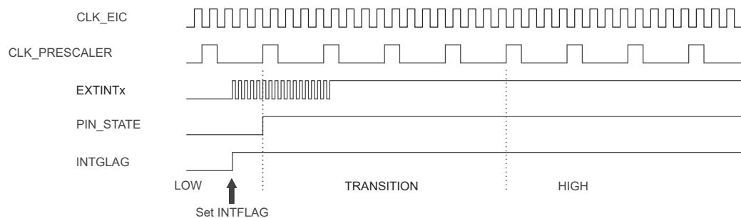
Figure 25-4. EXTINT Pin Asynchronous Debouncing (Rising Edge)
