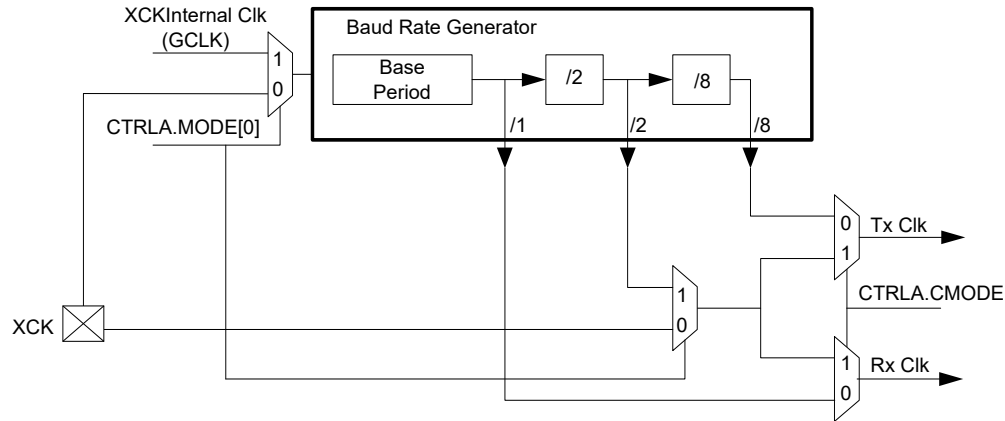
Figure 30-3. Clock Generation
