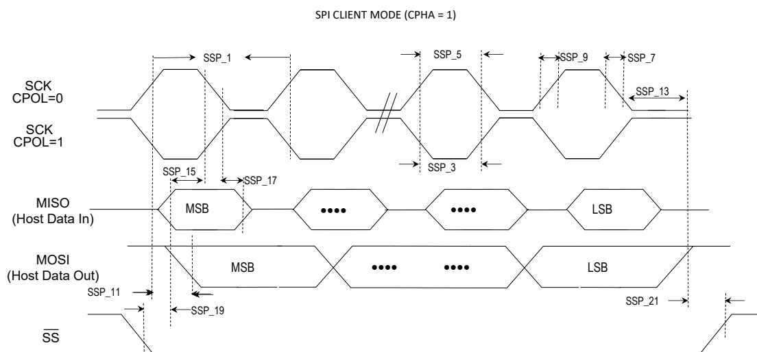
Figure 47-7. SPIx Client Module CPHA = 1 Timing Diagram
