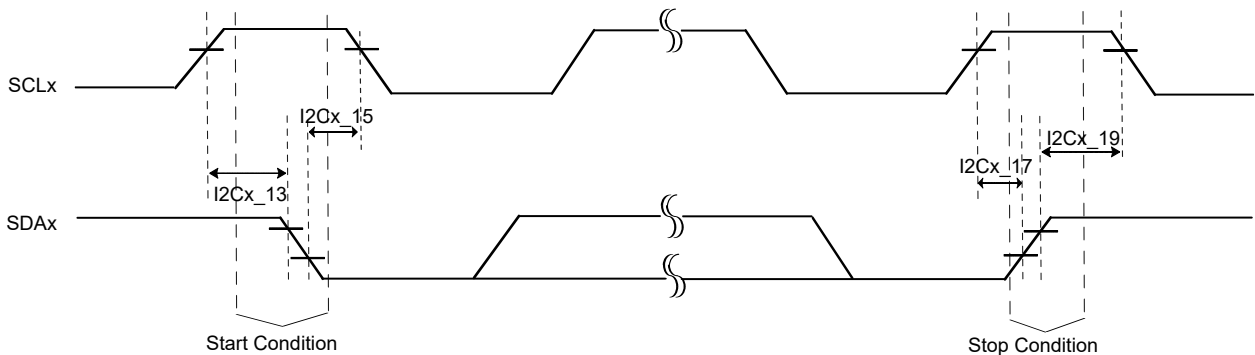
Figure 46-13. SERCOM I 2 C Start/Stop Bits Client Mode Timing Diagram
