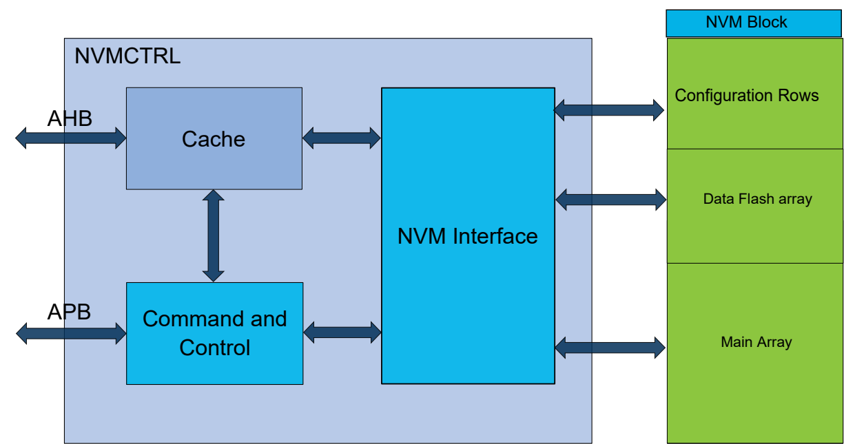
Figure 26-1. Block Diagram
