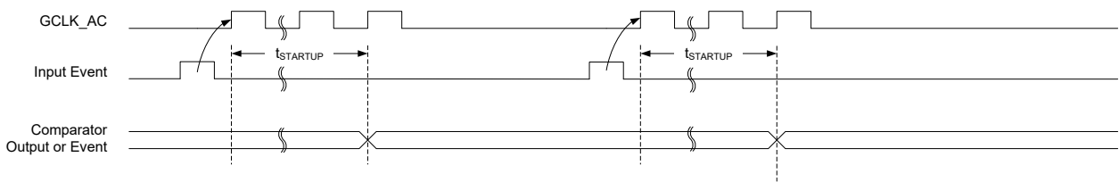
Figure 38-11. Single-Shot SleepWalking
