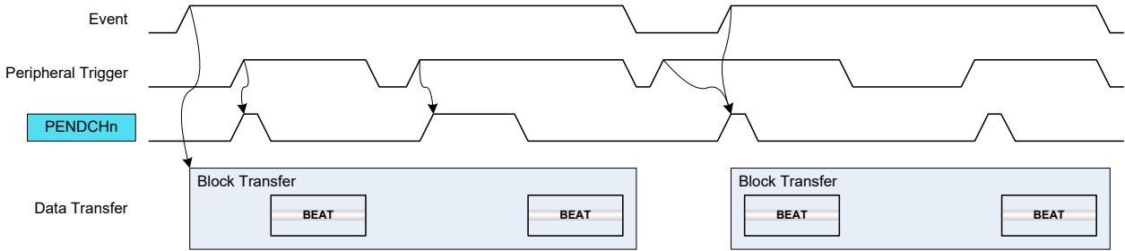
Figure 24-14. Conditional Block Transfer with Beat Peripheral Triggers
