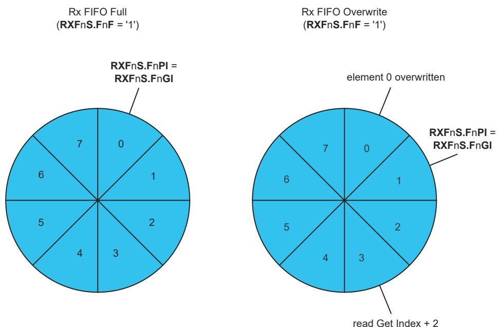
Figure 33-8. Rx FIFO Overflow Handling
