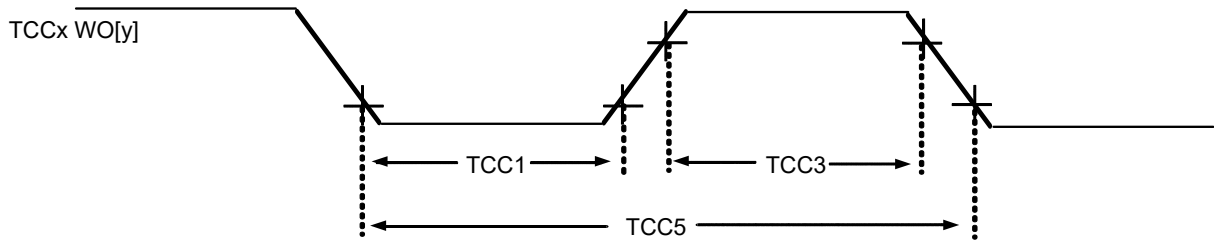
Figure 46-19. TCCx Timer Compare Output Timing Diagrams
