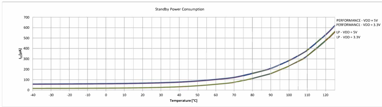
Figure 46-4. Power Consumption at VDD = VDDIO = 3.3 / 5.0V Over Temperature in Standby Sleep Mode with RTC
