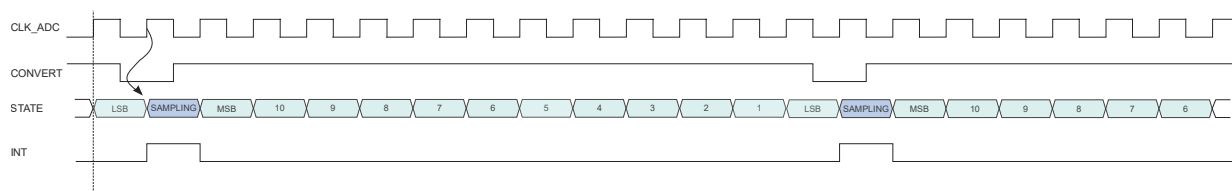
Figure 37-6. ADC Timing for Free Running in 12-bit Resolution
