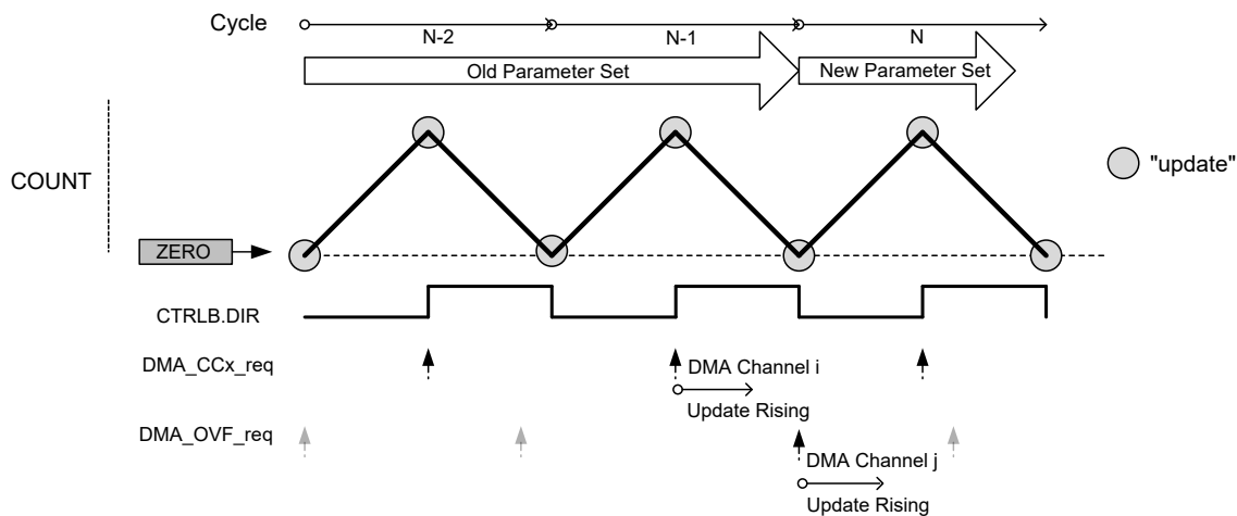
Figure 35-41. DMA Triggers in DSBOTH Operation Mode and Circular Buffer Enabled
