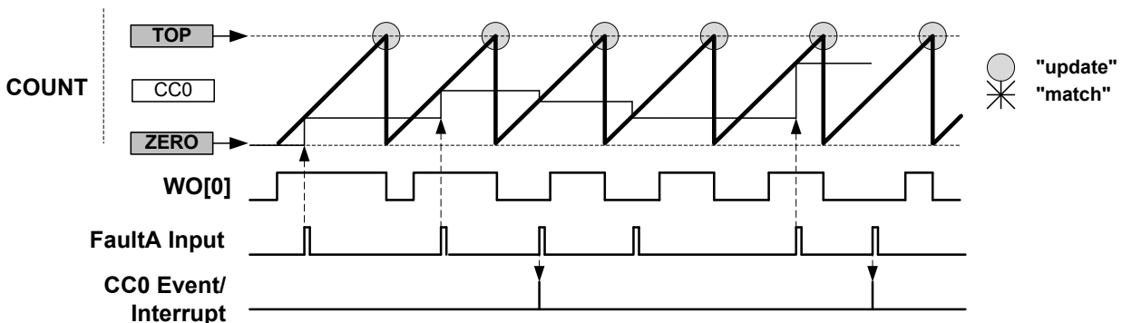
Figure 35-31. Capture Action "DERIVO"
