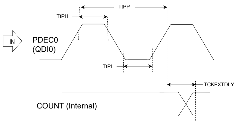
Figure 46-20. PDEC Timing Diagrams Counter Mode
