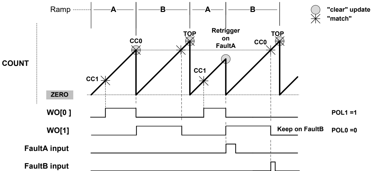
Figure 35-23. Critical Swapped RAMP2 Operation
