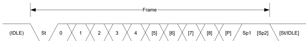
Figure 30-2. Frame Formats
