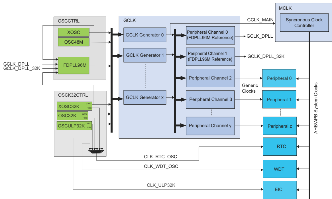
Figure 9-1. Clock Distribution
