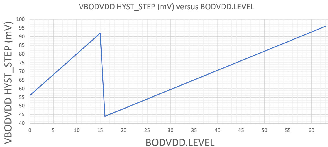
Figure 46-1. VBODVDDHYST_STEP Graph
