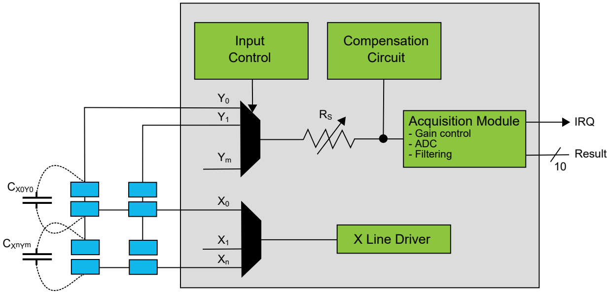
Figure 40-1. PTC Block Diagram Mutual Capacitance
