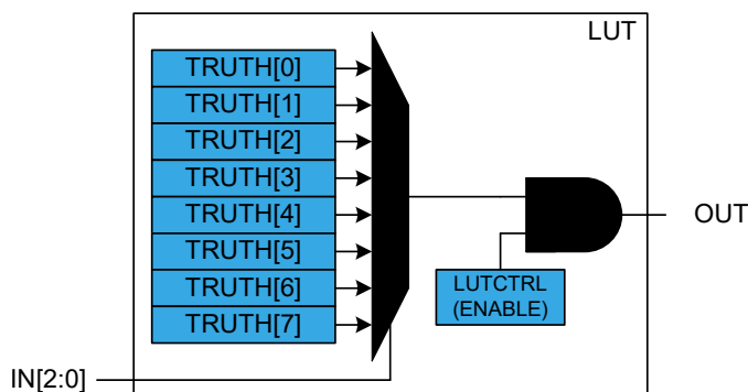
Figure 36-2. Truth Table Output Value Selection
