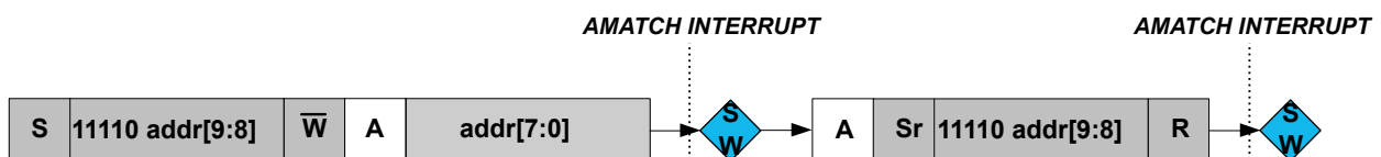
Figure 32-12. 10-bit Addressing
