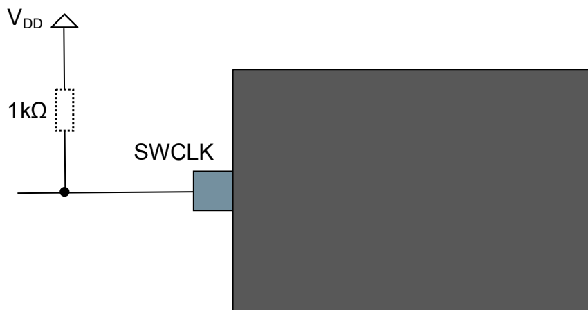
Figure 49-11. SWCLK Circuit Connections
