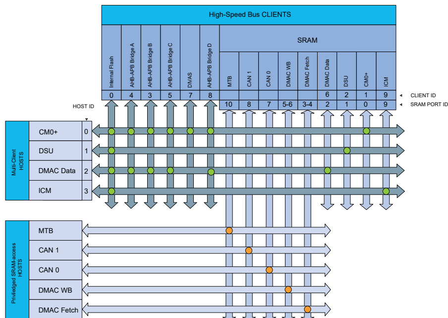
Figure 11-1. Host-Client Relation High-Speed Bus Matrix
