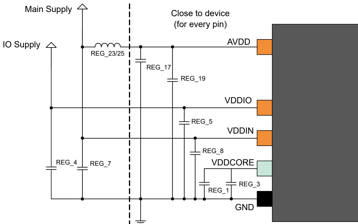
Figure 49-2. Dual Power Supply Schematic
