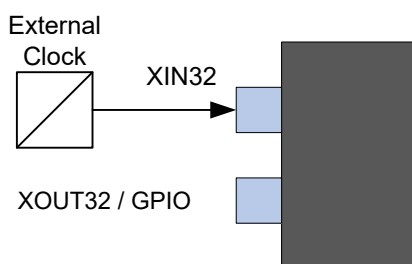
Figure 49-8. 32.768 kHz External Clock Source Schematic
