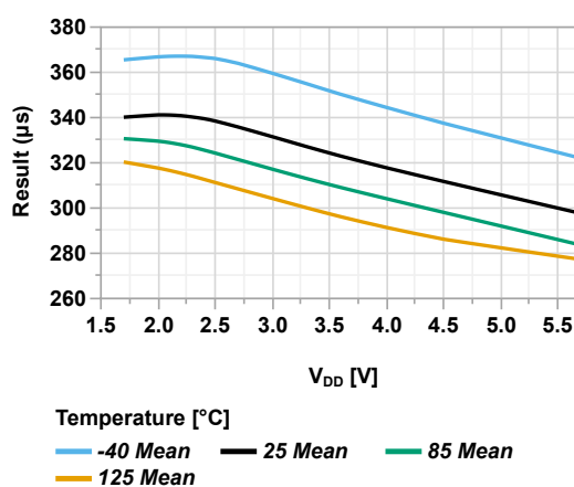
Figure 44-73. LFO Oscillator Start-Up Time vs V_{DD}
