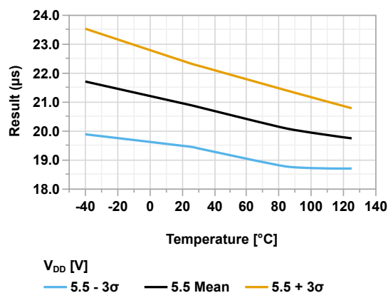
Figure 44-68. HFO Oscillator Start-Up Time vs Temperature ( V_{DD} = 5.5V )
