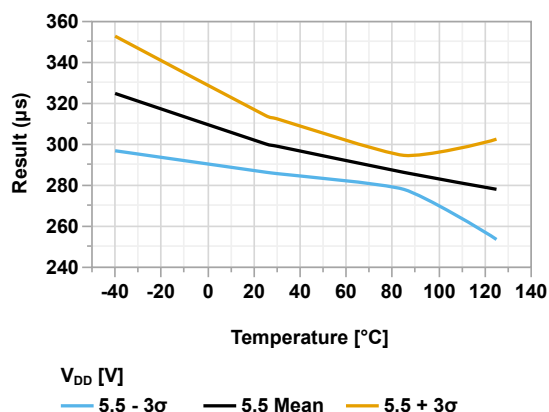
Figure 44-72. LFO Oscillator Start-Up Time vs Temperature ( V_{DD} = 5.5V )
