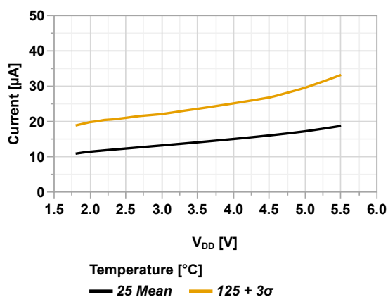
Figure 44-15. I_{DD} vs V_{DD} (XT = 1 MHz, PMDx = 0x00)
