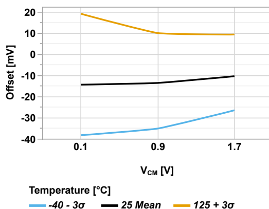
Figure 44-122. Input Offset vs Common-Mode Voltage ( V_{DD} = 1.8V )
