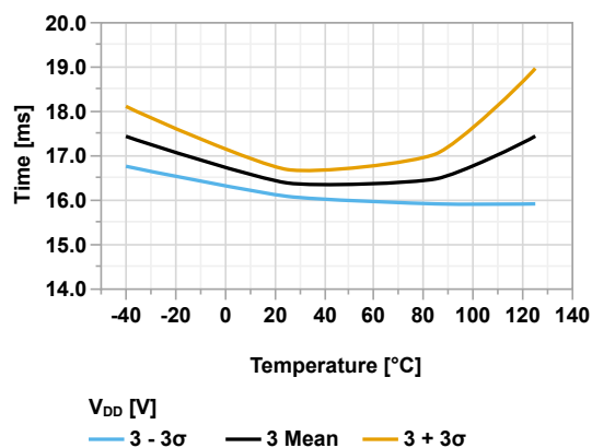
Figure 44-88. WDT Time-out Period vs Temperature ( V_{DD} = 3.0V )
