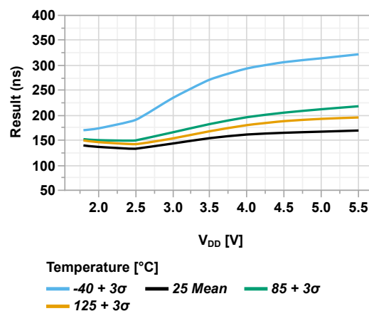
Figure 44-131. Falling Edge Response Time vs V_{DD} (CxSP = '0', CPON = 'b01')
