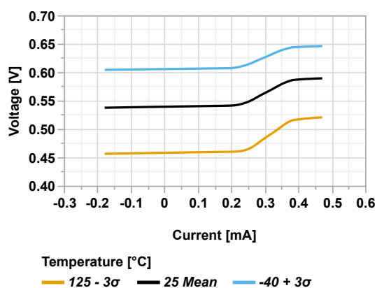
Figure 44-151. ZCD Pin Voltage vs Current, ( V_{DD} = 3.0V )
