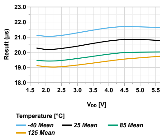
Figure 44-69. HFO Oscillator Start-Up Time vs V_{DD}
