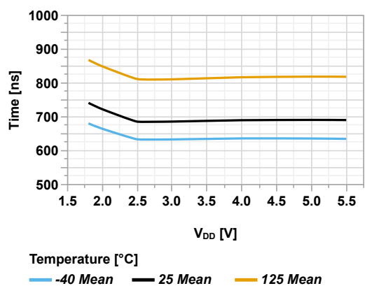
Figure 44-156. ZCD Falling-Edge Response Time vs V_{DD} (Mean Values)
