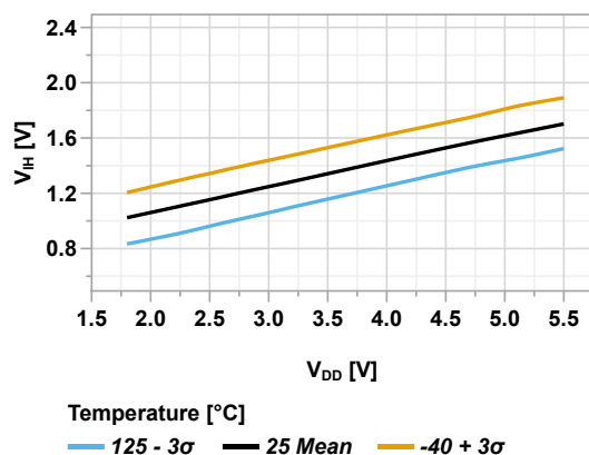
Figure 44-52. Input Pin with SMBus 2.0 Minimum V_{IH} vs V_{DD}
