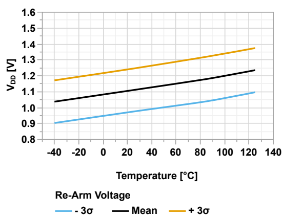
Figure 44-83. POR Rearm Voltage vs Temperature
