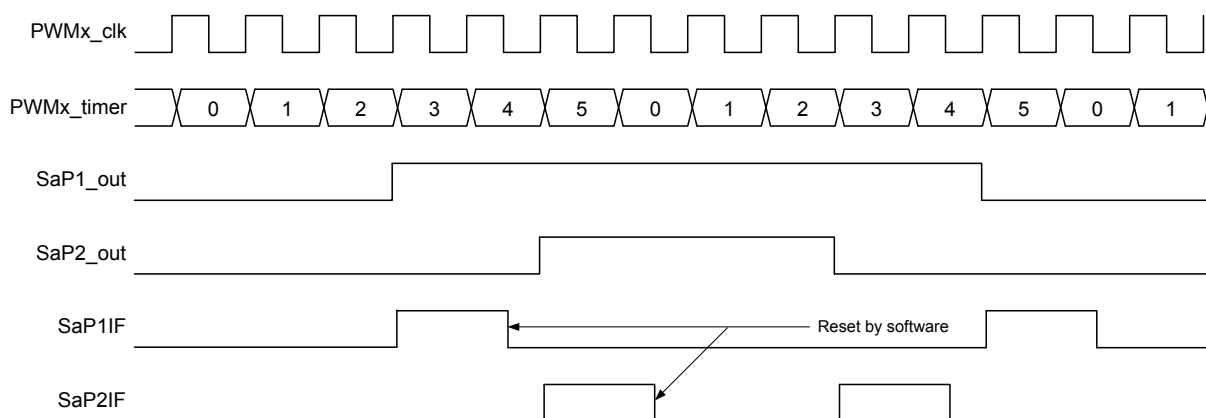
Figure 29-6. Center-Aligned Timing Diagram
