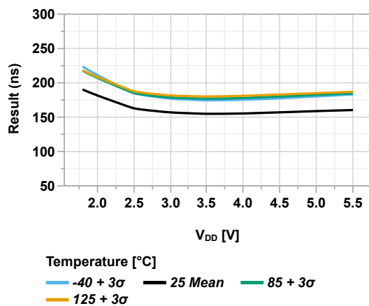
Figure 44-126. Rising Edge Response Time vs V_{DD} (CxSP = '1', CPON = 'b01')
