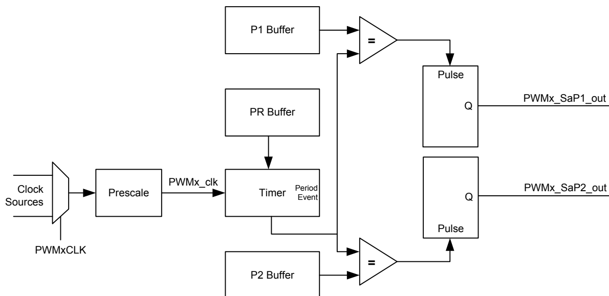
Figure 29-9. Pulsed Compare Block Diagram
