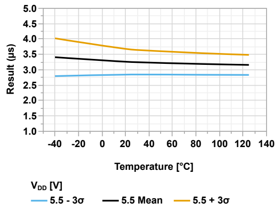
Figure 44-117. DAC Settling Time vs. Temperature ( V_{DD} = 5.5V )
