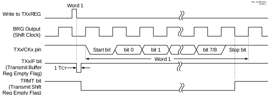
Figure 32-10. Synchronous Transmission
