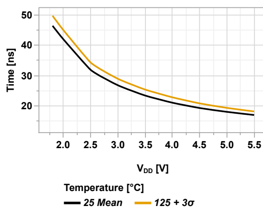
Figure 44-45. Rise Time vs V_{DD} (SLRxn = '0', T_A = 125^\circ C )
