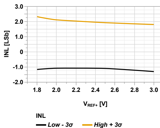
Figure 44-98. ADC INL vs V_{REF+} (Single-Ended Mode, T_{AD} = 1 \mu s , V_{DD} = 3.0V , T_A = 125^\circ C , CPON = 'b11')
