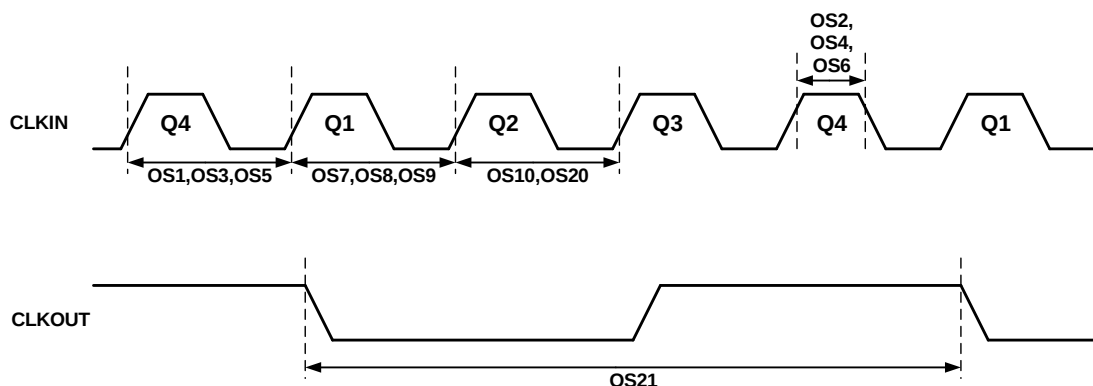
Figure 43-4. Clock Timing
