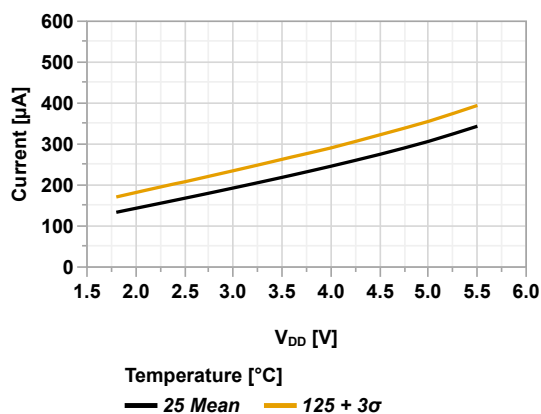
Figure 44-17. I_{DD} vs V_{DD} (XT = 4 MHz, PMDx = 0x00)
