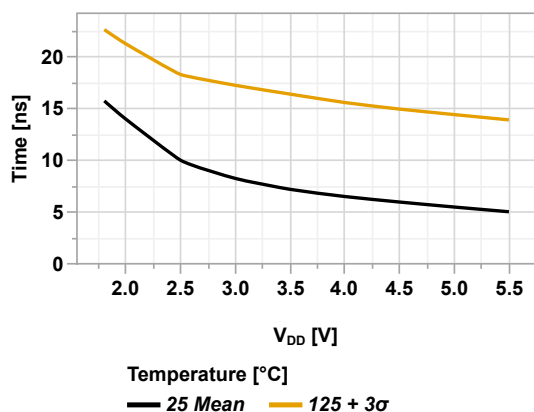
Figure 44-46. Fall Time vs V_{DD} (SLRxn = '1', T_A = 125^\circ\text{C} )
