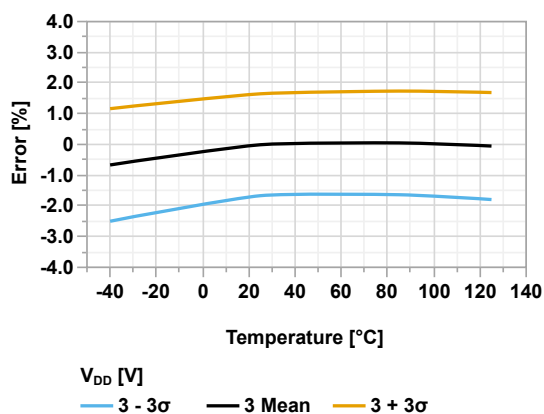
Figure 44-145. CDAFVR Voltage Error vs Temperature ( V_{DD} = 3.0V , V_{REF} = 2.048V )
