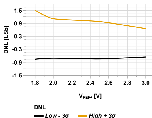
Figure 44-94. ADC DNL vs V_{REF+} (Single-Ended Mode, T_{AD} = 1 \mu s , V_{DD} = 3.0V , T_A = 125^\circ C , CPON = 'b11')
