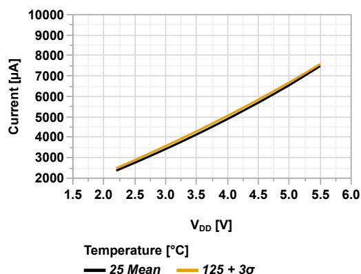
Figure 44-22. I_{DD} vs V_{DD} (ECL = 32 kHz, PMDx = 0xFF)
