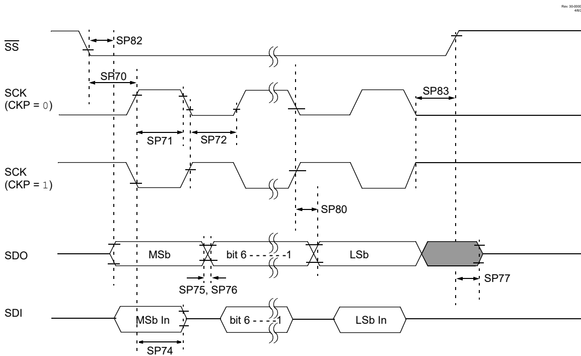
Figure 43-18. SPI Client Mode Timing (CKE = 1)
