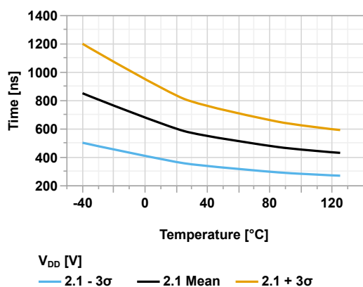
Figure 44-81. BOR Minimum Pulse Width for Response vs Temperature
