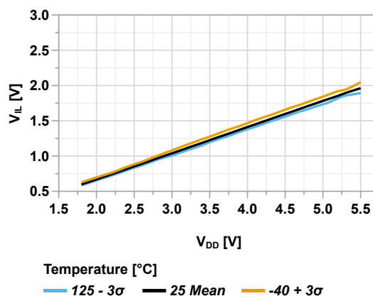
Figure 44-57. Input Pin with I 2 C Trigger Maximum V_{IL} vs V_{DD}
