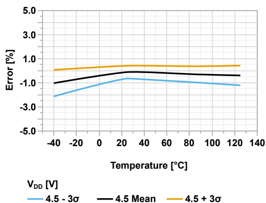
Figure 44-141. ADFVR Voltage Error vs Temperature ( V_{DD} = 4.5V , V_{REF} = 4.096V )
