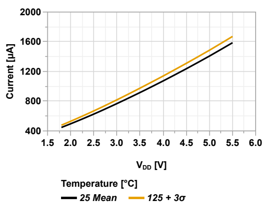
Figure 44-28. I_{DD} vs V_{DD} (Doze Mode, HFINTOSC = 16 MHz, PMDx = 0xFF)
