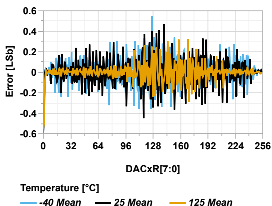
Figure 44-105. DAC DNL vs. DAC Code ( V_{REF} = V_{DD} = 5.0V )
