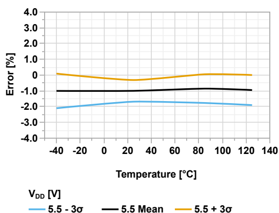
Figure 44-137. ADFVR Voltage Error vs Temperature ( V_{DD} = 5.5V , V_{REF} = 1.024V )
