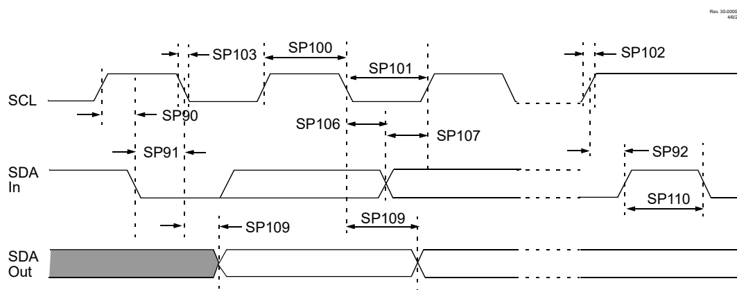
Figure 43-20. I 2 C Bus Data Timing
