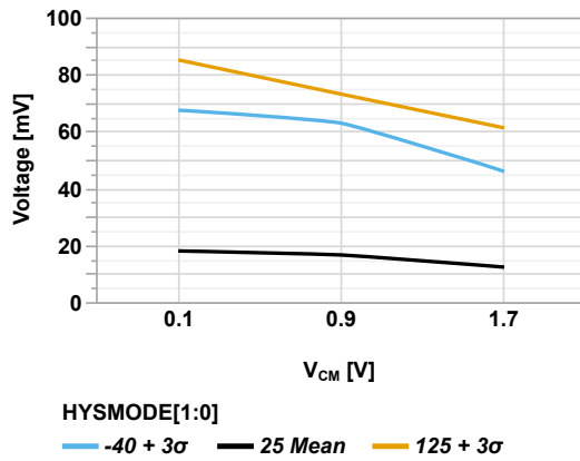
Figure 44-118. Input Hysteresis vs Common-Mode Voltage ( V_{DD} = 1.8V )
