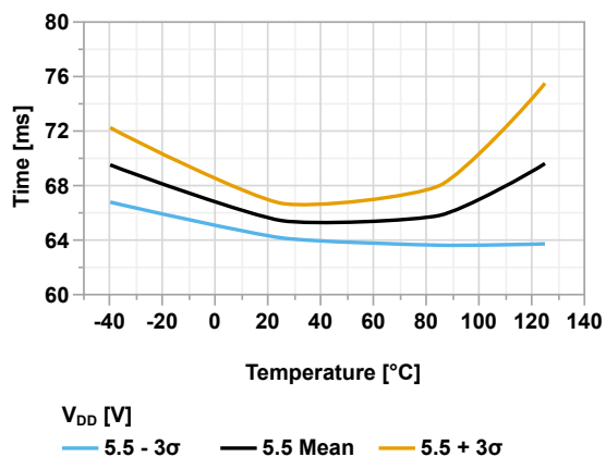
Figure 44-86. Start-Up Time vs Temperature (PWRTS = 'b10, V_{DD} = 5.5V )
