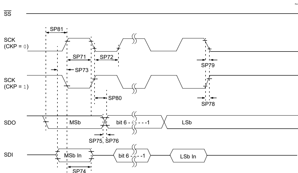
Figure 43-16. SPI Host Mode Timing (CKE = 1, SMP = 1)
