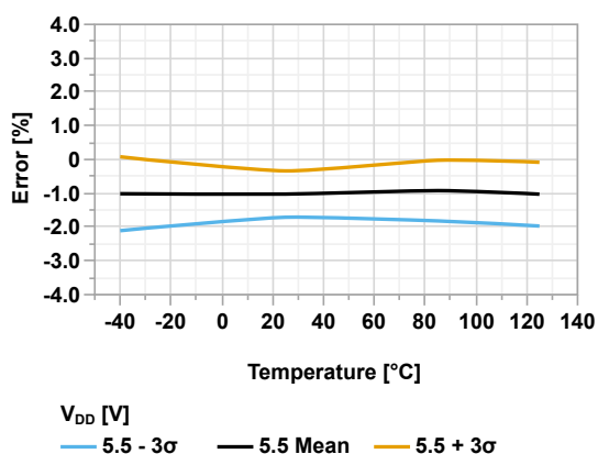
Figure 44-142. ADFVR Voltage Error vs Temperature ( V_{DD} = 5.5V , V_{REF} = 4.096V )
