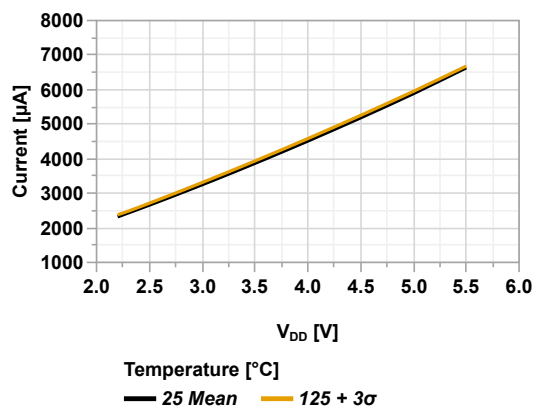
Figure 44-12. I_{DD} vs V_{DD} (HFINTOSC = 32 MHz, PMDx = 0xFF)
