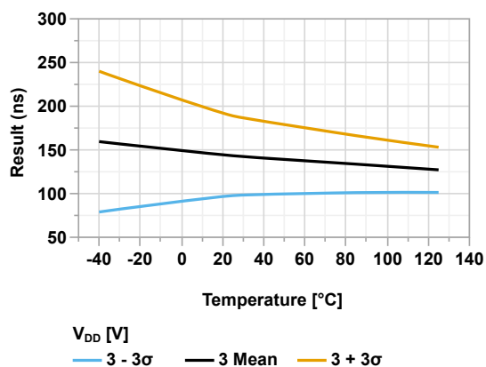
Figure 44-133. Falling Edge Response Time vs Temperature (CxSP = '0', CPON = 'b01', V_{DD} = 3.0V)
