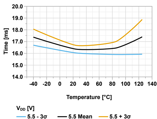
Figure 44-89. WDT Time-out Period vs Temperature ( V_{DD} = 5.5V )
