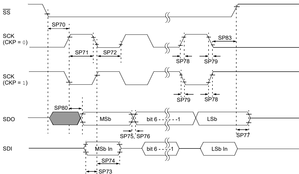
Figure 43-17. SPI Client Mode Timing (CKE = 0)
