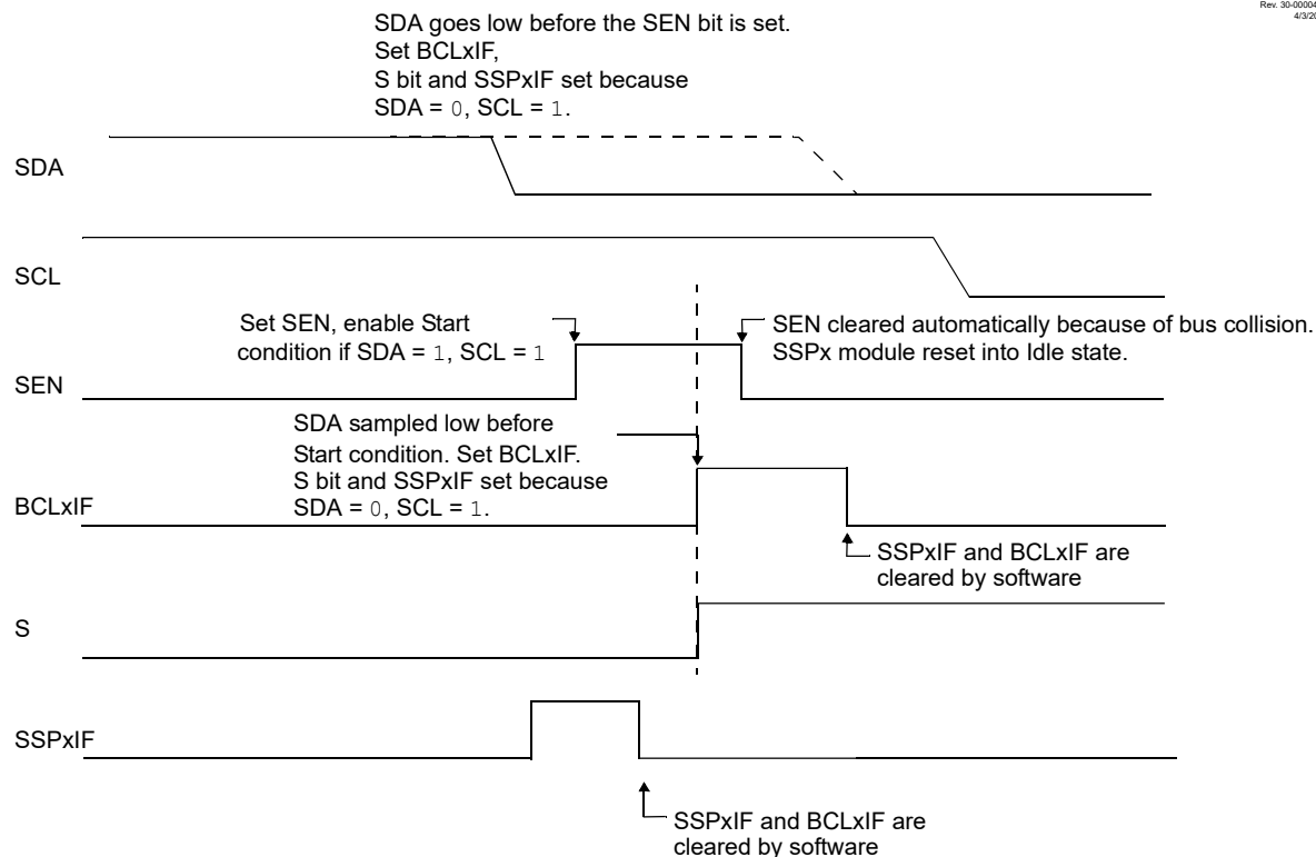
Figure 31-34. Bus Collision During Start Condition (SDA Only)
