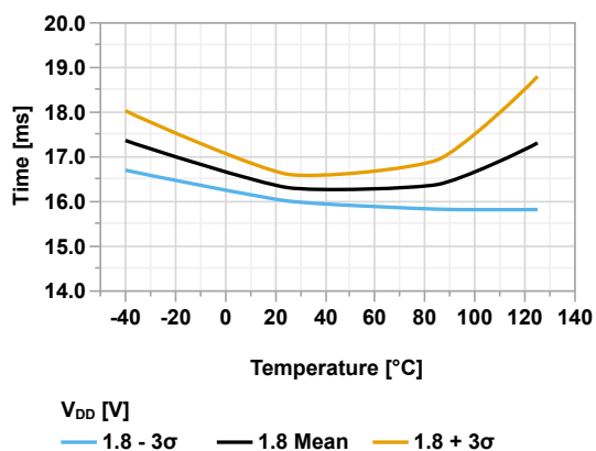
Figure 44-87. WDT Time-out Period vs Temperature ( V_{DD} = 1.8V )
