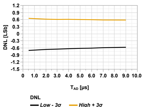
Figure 44-93. ADC DNL vs T_{AD} (Single-Ended Mode, V_{REF+} = V_{DD} = 3.0V , T_A = 125^\circ C , CPON = 'b11')
