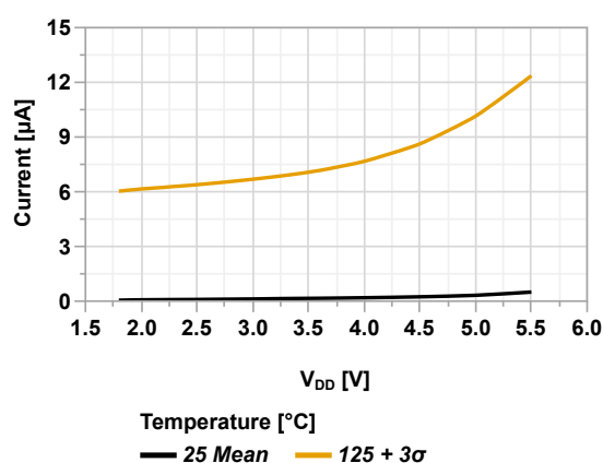
Figure 44-42. I_{PD} FVR Buffer 1 (ADC) vs V_{DD}
