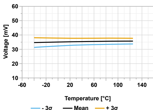
Figure 44-79. Low-Power Brown-out Reset Threshold Level vs Temperature
