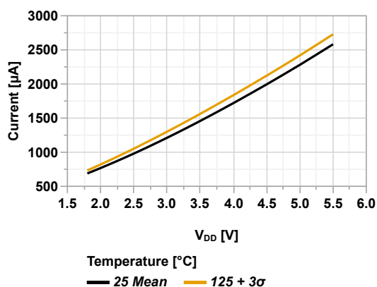
Figure 44-29. I_{DD} vs V_{DD} (Idle Mode, HFINTOSC = 16 MHz, PMDx = 0x00)
