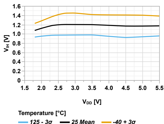
Figure 44-56. Input Pin with I 2 C Trigger Minimum V_{IH} vs V_{DD}
