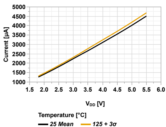
Figure 44-11. I_{DD} vs V_{DD} (HFINTOSC = 32 MHz, PMDx = 0x00)
