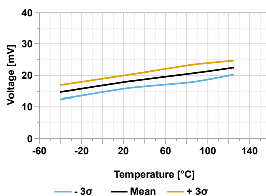
Figure 44-80. Low-Power Brown-out Reset Hysteresis vs Temperature
