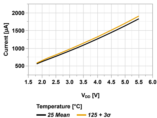
Figure 44-8. I_{DD} vs V_{DD} (HFINTOSC = 8 MHz, PMDx = 0xFF)
