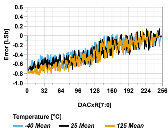
Figure 44-111. DAC INL vs. DAC Code ( V_{REF} = V_{DD} = 5.5V )
