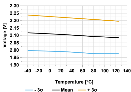
Figure 44-79. Low-Power Brown-out Reset Threshold Level vs Temperature
