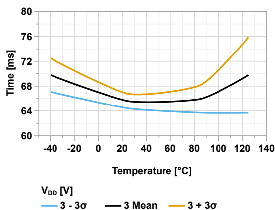
Figure 44-85. Start-Up Time vs Temperature (PWRTS = 'b10, V_{DD} = 3.0V )
