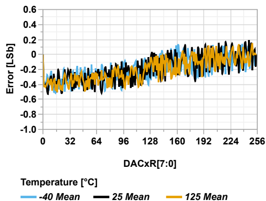
Figure 44-111. DAC INL vs. DAC Code ( V_{REF} = V_{DD} = 5.5V )
