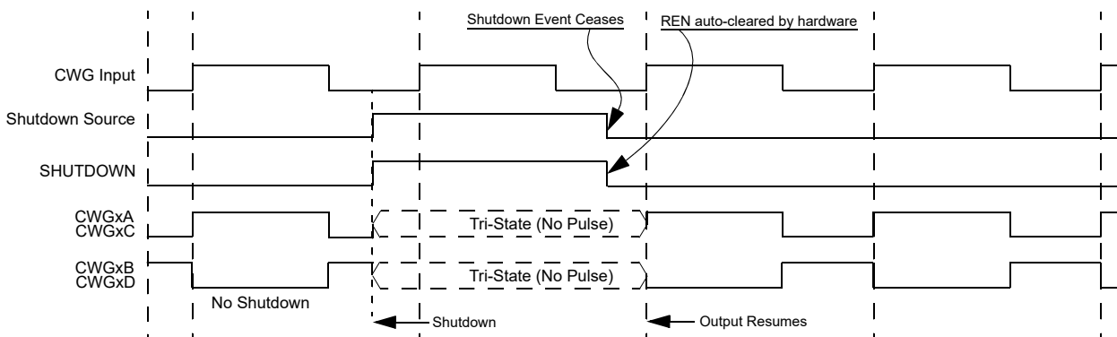
Figure 26-16. Shutdown Functionality, Auto-Restart Enabled (REN = 1, LSAC = 'b01, LSB0 = 'b01)
