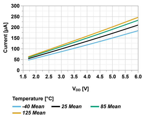
Figure 44-65. Weak Pull-Up Current vs V_{DD} (Mean Values)
