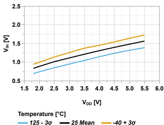
Figure 44-48. Input Pin with TTL Buffer Minimum V_{IH} vs V_{DD}
