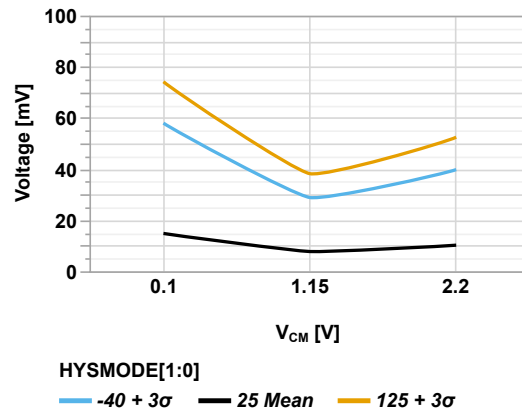
Figure 44-119. Input Hysteresis vs Common-Mode Voltage ( V_{DD} = 2.3V )
