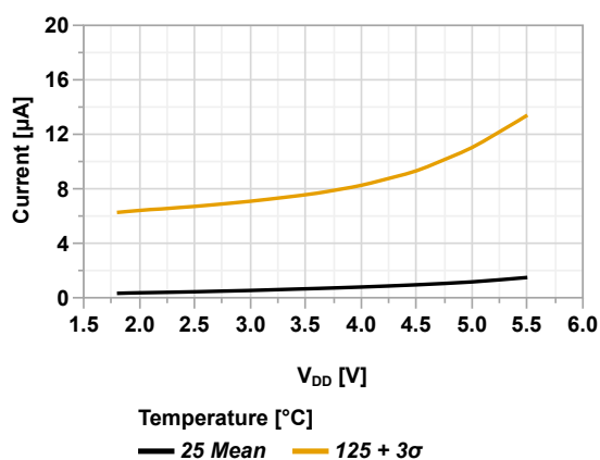
Figure 44-35. I_{PD} WWDT vs V_{DD}
