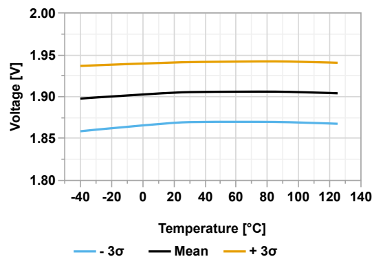
Figure 44-75. Brown-out Reset Voltage Threshold Level vs Temperature (BORV = '1') (BORV = '1')
