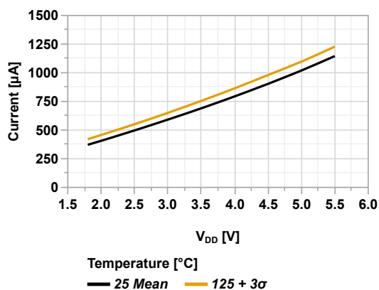
Figure 44-17. I_{DD} vs V_{DD} (XT = 4 MHz, PMDx = 0x00)
