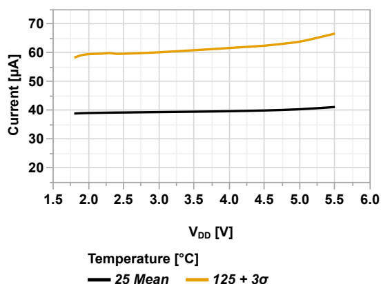
Figure 44-43. I_{PD} FVR Buffer 2 (DAC) vs V_{DD}
