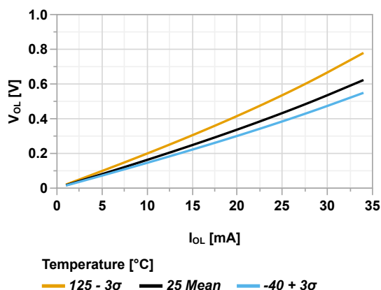
Figure 44-62. Output Pin Maximum V_{OL} vs Current ( V_{DD} = 3.0V )
