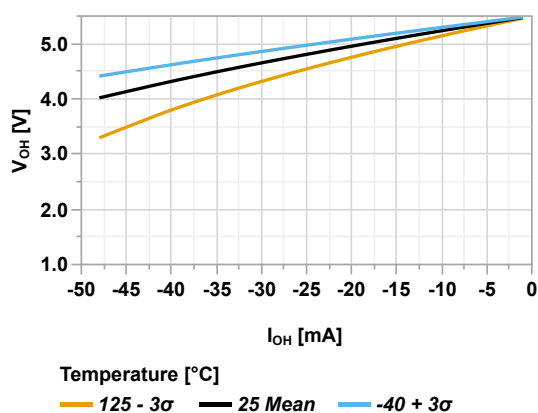
Figure 44-60. Output Pin Minimum V_{OH} vs Current ( V_{DD} = 5.5V )
