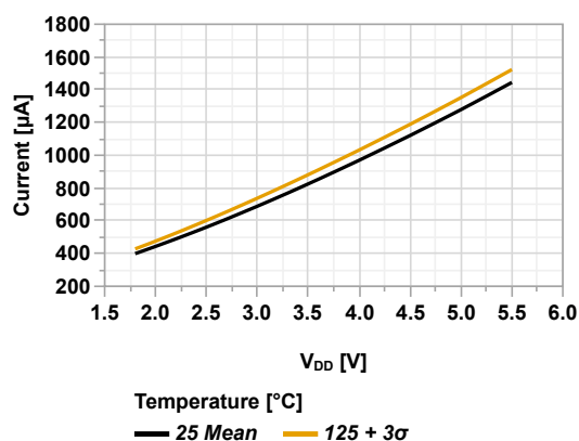
Figure 44-30. I_{DD} vs V_{DD} (Idle Mode, HFINTOSC = 16 MHz, PMDx = 0xFF)
