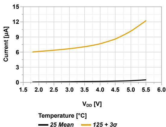
Figure 44-31. I_{PD} Base vs V_{DD}
