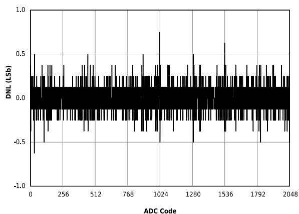
Figure 44-91. ADC DNL vs ADC Code (Single-Ended Mode, V_{DD} = 3.0V , T_{AD} = 1 \mu s )
