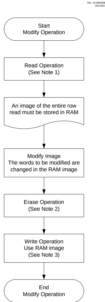
Figure 15-6. Program Flash Memory Modify Sequence
