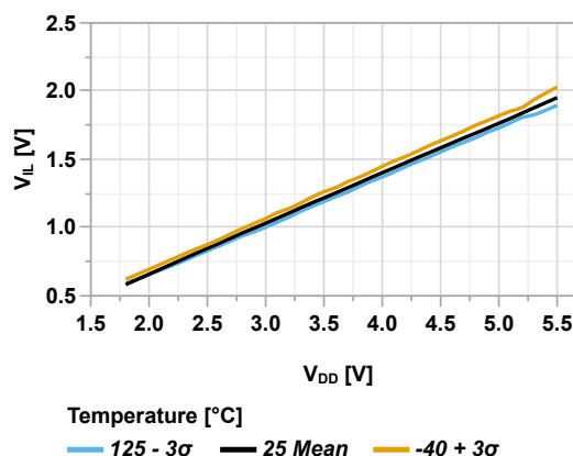
Figure 44-53. Input Pin with SMBus 2.0 Maximum V_{IL} vs V_{DD}
