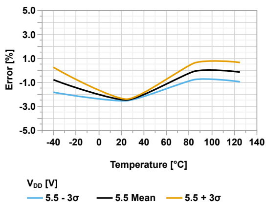
Figure 44-142. ADFVR Voltage Error vs Temperature ( V_{DD} = 5.5V , V_{REF} = 4.096V )
