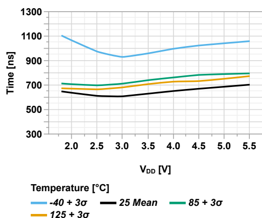
Figure 44-90. Minimum Reset Pulse-Width vs V_{DD}
