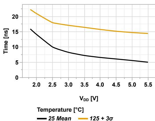
Figure 44-44. Rise Time vs V_{DD} (SLRxn = '1', T_A = 125^\circ C )
