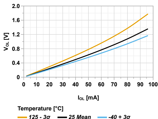
Figure 44-63. Output Pin Maximum V_{OL} vs Current ( V_{DD} = 5.5V )
