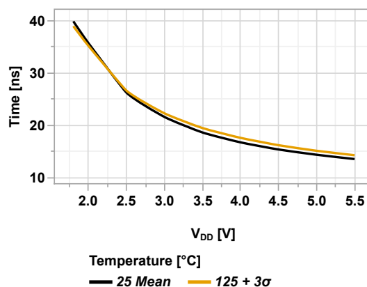
Figure 44-47. Fall Time vs V_{DD} (SLRxn = '0', T_A = 125^\circ\text{C} )
