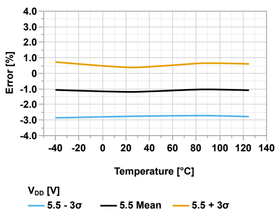
Figure 44-146. CDAFVR Voltage Error vs Temperature ( V_{DD} = 5.5V , V_{REF} = 2.048V )
