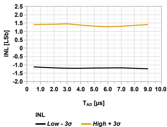
Figure 44-97. ADC INL vs T_{AD} (Single-Ended Mode, V_{REF+} = V_{DD} = 3.0V , T_A = 125^\circ C , CPON = 'b11')
