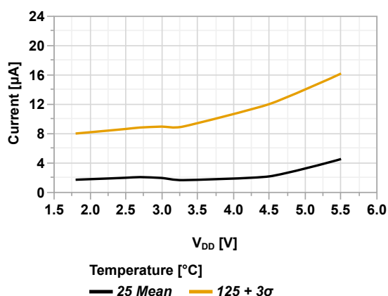
Figure 44-39. I_{PD} Comparator (High-Power Mode) vs V_{DD}
