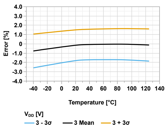
Figure 44-145. CDAFVR Voltage Error vs Temperature ( V_{DD} = 3.0V , V_{REF} = 2.048V )
