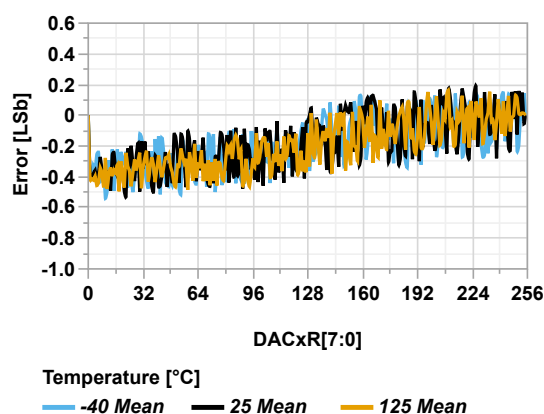
Figure 44-112. DAC INL vs. Temperature ( V_{REF} = V_{DD} = 3.0V )
