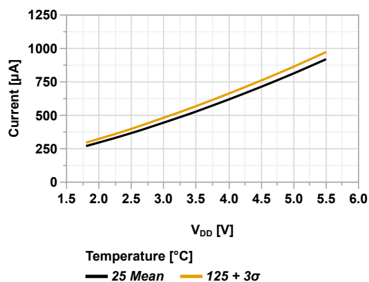
Figure 44-3. I_{DD} vs V_{DD} (HFINTOSC = 2 MHz, PMDx = 0x00)
