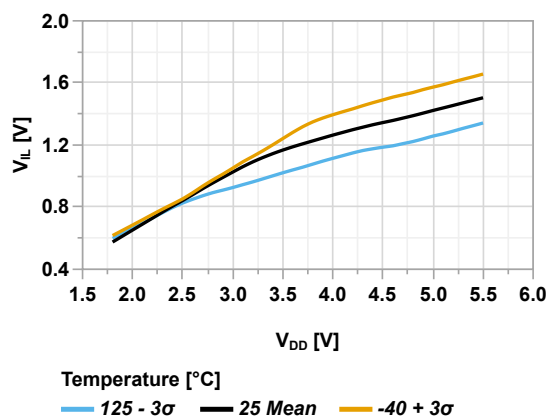
Figure 44-49. Input Pin with TTL Buffer Maximum V_{IL} vs V_{DD}
