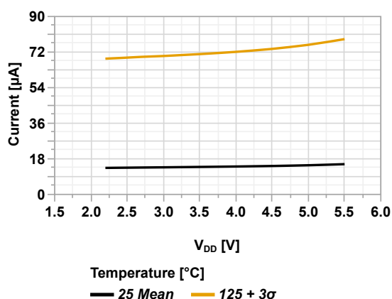
Figure 44-33. I_{PD} Brown-out Reset (BOR) vs V_{DD}
