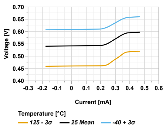
Figure 44-152. ZCD Pin Voltage vs Current, ( V_{DD} = 5.5V )
