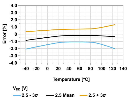
Figure 44-138. ADFVR Voltage Error vs Temperature ( V_{DD} = 2.5V , V_{REF} = 2.048V )
