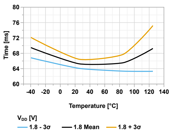
Figure 44-84. Start-Up Time vs Temperature (PWRTS = 'b10, V_{DD} = 1.8V )
