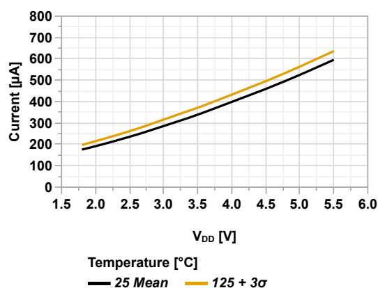
Figure 44-4. I_{DD} vs V_{DD} (HFINTOSC = 2 MHz, PMDx = 0xFF)
