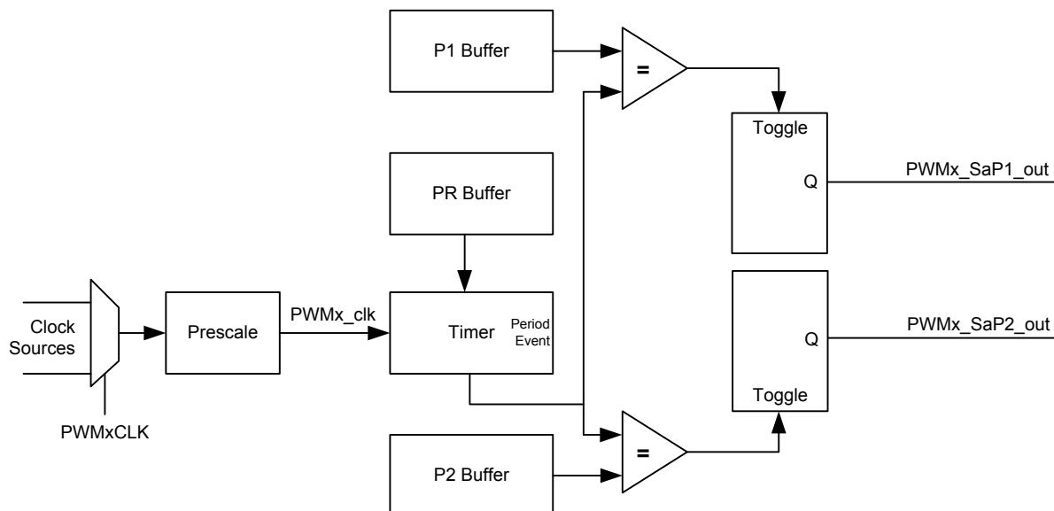
Figure 29-11. Toggled Compare Block Diagram
