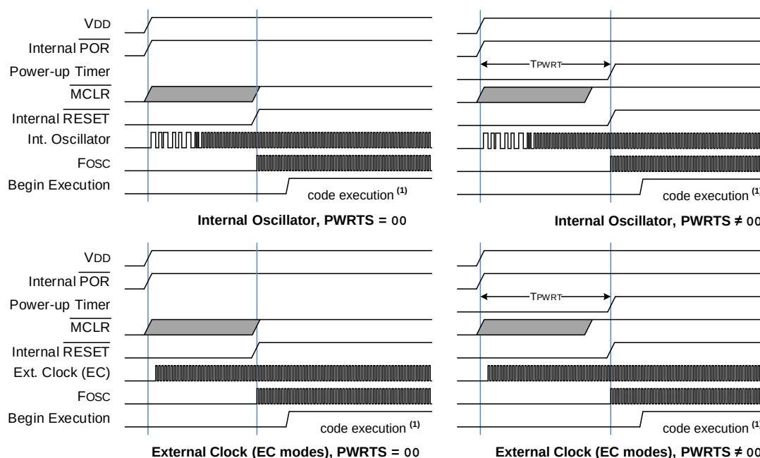
Figure 10-4. Reset Start-Up Sequence
