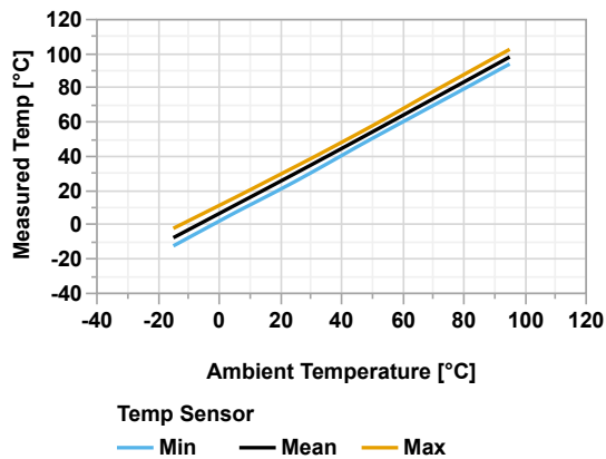
Figure 44-148. TEMPERATURE INDICATOR CHARACTERISTICS ( V_{DD} = 3.0V )
