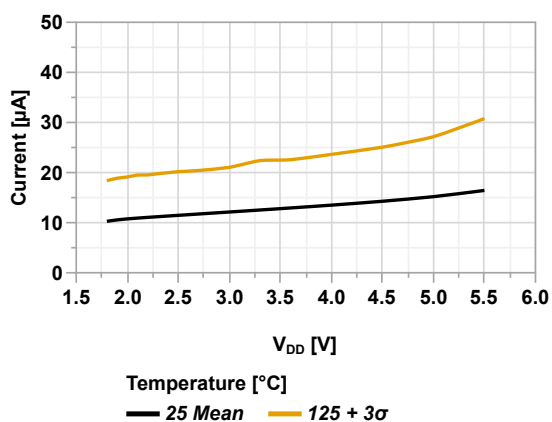
Figure 44-16. I_{DD} vs V_{DD} (XT = 1 MHz, PMDx = 0xFF)
