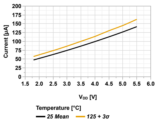
Figure 44-23. I_{DD} vs V_{DD} (ECL = 500 kHz, PMDx = 0x00)
