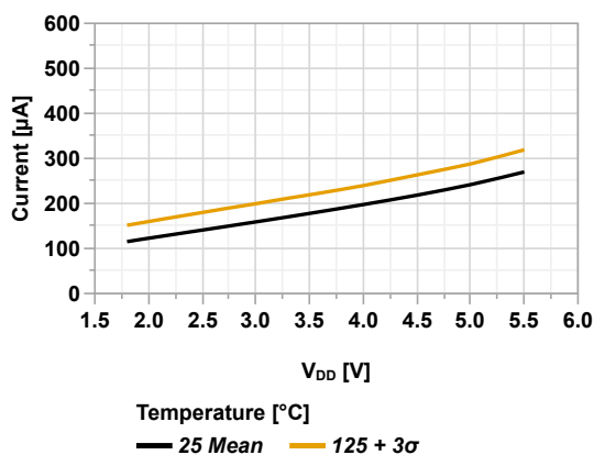
Figure 44-18. I_{DD} vs V_{DD} (XT = 4 MHz, PMDx = 0xFF)
