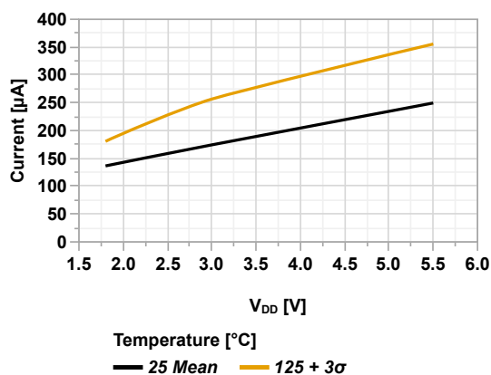
Figure 44-41. I_{PD} ADCRC (Converting) vs V_{DD}
