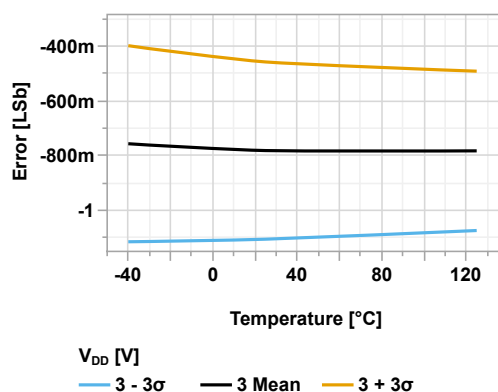
Figure 44-112. DAC INL vs. Temperature ( V_{REF} = V_{DD} = 3.0V )
