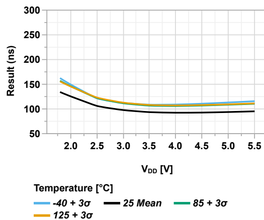
Figure 44-127. Rising Edge Response Time vs V_{DD} (CxSP = '0', CPON = 'b01')
