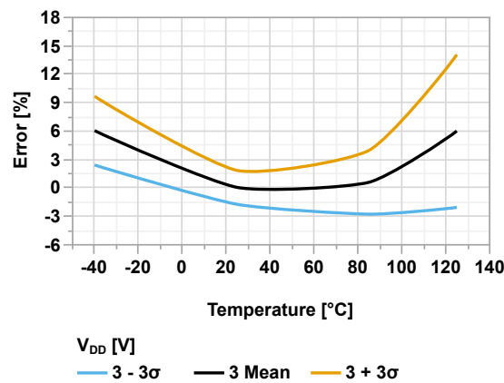
Figure 44-74. LFO Oscillator Error (%) vs Temperature ( V_{DD} = 3.0V )
