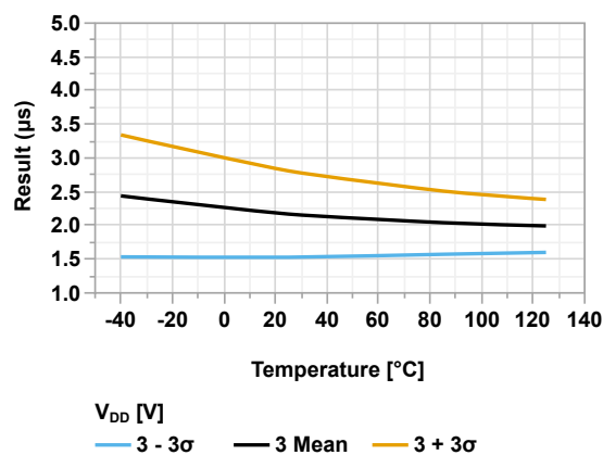
Figure 44-116. DAC Settling Time vs. Temperature ( V_{DD} = 3.0V )
