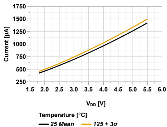
Figure 44-7. I_{DD} vs V_{DD} (HFINTOSC = 8 MHz, PMDx = 0x00)
