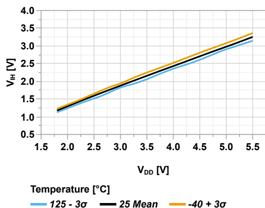
Figure 44-56. Input Pin with I 2 C Trigger Minimum V_{IH} vs V_{DD}
