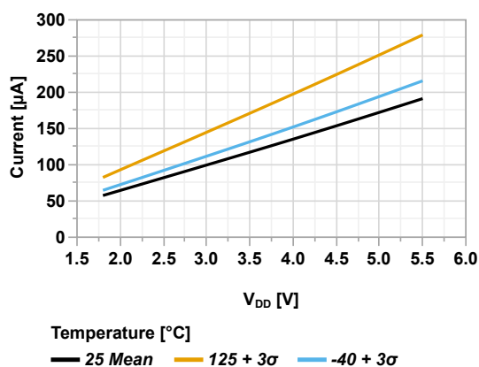
Figure 44-64. Weak Pull-Up Current vs V_{DD}
