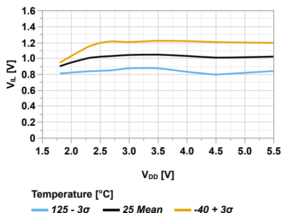
Figure 44-57. Input Pin with I 2 C Trigger Maximum V_{IL} vs V_{DD}
