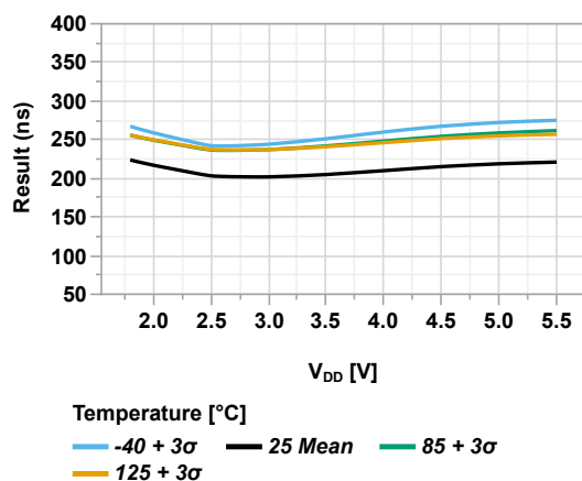
Figure 44-130. Falling Edge Response Time vs V_{DD} (CxSP = '1', CPON = 'b01')
