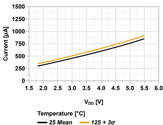
Figure 44-18. I_{DD} vs V_{DD} (XT = 4 MHz, PMDx = 0xFF)
