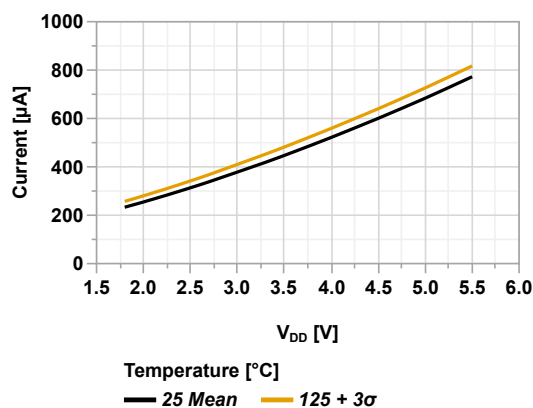
Figure 44-4. I_{DD} vs V_{DD} (HFINTOSC = 2 MHz, PMDx = 0xFF)
