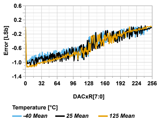
Figure 44-108. DAC INL vs. DAC Code ( V_{REF} = V_{DD} = 2.3V )
