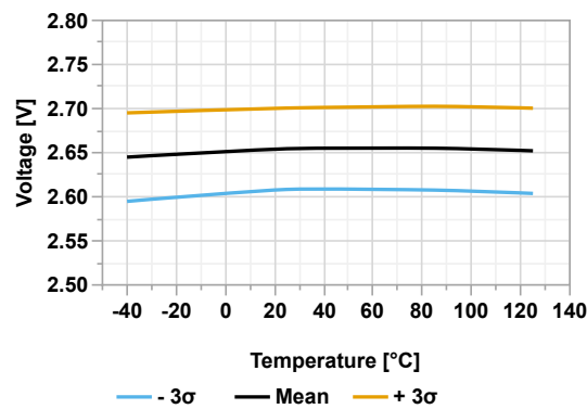
Figure 44-76. Brown-out Reset Voltage Threshold Level vs Temperature (BORV = '0') (BORV = '0')
