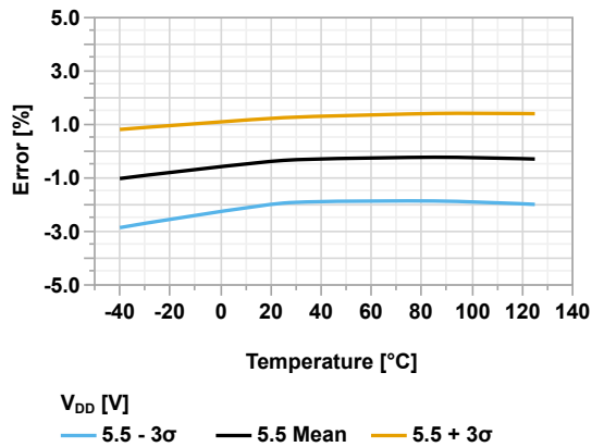
Figure 44-147. CDAFVR Voltage Error vs Temperature ( V_{DD} = 5.5V , V_{REF} = 4.096V )
