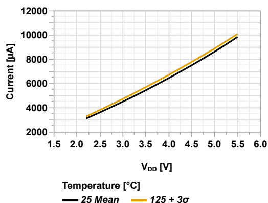
Figure 44-21. I_{DD} vs V_{DD} (ECL = 32 kHz, PMDx = 0x00)
