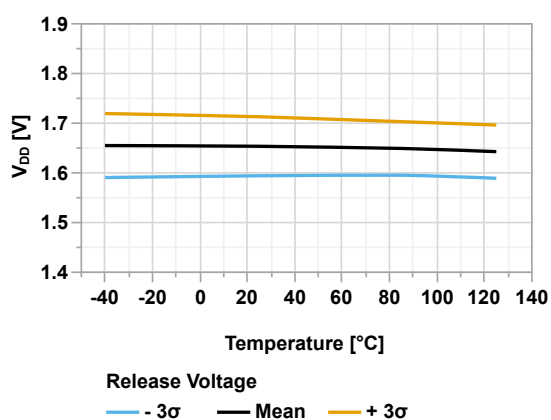
Figure 44-82. POR Release Voltage vs Temperature
