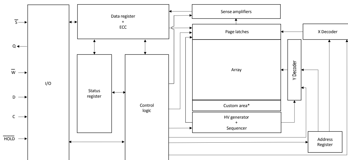
Figure 4. SPI block diagram
