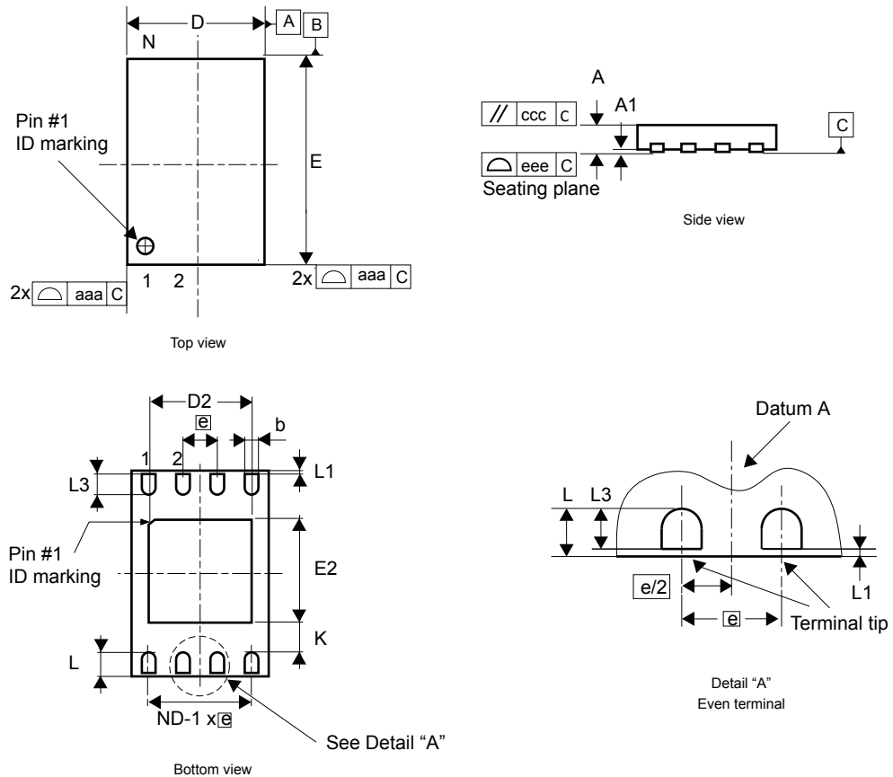
Figure 27. UFDFPN8 - Outline
