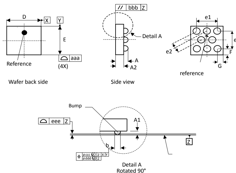
Figure 29. WLCSP8 - Outline
