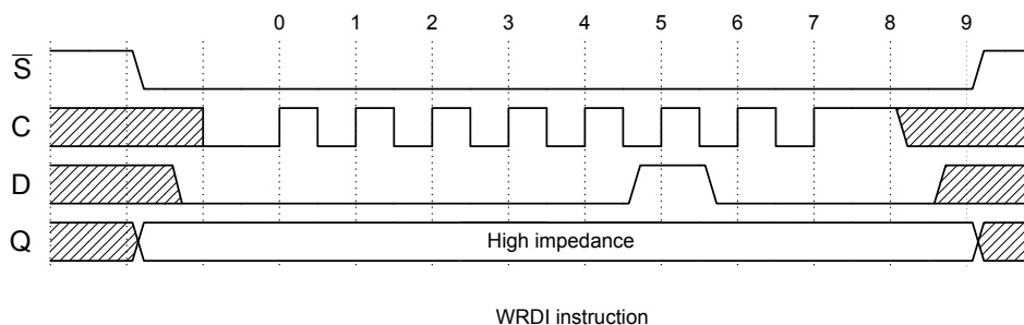
Figure 9. Write disable (WRDI) sequence
