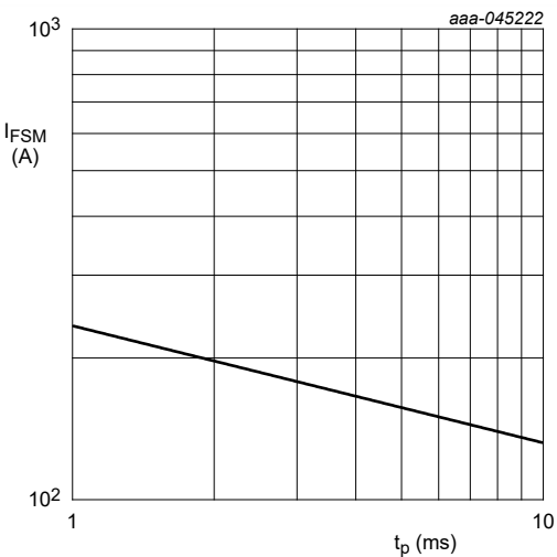
square wave; T_{amb} = 25^\circ\text{C}
