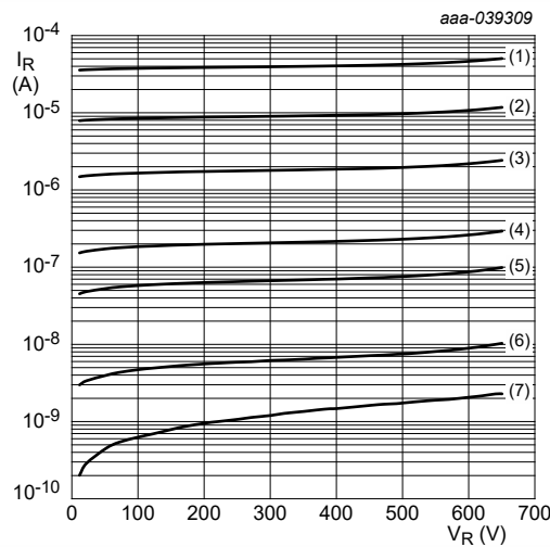
pulsed condition (1) T_j = 175^\circ\text{C} (2) T_j = 150^\circ\text{C} (3) T_j = 125^\circ\text{C} (4) T_j = 100^\circ\text{C} (5) T_j = 85^\circ\text{C} (6) T_j = 55^\circ\text{C} (7) T_j = 25^\circ\text{C}
