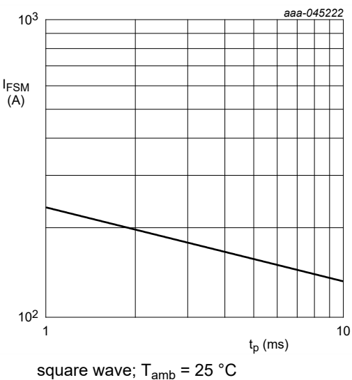
Fig. 5. Non-repetitive peak forward current as a function of pulse duration; typical values
