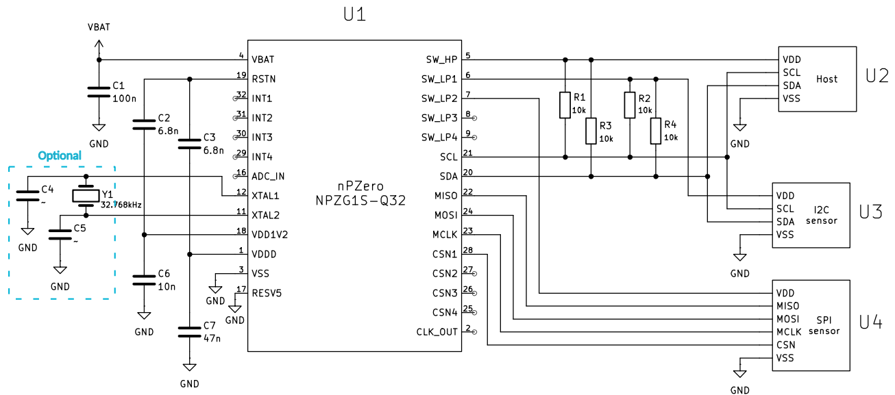
Figure 4: nPZero G1S typical application
