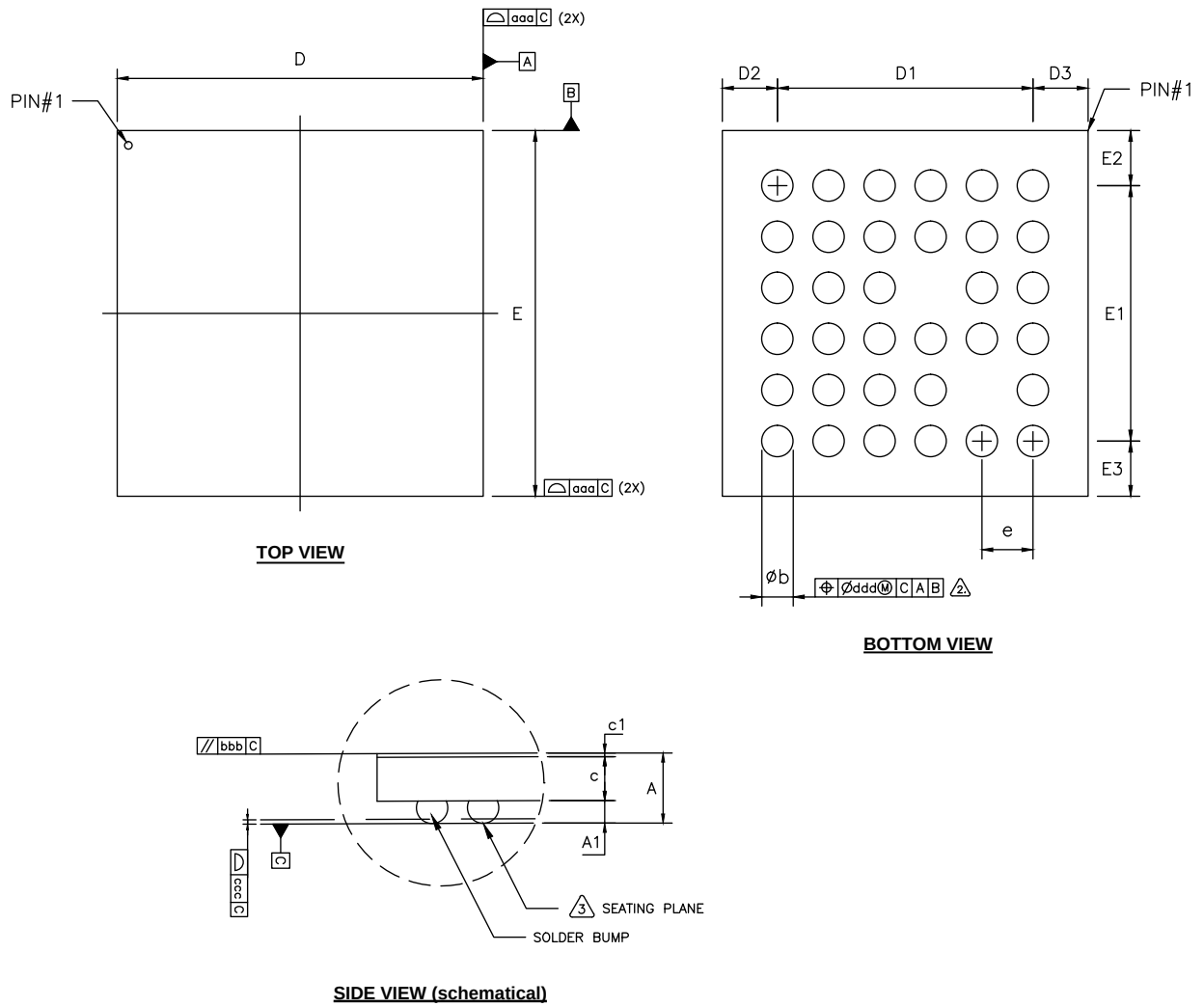
Figure 27: WLCSP34 packaging outline
