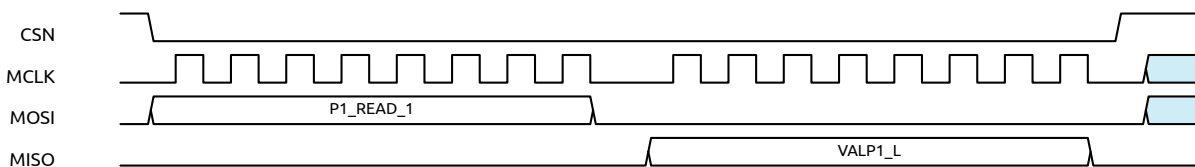
Figure 18: Typical SPI read of a peripheral using SPI mode 0. The illustration shows an example with one read command and 8-bit peripheral data.
