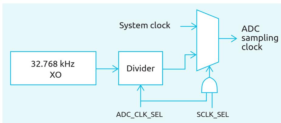
Figure 20: nPZero G1S ADC sampling clock routing diagram
