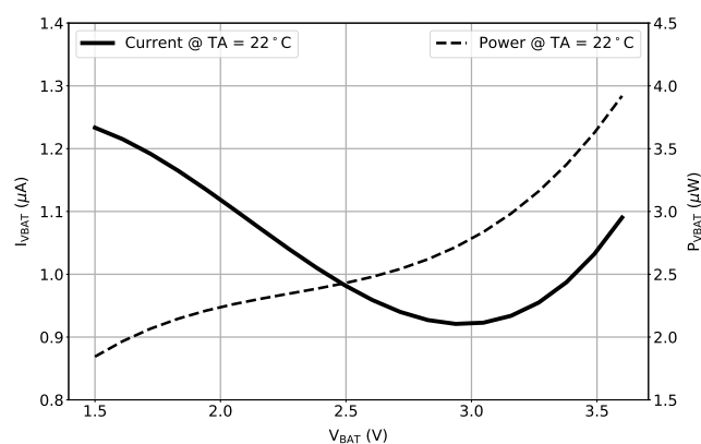
(b) VBAT current and power vs VBAT in Standby mode
