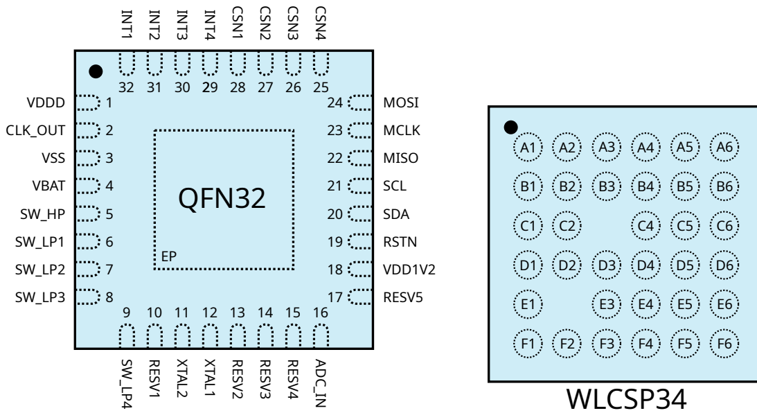
(a) QFN32 pinout, top view
