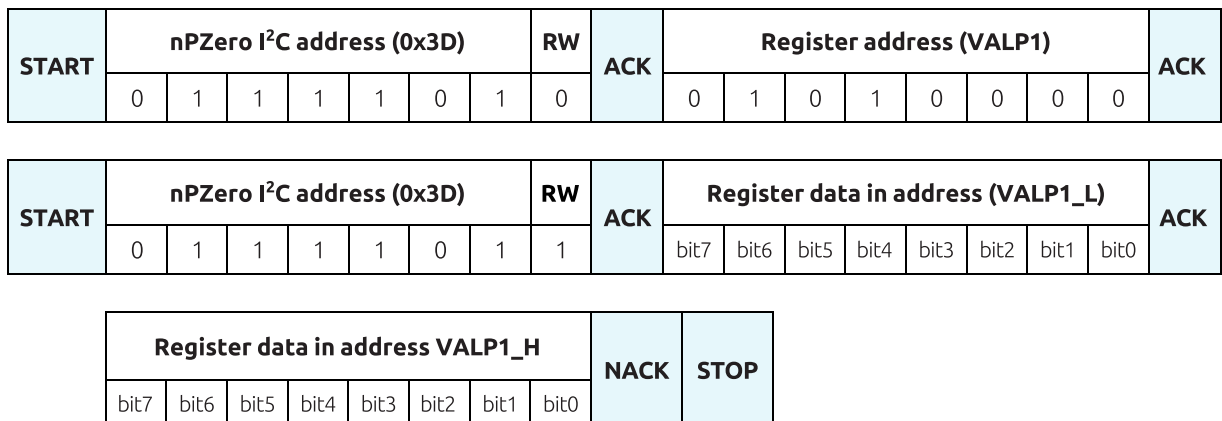
Figure 7: Example I 2 C multi-byte read operation on the nPZero G1S
