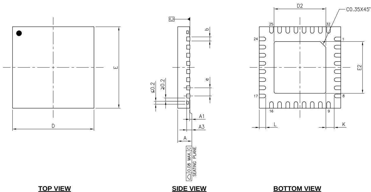
Figure 25: QFN32 packaging outline
