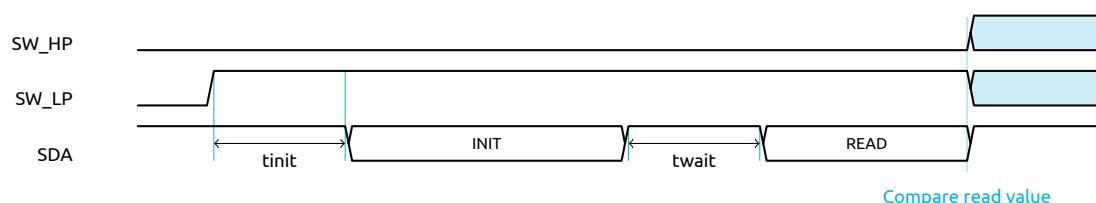
Figure 10: Timing diagram for Polling Mode 0
