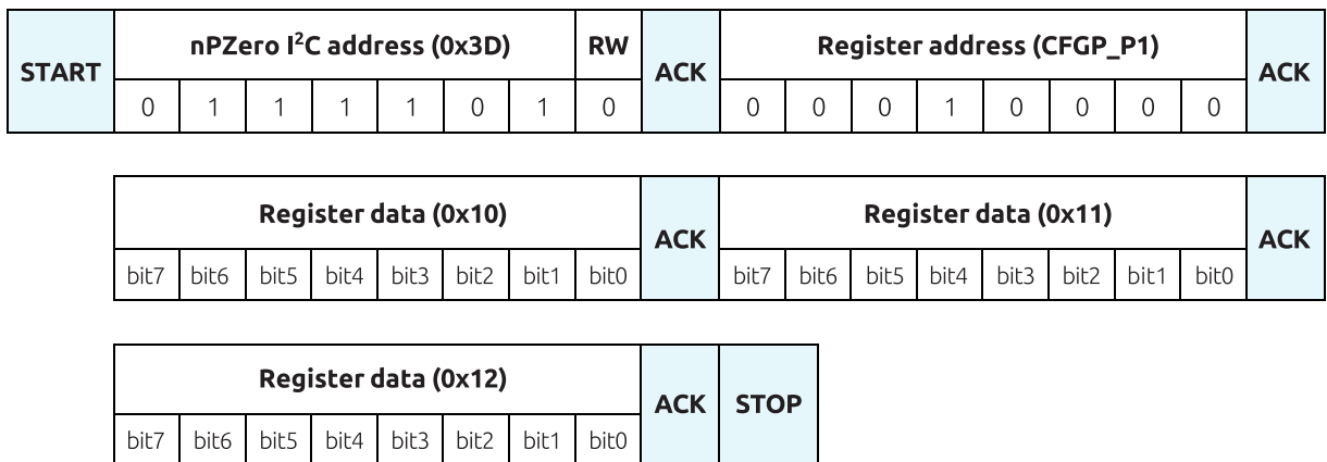
Figure 6: Example I 2 C multi-byte write operation on the nPZero G1S
