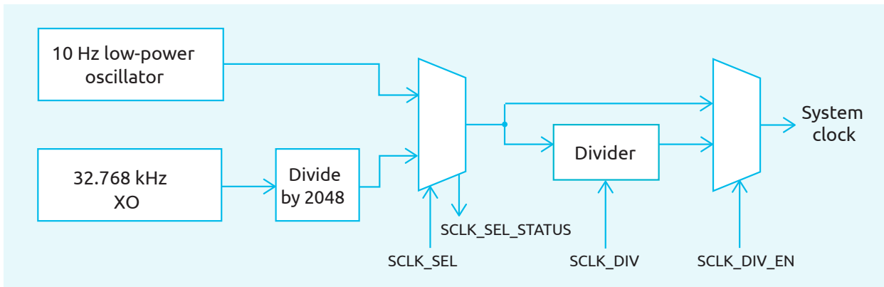
Figure 19: nPZero G1S system clock routing diagram
