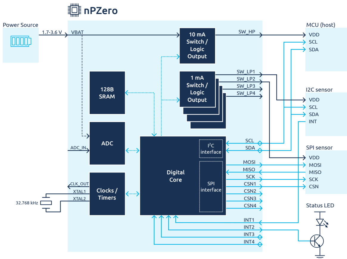
Figure 1: Illustration of the nPZero G1S in a system
