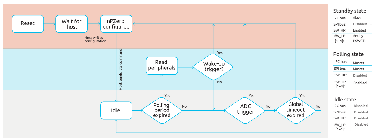
Figure 8: nPZero G1S decision flow chart and operation states
