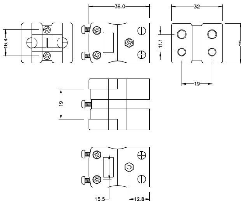
Standard Duplex in-line Socket (dimensions in mm)
